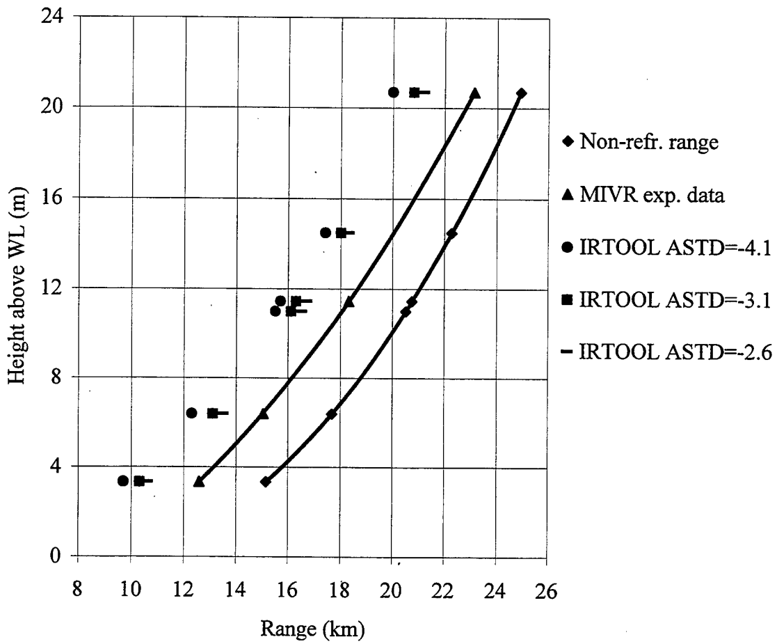
Figure 18. Comparison of the predictions of IRTOOL (MIVR) for ASTDs -4.1, -3.1 and -2.6°C with the ship-tracking data, measured by the visible camera
