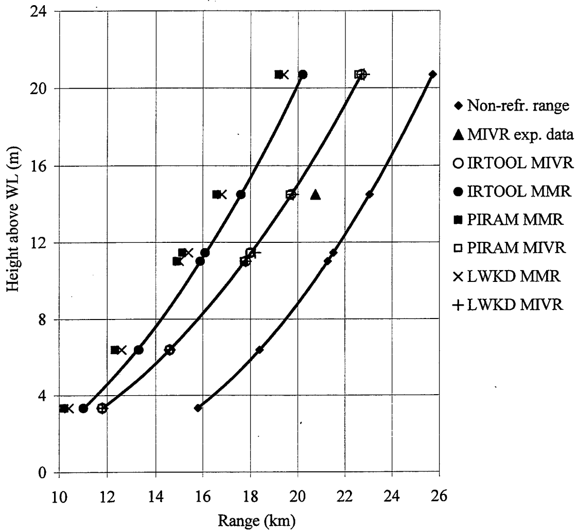
Figure 28. Comparison of the LWKD, PIRAM and IRTOOL model MIVRs and MMRs
