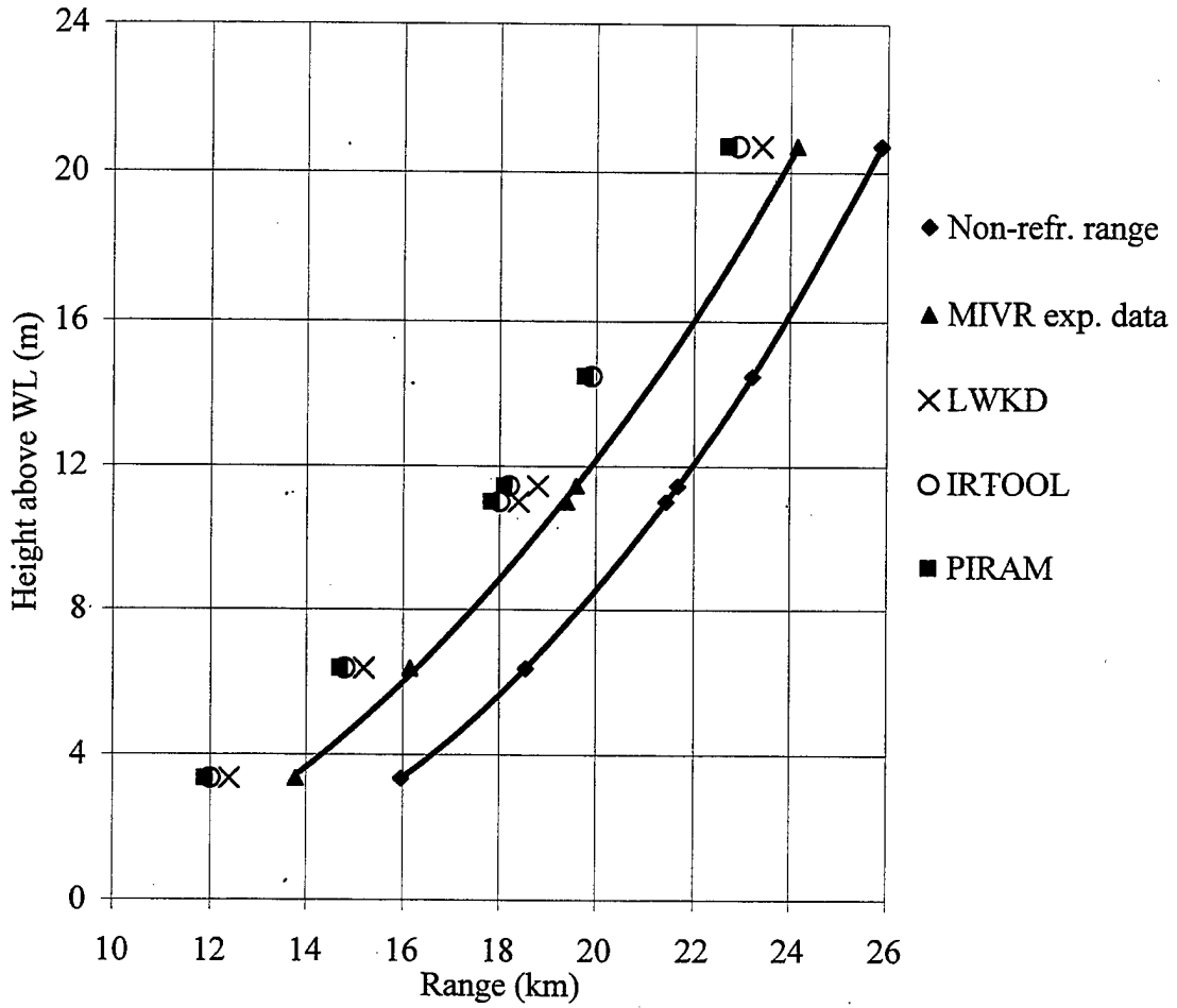
Figure 20. Comparison of the LWKD, PIRAM and IRTOOL model MIVRs with the ship-tracking data measured by the V1 visible camera
