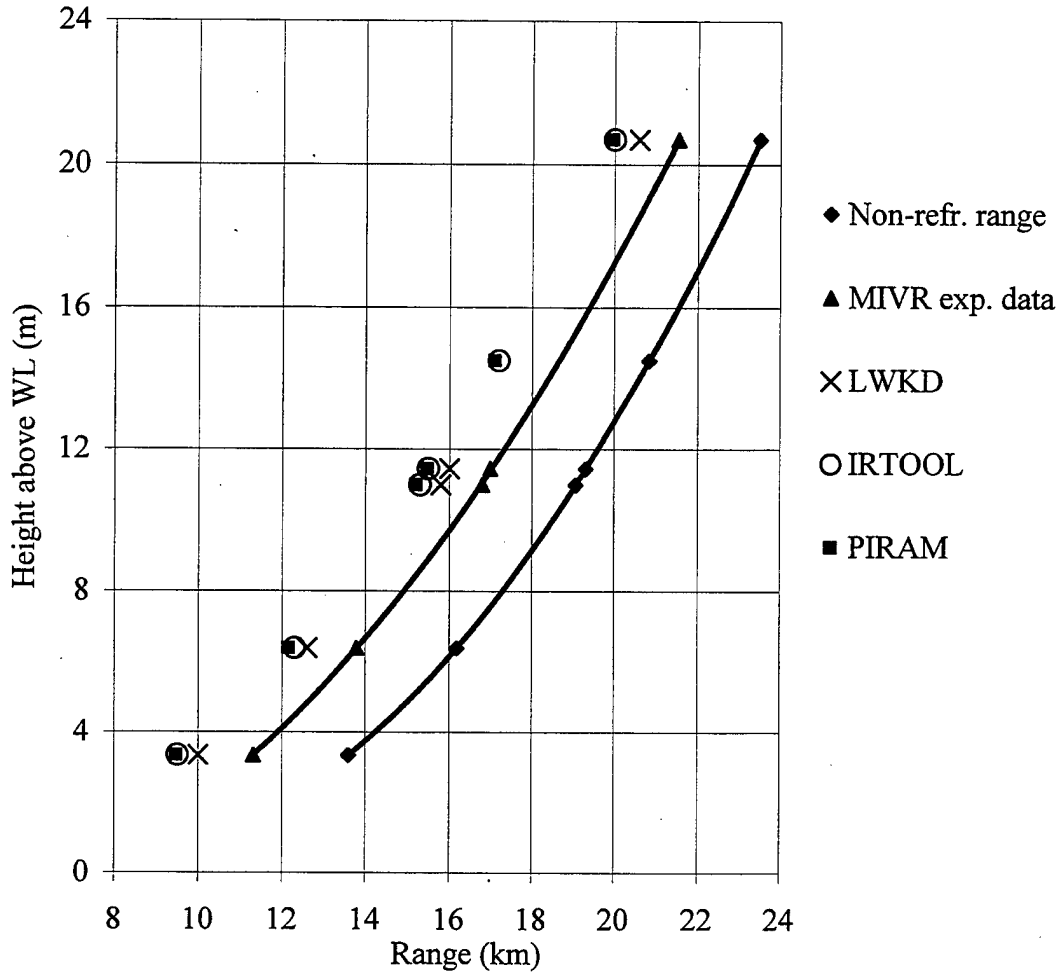
Figure 22. Comparison of the LWKD, PIRAM and IRTOOL model MIVRs with the ship-tracking data measured by the V2 visible camera
