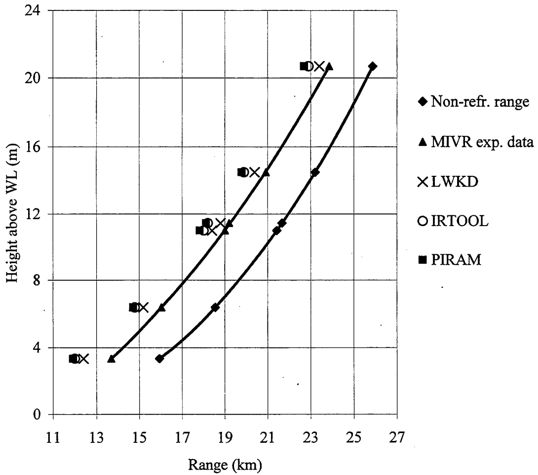
Figure 26. Comparison of the LWKD, PIRAM and IRTOOL model MIVRs with the ship-tracking data measured by the IR1 (3-5 \mu m) infrared camera
