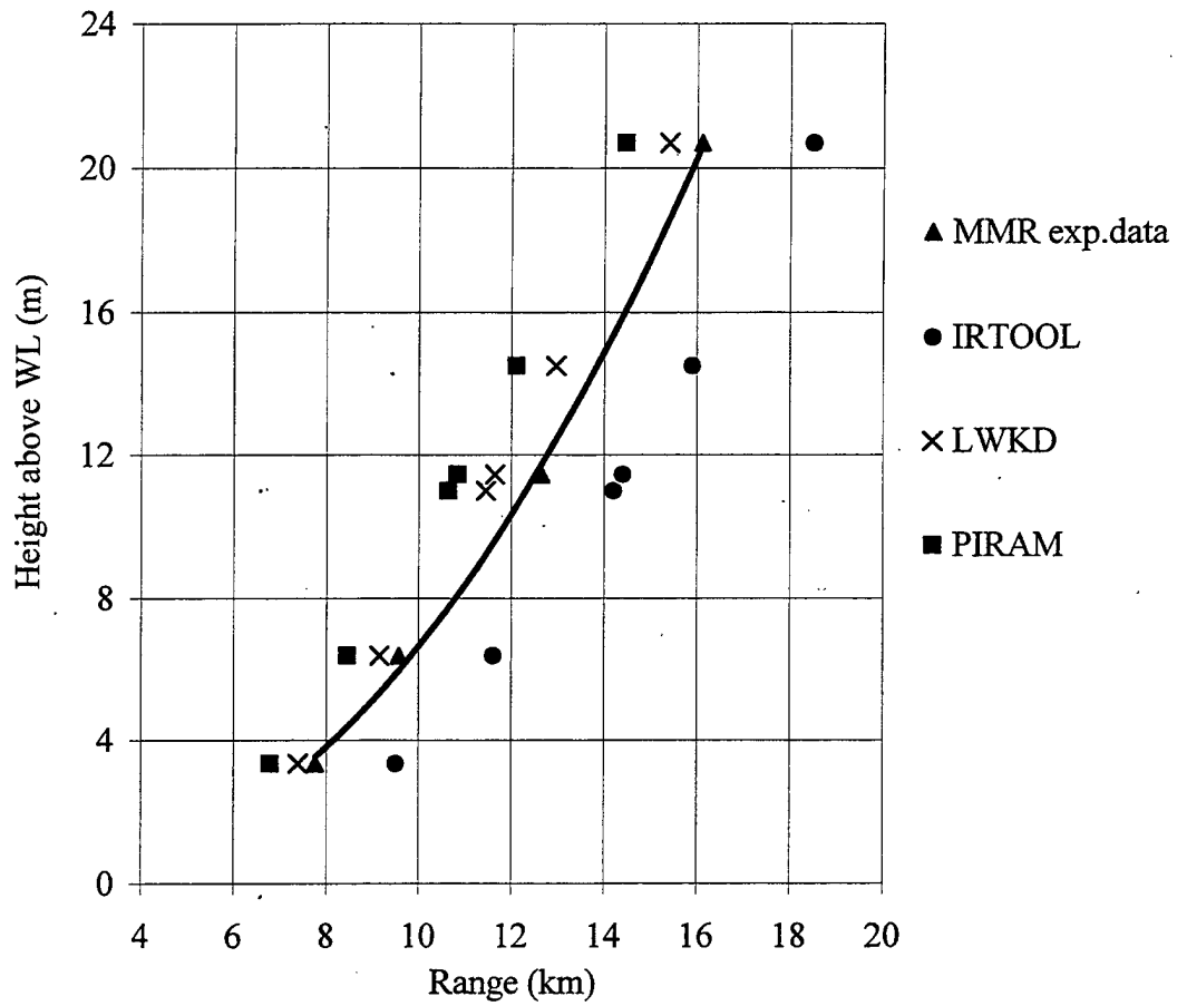
Figure 15. Comparison of the LWKD, PIRAM and IRTOOL model MMRs with the ship-tracking data, measured by the IR1 (3-5 \mu m) camera
