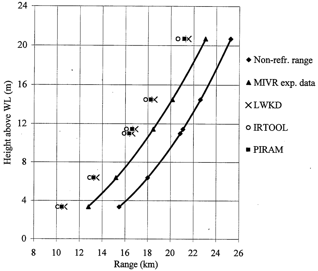
Figure 14. Comparison of the LWKD, PIRAM and IRTOOL model MIVRs with the ship-tracking data, measured by the IR1 (3-5 \mu m) camera
