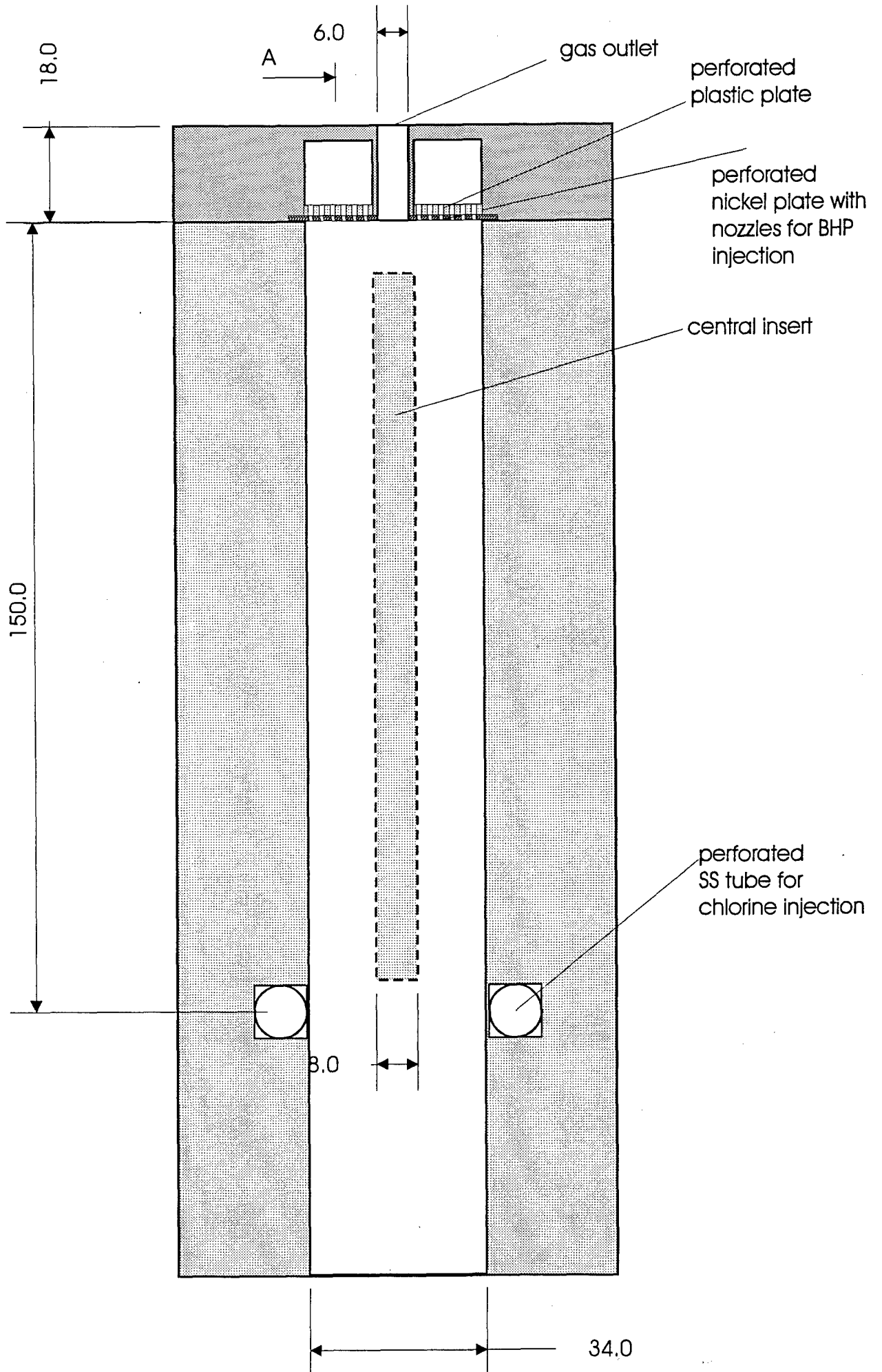
Fig 11. The sketch of verty Jet-SOG (central sectional view)
