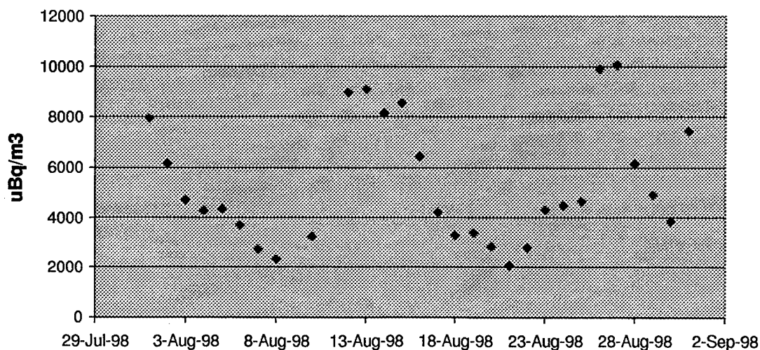
Figure 1: Pb-212 Concentration
