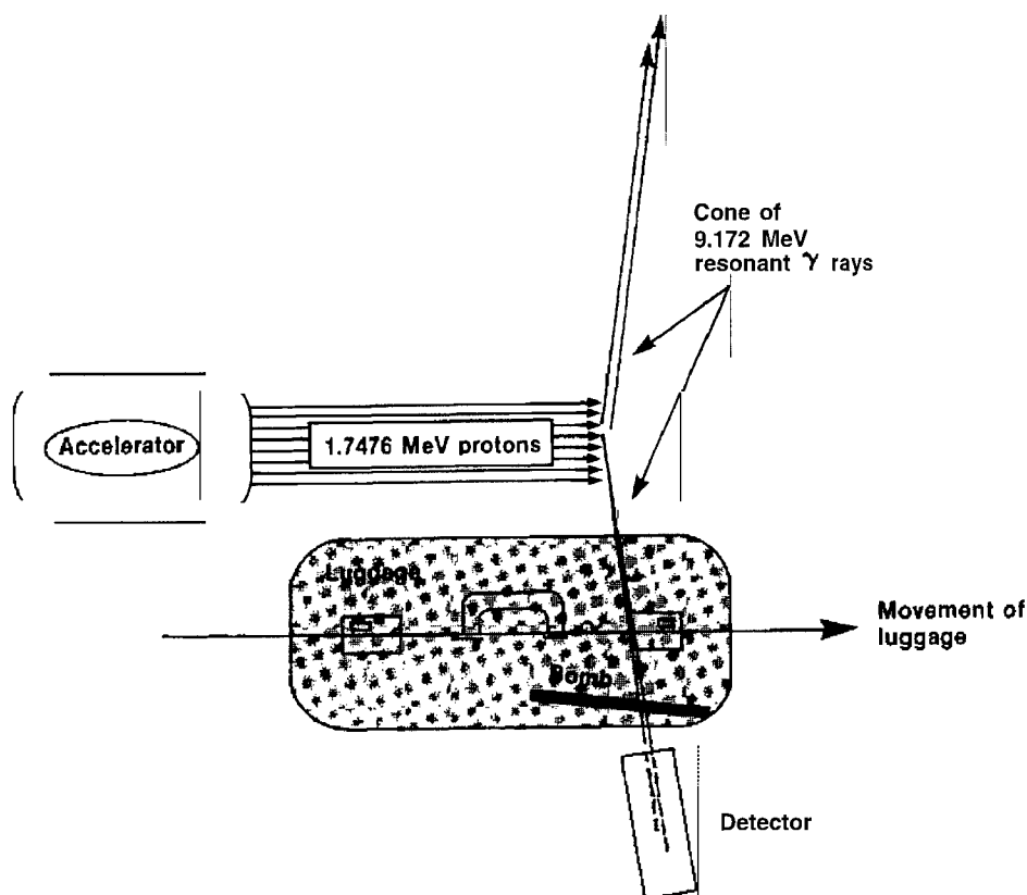
Figure A-5-Resonant Absorption of Gamma Rays
