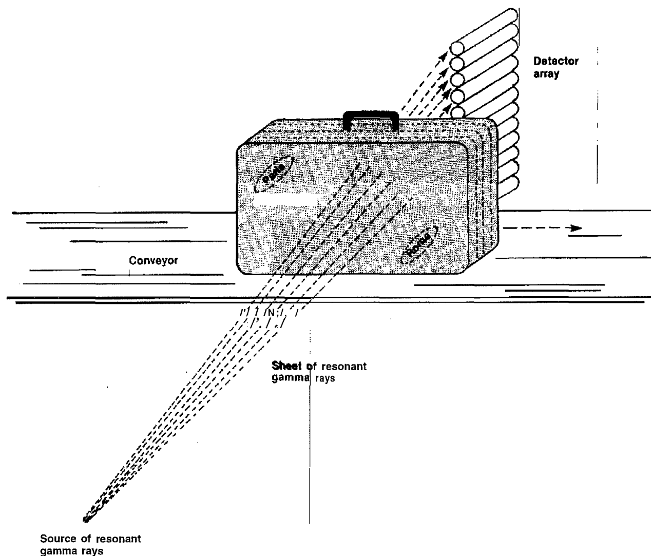
Figure A-4-Resonant Absorption of Gamma Rays
