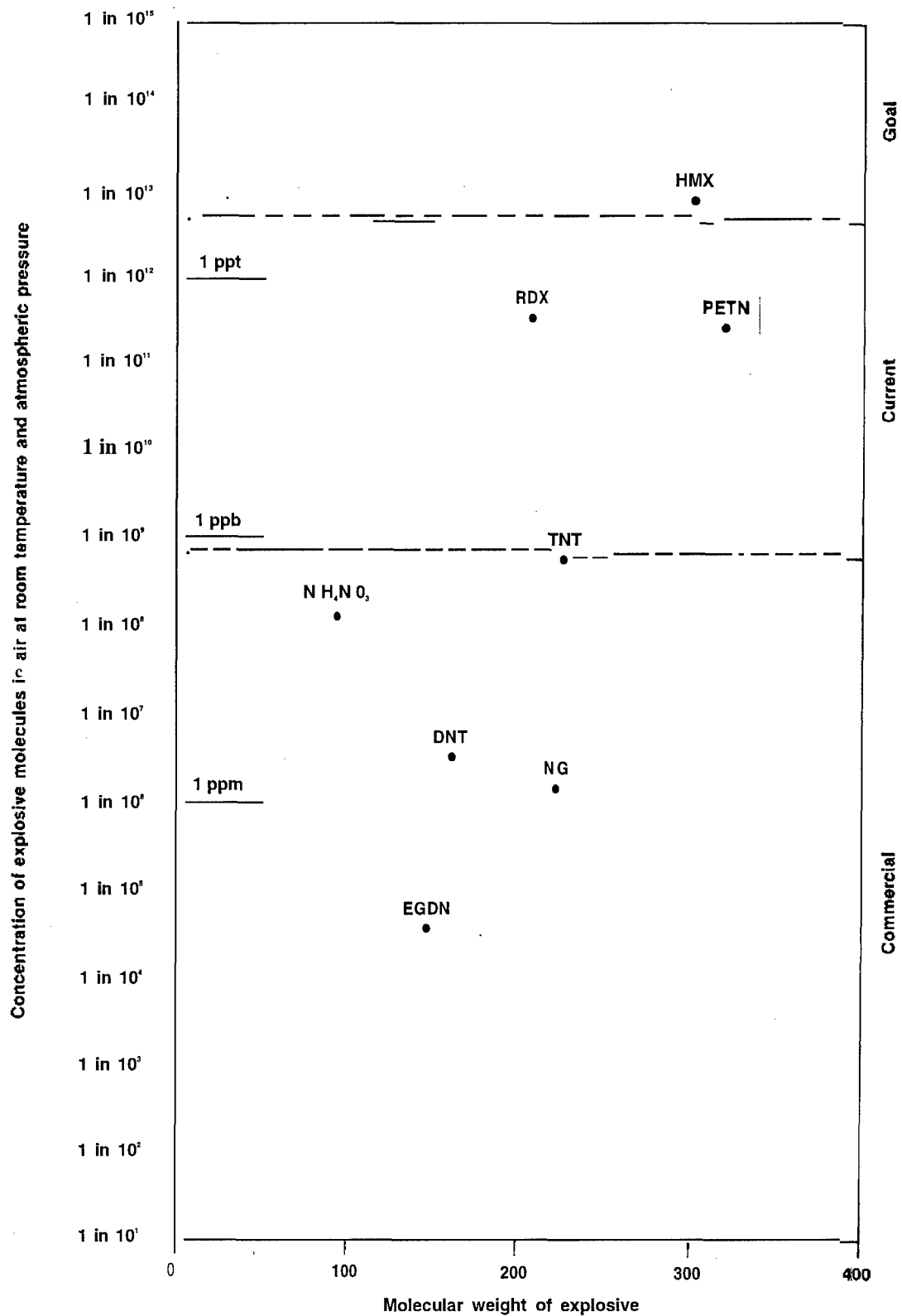
Figure 4-5-Relative Volatilities of Some Common Explosives
