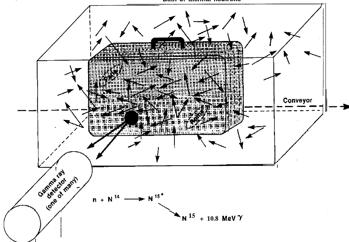
Figure A-1—Sketch of Apparatus for Thermal Neutron Analysis of Nitrogen Bath of thermal neutrons
