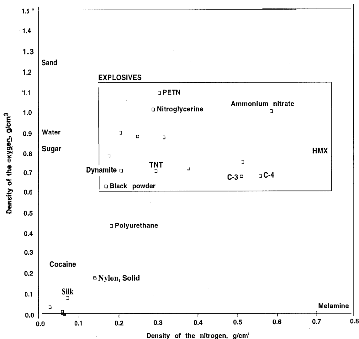
Figure 4-4-Correlation Between Oxygen and Nitrogen Densities in Explosives and Other Materials
