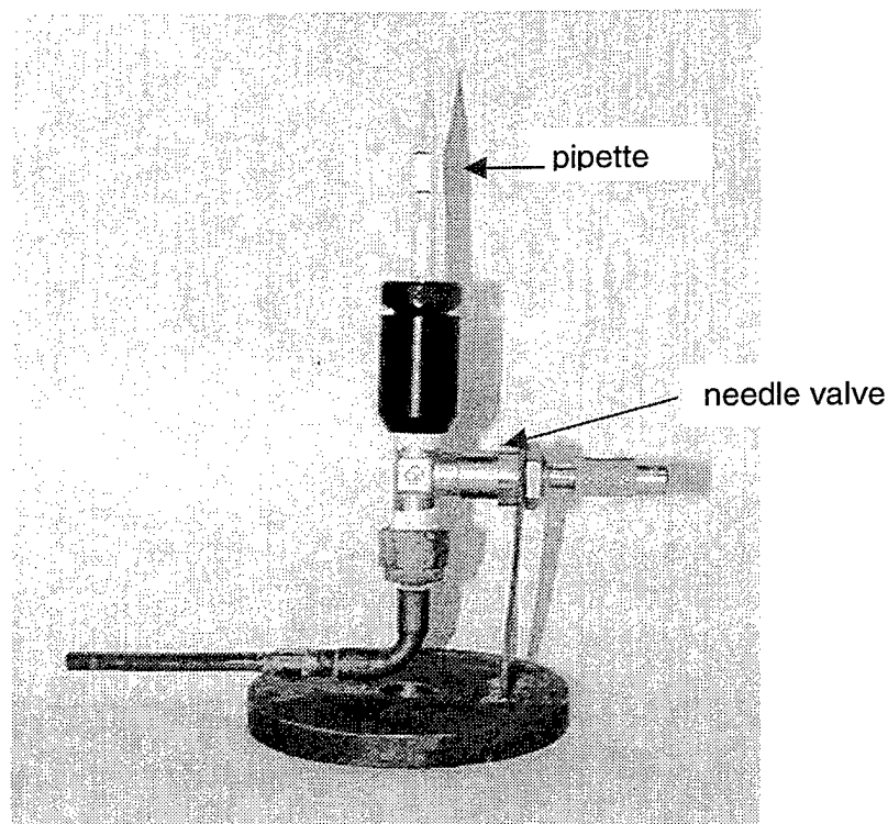
Figure 2.4 . Pipette and pipette holder. The needle valve was constructed into the holder with the hope of additional rate control. However, the needle valve quickly became corroded and was of little use. It was kept in the full open position throughout the experiment.
