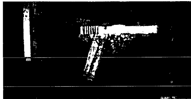
90-GHz radar image of Glock-17 pistol behind one layer of heavy wool and one of light polyester fabric.
