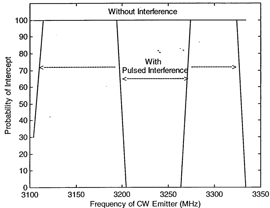
Fig. 17 — CW Emitter with pulsed emitter interference
