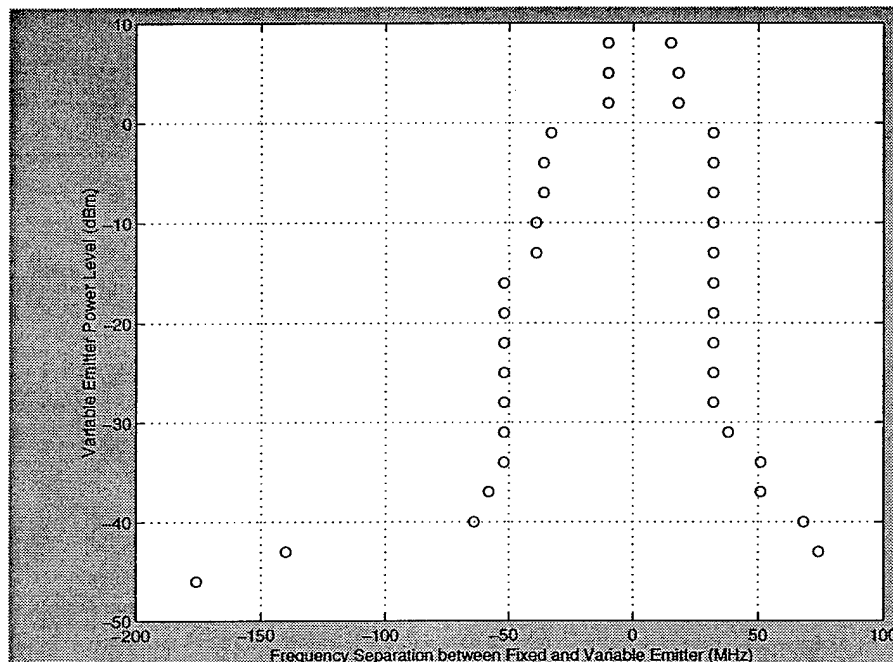
Fig. 14 — Two-Tone Frequency Resolution Test data
