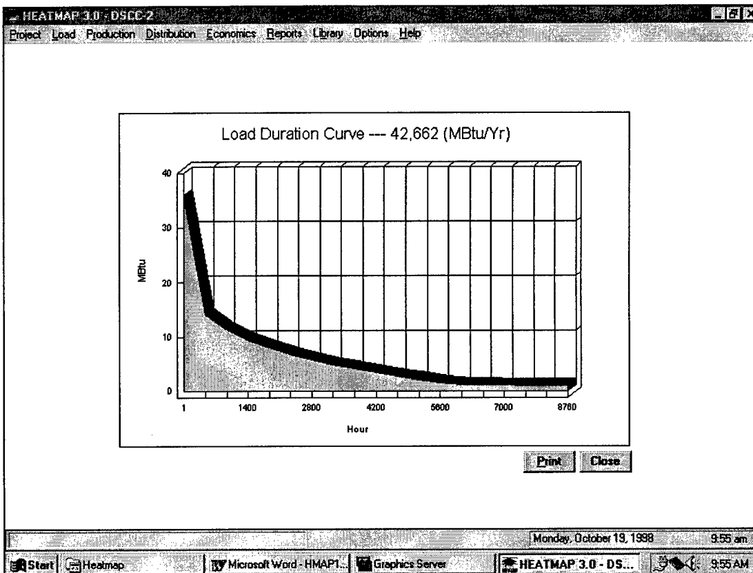
Figure 9. HEATMAP load duration curve output.
