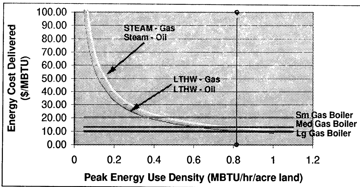
Figure 3. Energy cost versus peak energy density.
