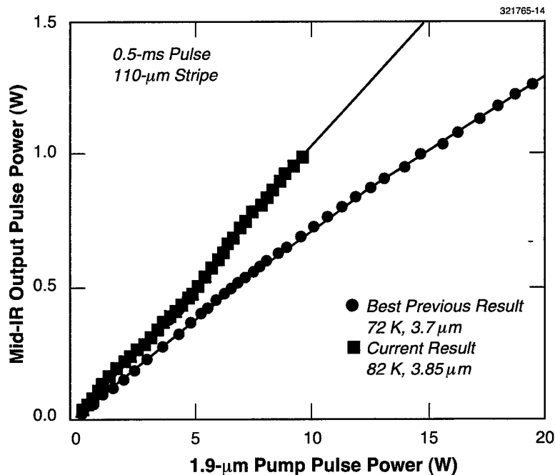
Figure 2-8. Mid-infrared pulse output power vs 1.9- \mu\text{m} input pump power for improved double heterostructure at 82 K and best previous result at 72 K.
