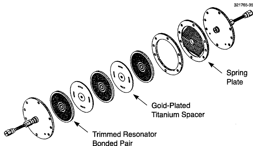
Figure 6-1. Exploded view of 3-pole filter.
