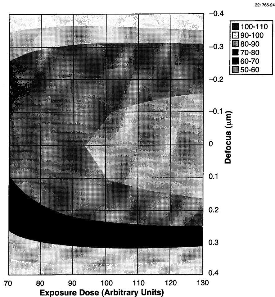
Figure 3-5. Calculated inverse image-log slope at all values of dose and focus for exposure conditions: \lambda = 193 \text{ nm} , NA = 0.5 , \sigma = 0.6 , and nominal 175-nm linewidth (isolated). Contours represent lines of equal inverse image-log slope in nm.
