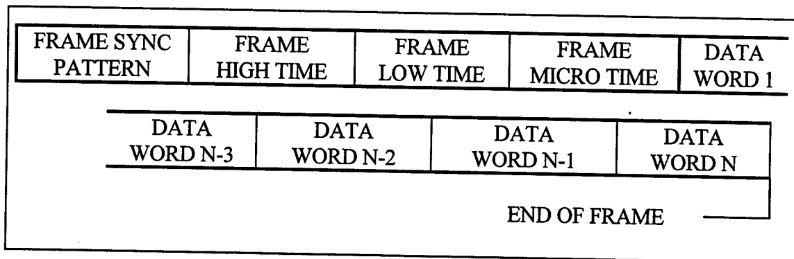
Figure 8-3. Composite frame structure.
