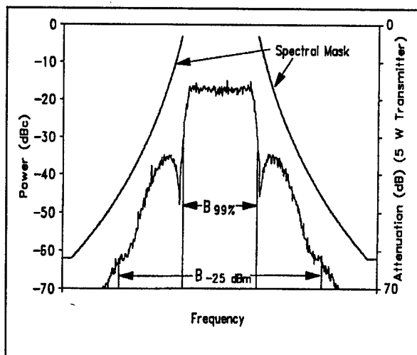
Figure A-7. 1000 kbps RNRZ PCM/FM signal and spectral mask (frequency span = 5 MHz).
