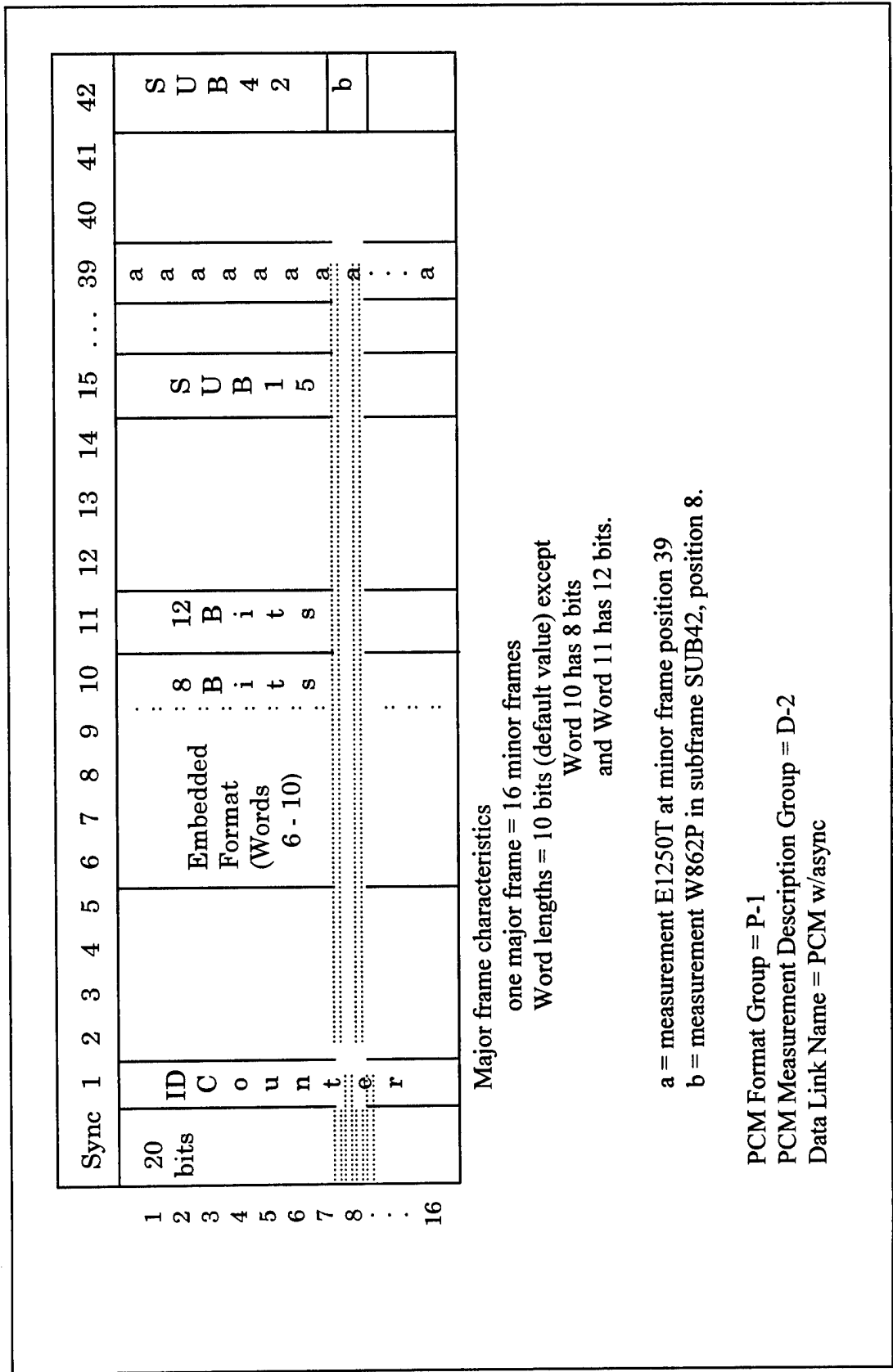
Figure J-2. PCM format for PCM w/async.
