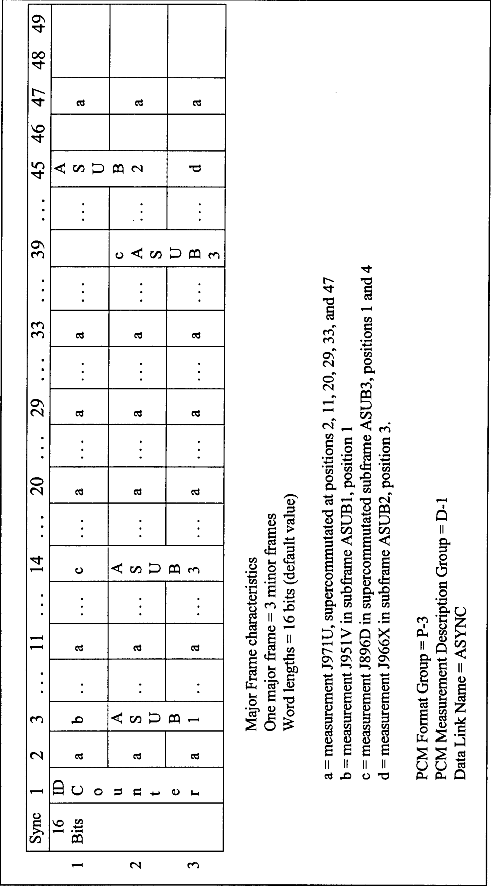
Figure J-4. PCM format for async.
