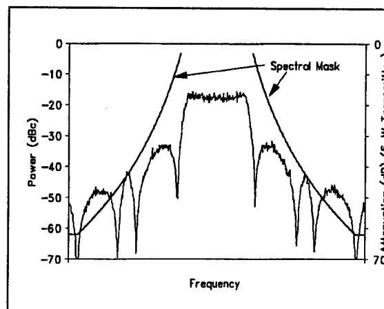
Figure A-8. Unfiltered 1000 kbps RNRZ PCM/FM signal and spectral mask.
