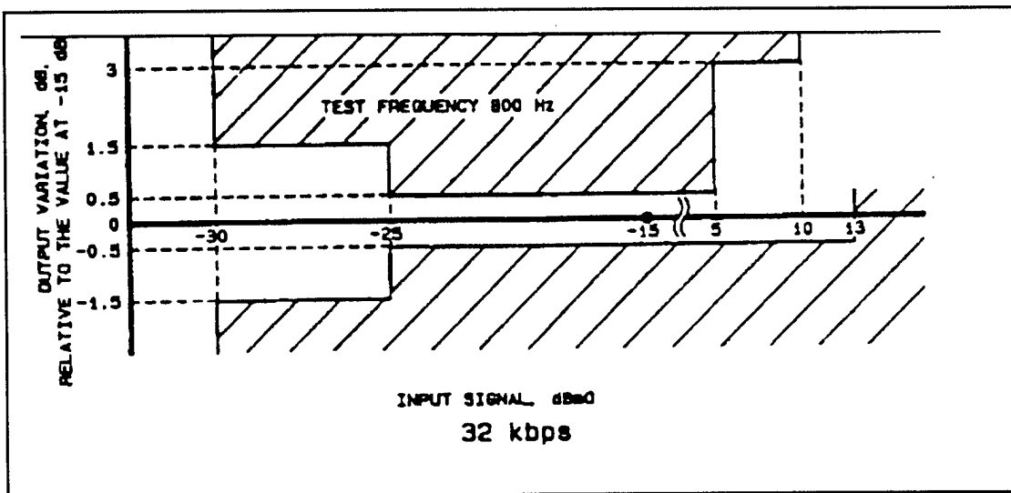
Figure F-5b. Variation of gain with input level for CVSD (32 kbps).
