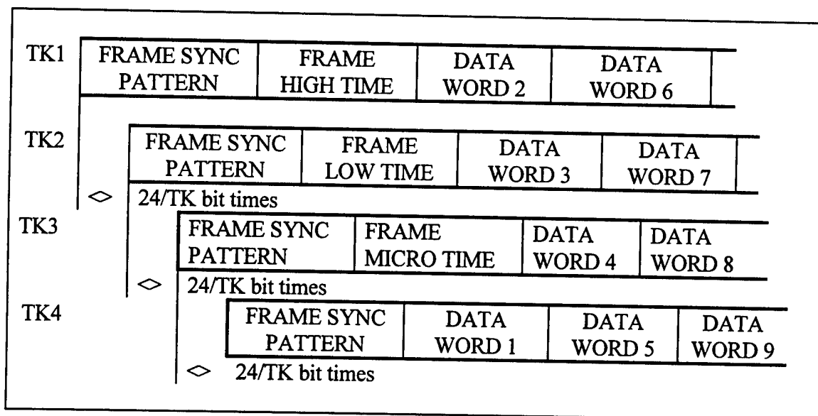
Figure 8-4. Multiple tape track spread format (4-track spread example).
