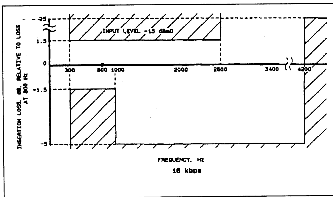
Figure F-4a. Insertion loss versus frequency for CVSD (16 kpbs).
