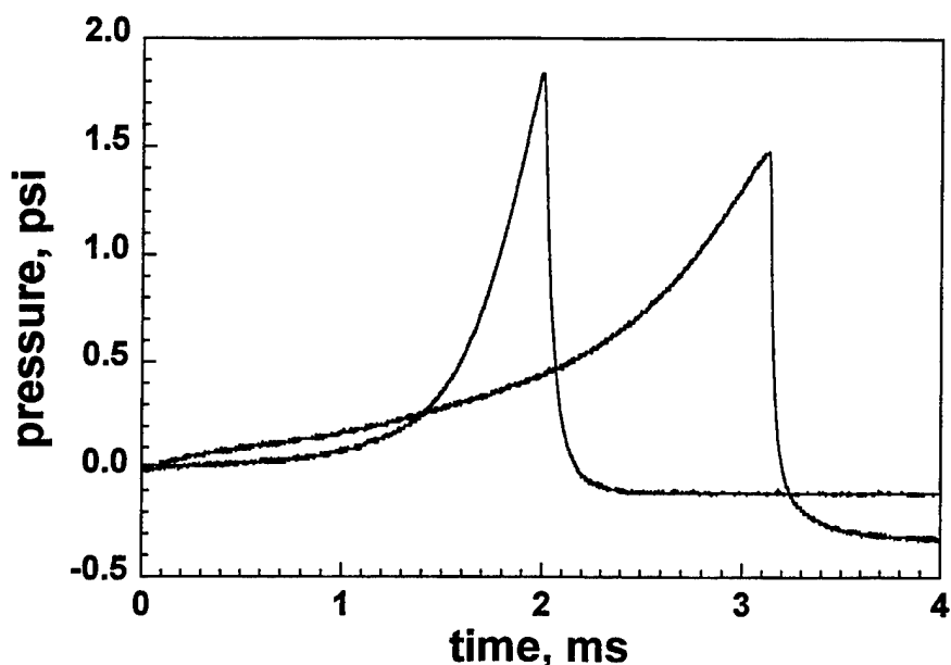
Figure 2. Typical Pressure-Time Records for 44 (Right Peak) and 90 mg of BP.
