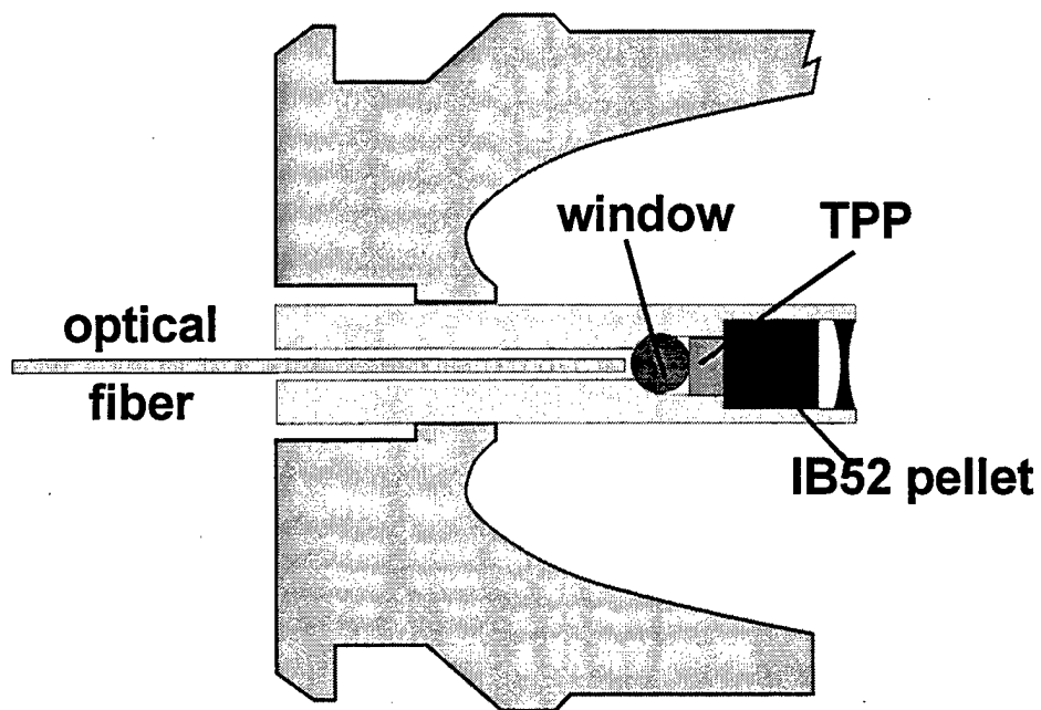
Figure 10. Short Flashtube Configuration.
