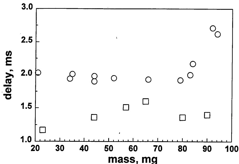
Figure 4. Ignition Delay vs. Loading Density for Class 7 (○) and FFFg (□) BP, Laser Unfocused.
