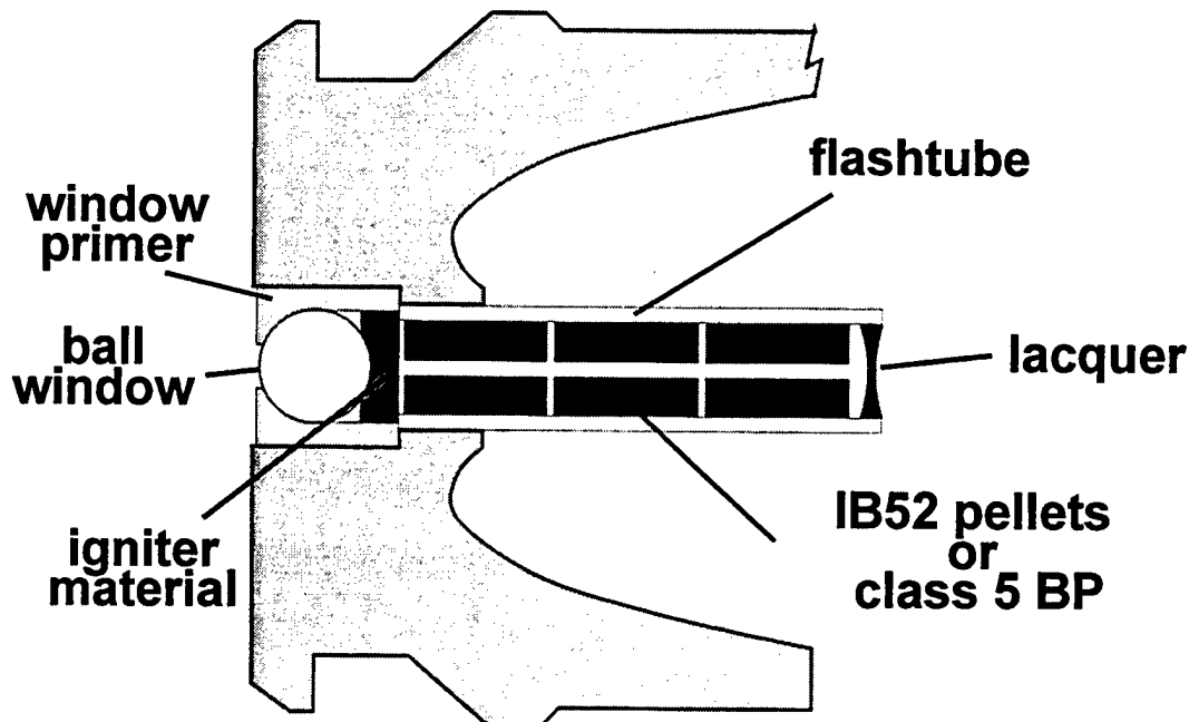
Figure 12. Ball Window Configuration for Third Gun Test Series.
