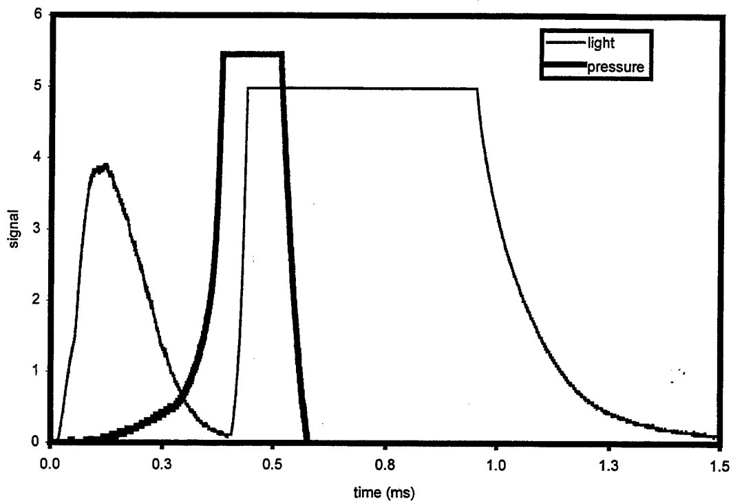
Figure 7. Pressure-Time Record and Photodiode Signals.
