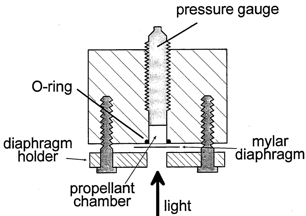
Figure 1. Schematic of Chamber for Laboratory Tests.
