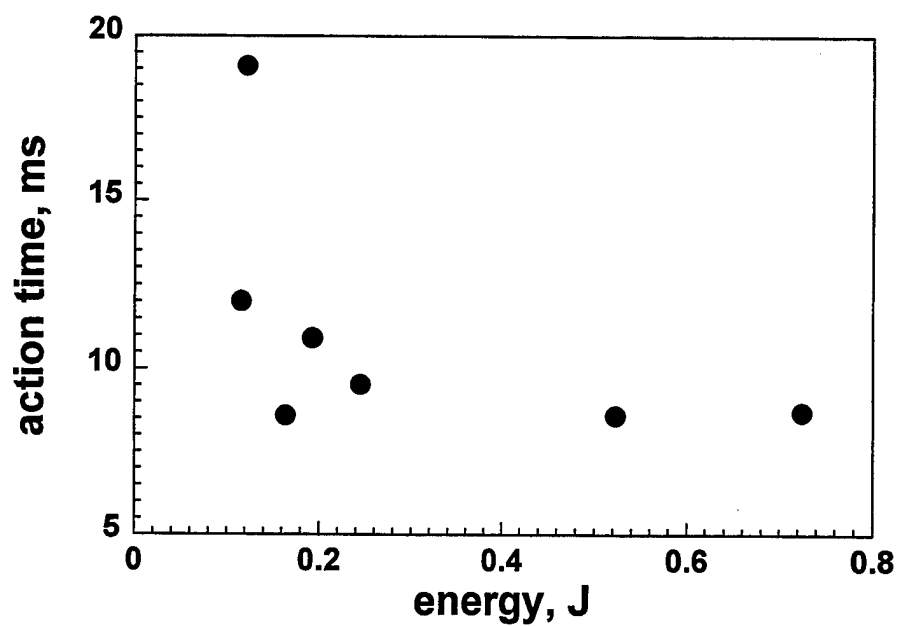
Figure 11. Gun Action Time With Reduced Laser Energy.
