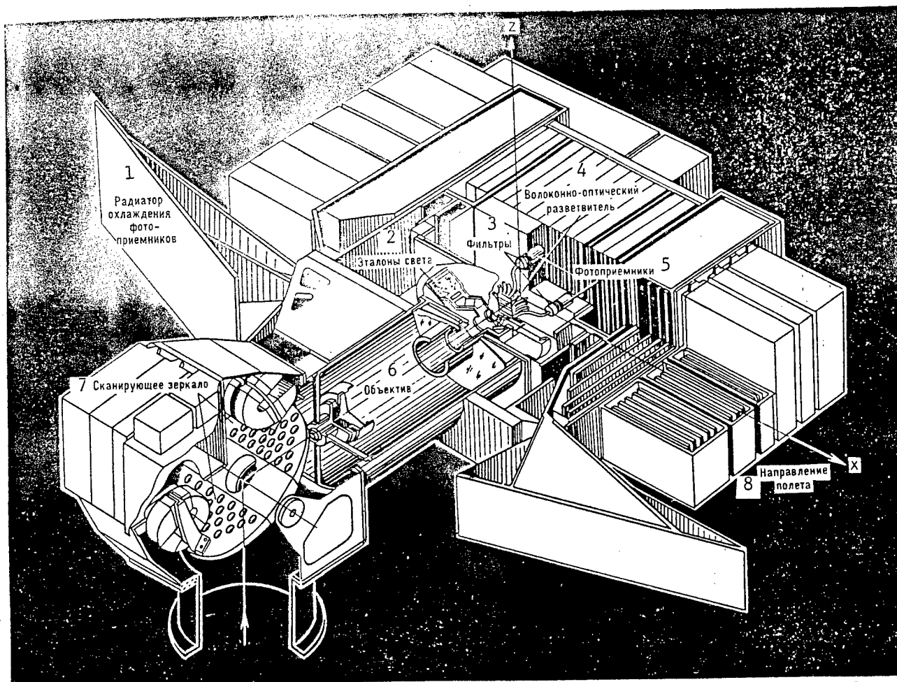
Cutaway diagram of "Fragment" imaging system. Key: 1) photodetector cooling radiator; 2) light standards; 3) filters; 4) fiberoptic splitter; 5) photodetectors; 6) objective; 7) scanning mirror; 8) direction of flight.
