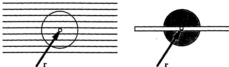
Figure 2.2 (a) The integral term in equation (2.2) is evaluated in a spherical region of radius R . (b) The region R is divided into two parts.
