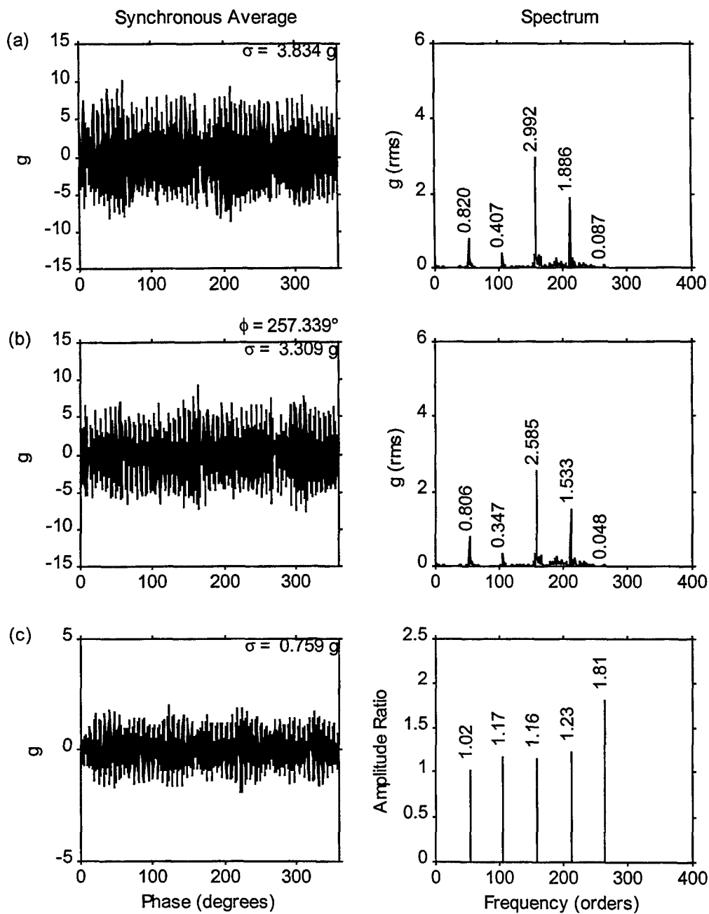
Figure 46. Synchronous Averages for Hover a) using the photocell signal, b) using the AC generator signal ( \phi = phase offset of (b) to (a)), c) difference between (a) and phase shifted (b), and amplitude ratios of gear mesh harmonics.
