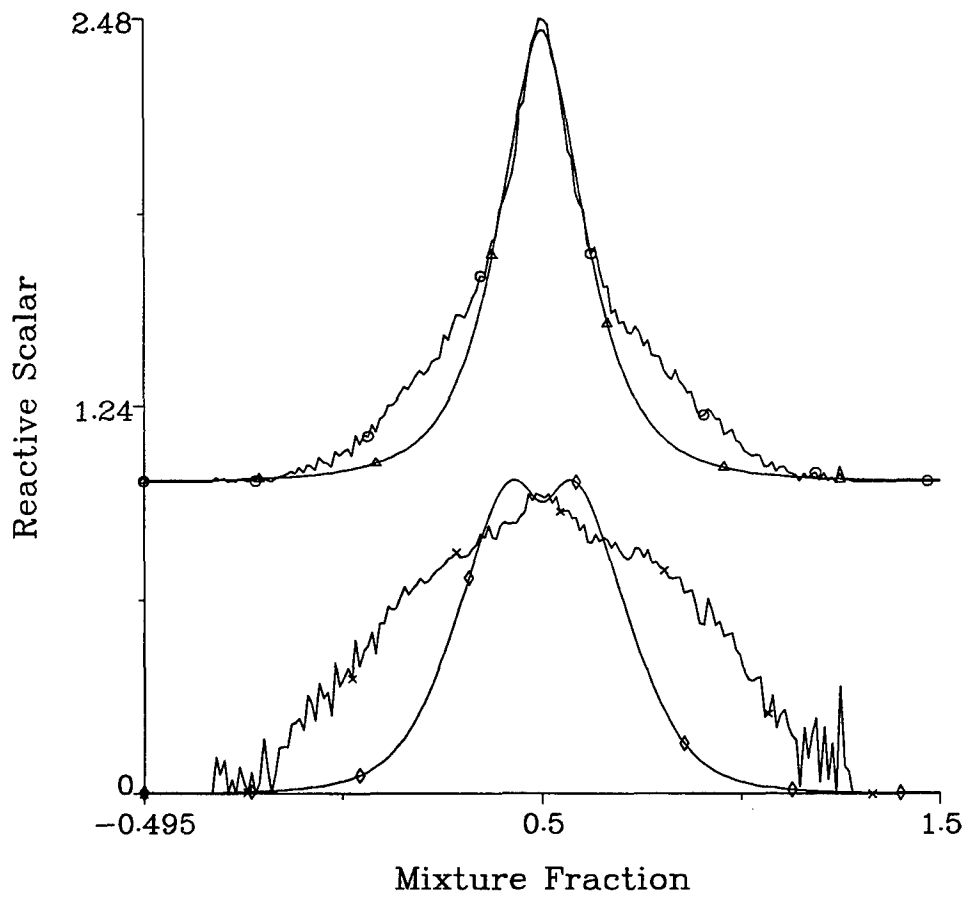
Figure 6: Modelled and observed conditional mean and variance of particle mass fraction for case s2i. Symbols denote the following profiles: \Delta - Q_\eta prediction, \circ - simulated Q_\eta , \diamond - q_\eta prediction, and \times - simulated q_\eta .
