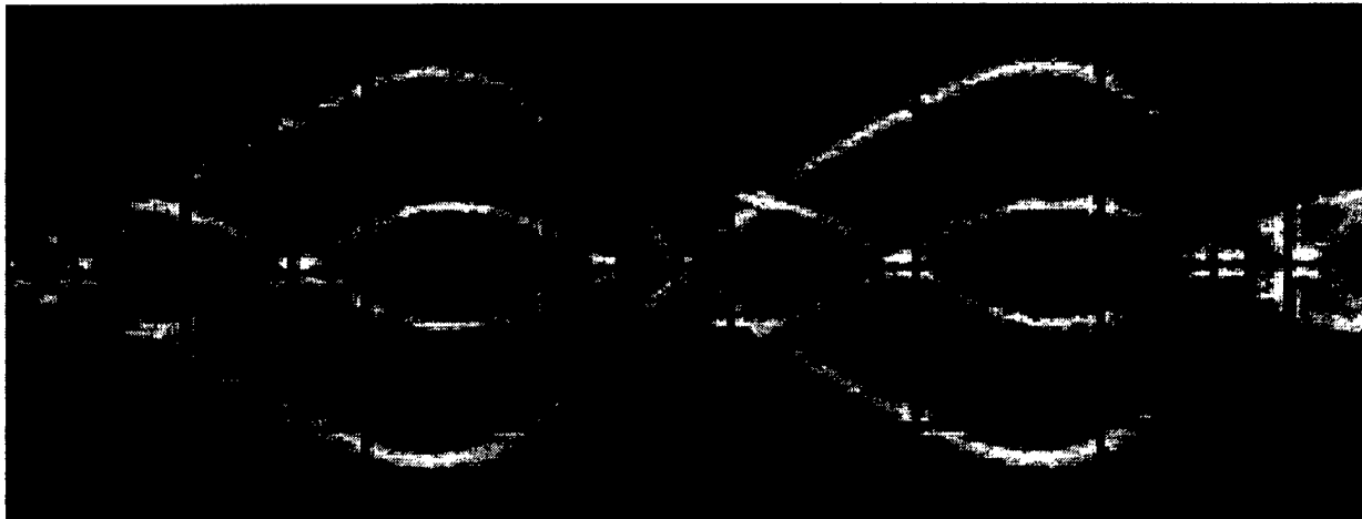
Figure 1-16. Poor bi-phase eye pattern.
