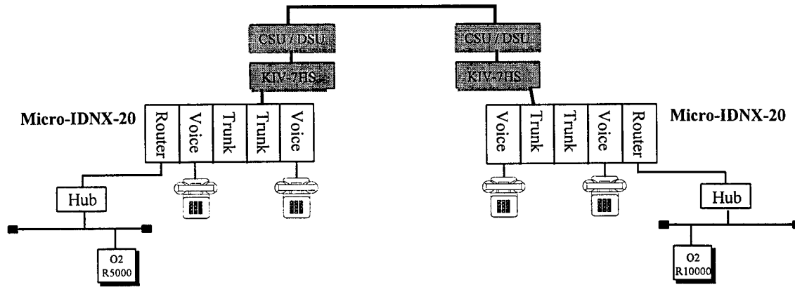
Figure 4. Two-Node RTI Test Configuration with Communications Devices
