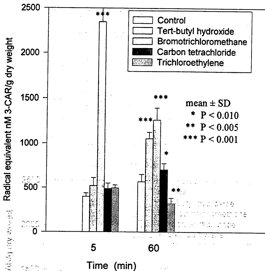
Figure 5. Radicals quantitated at 5 and 60 minutes in control liver slices and liver slices exposed to 1 mM TBOOH, \text{BrCCl}_3 , \text{CCl}_4 , or TCE
