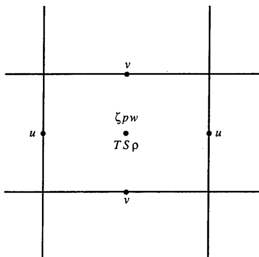
Fig. 1 — Horizontal arrangement of primary model variables on the numerical grid for all the models
