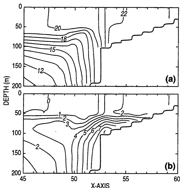
Fig. 35 — An expanded view of the temperature field in the downwelling area at 40 d from the 10-km simulation with POM. The temperature values are shown in (a) and the anomaly from the initial temperature profile is shown in (b).
