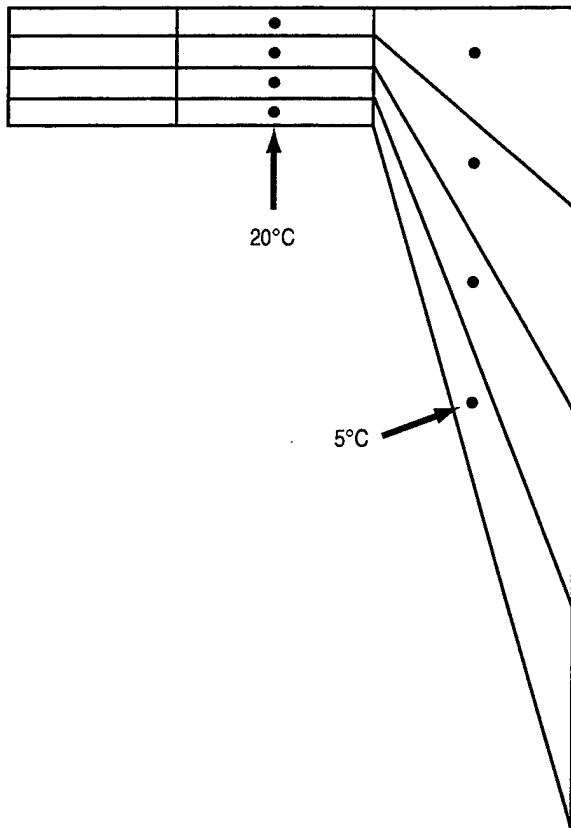
Fig. 8 — Schematic illustrating the large change in temperature that can occur between adjoining grid cells in the bottom layers of a sigma coordinate model if there is a large change in depth between the cells such that the cells lie on different sides of a strong thermocline
