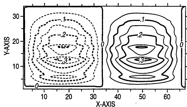
Fig. 30 — Analytically calculated cross-channel velocity field for a barotropic shelf wave propagating along step-wise bathymetry. The step-wise bathymetry is the same as that used by the SZM shelf-wave simulation with a z-level grid with \Delta z = 10 m.
