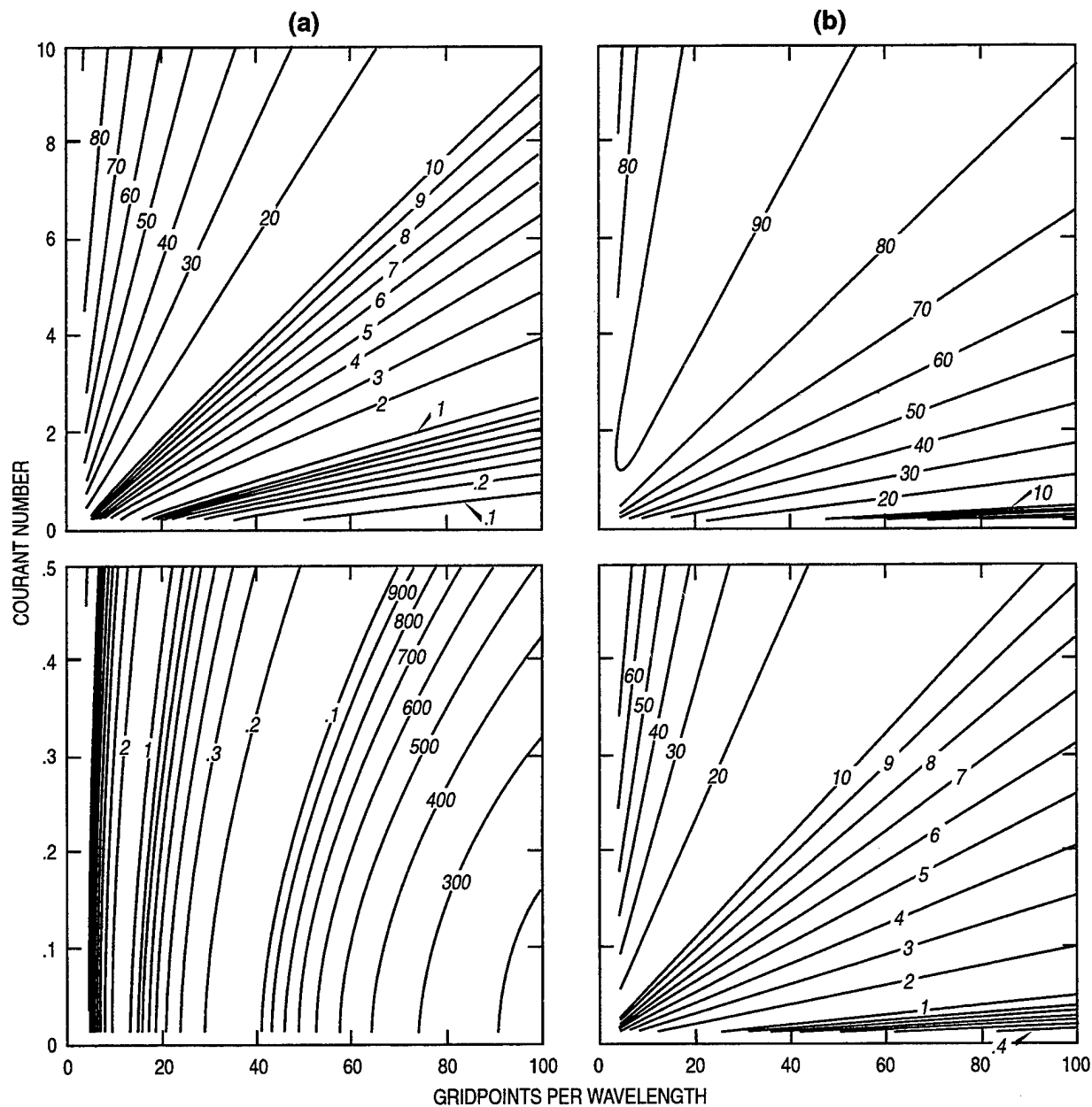
Fig. 38 — Same as Fig. 37, but for ECOM-si
