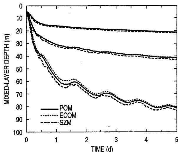
Fig. 9 — Surface mixed-layer depth vs. time for the models for a constant wind stress that is turned on at t = 0 . Three cases are shown for wind stress values of 1, 4, and 16 dynes/cm 2 . The initial condition was zero velocity, a constant salinity of 35 psu, and a linear temperature stratification of 5°C/100 m, with an SST of 24°C. The latitude is 29.91° N.
