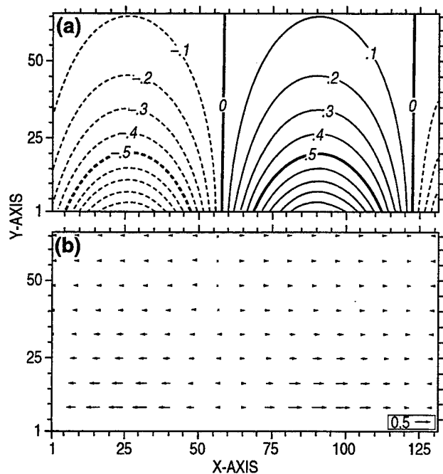
Fig. 23 — Analytical solution for a surface Kelvin wave at 48 h: (a) surface elevation in centimeters and (b) horizontal velocity vectors. The scaling arrow in the velocity vector plot indicates a speed of 0.5 cm/s.
