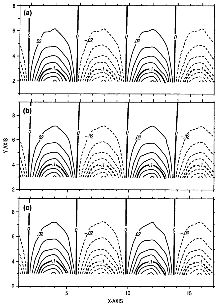
Fig. 26 — Comparison of horizontal section of salinity anomaly S' from models at 48 h for propagation of internal Kelvin wave for case with 4-km grid spacing and 800-s timestep: (a) POM, (b) ECOM-si, and (c) SZM. The horizontal section is at the center of the eighth model layer at a depth of 18.75 m. Contour interval is 0.02 psu.
