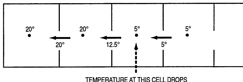
Fig. 7— Schematic showing advection between grid cells at the location of a sharp front. The temperature flux at the interface between the grid cells is calculated based on the mean temperature of the adjoining cells. The temperature at the cold grid cell on the upwind side of the front drops because the advective flux leaving the cell is much warmer than the advective flux entering the cell.
