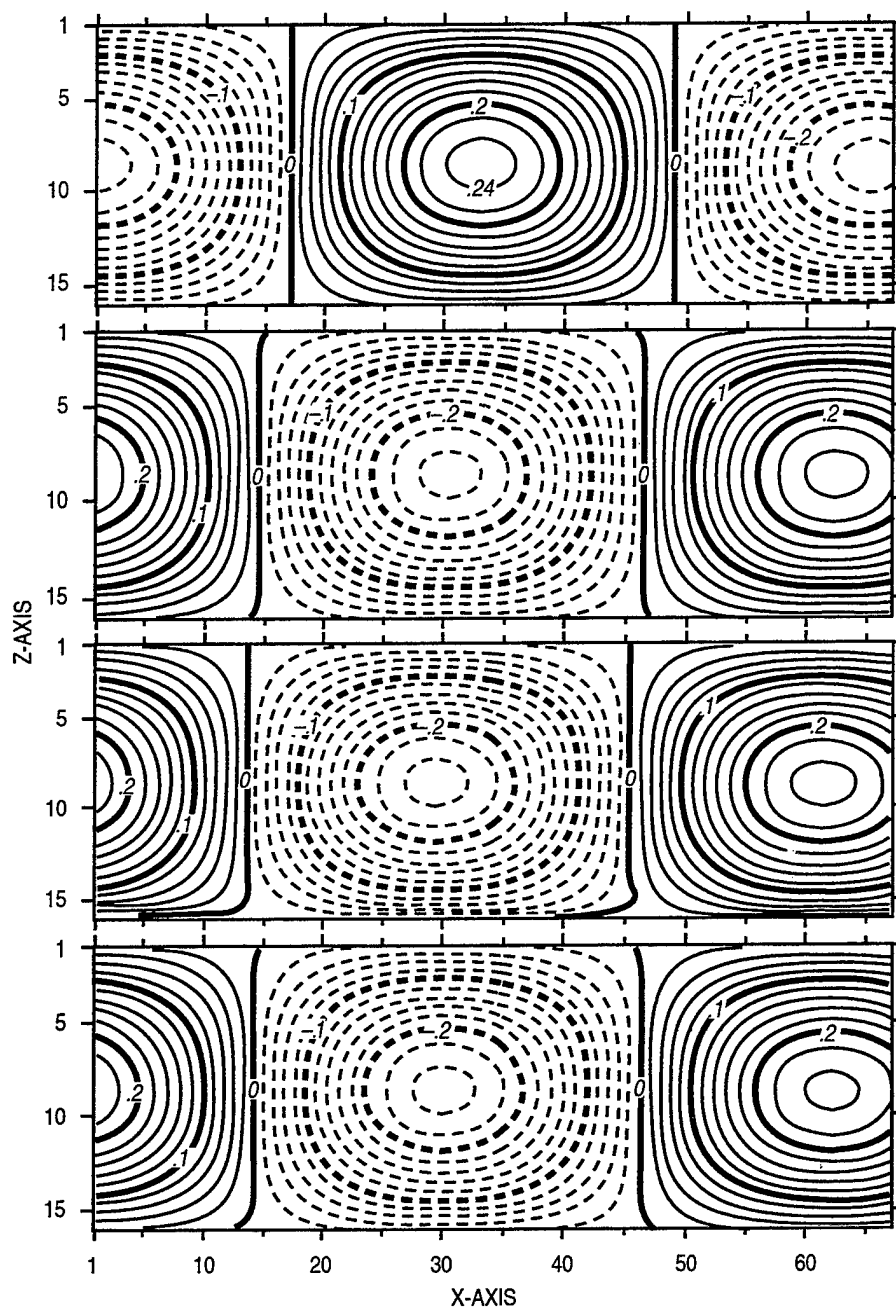
Fig. 20 — Salinity anomaly S' for propagation of internal waves of 64-km wavelength. The uppermost plot shows the initial condition, and the other plots show results after 48 h for POM, ECOM-si, and SZM. The internal wave amplitude was 100 cm and the timestep was 200 s.
