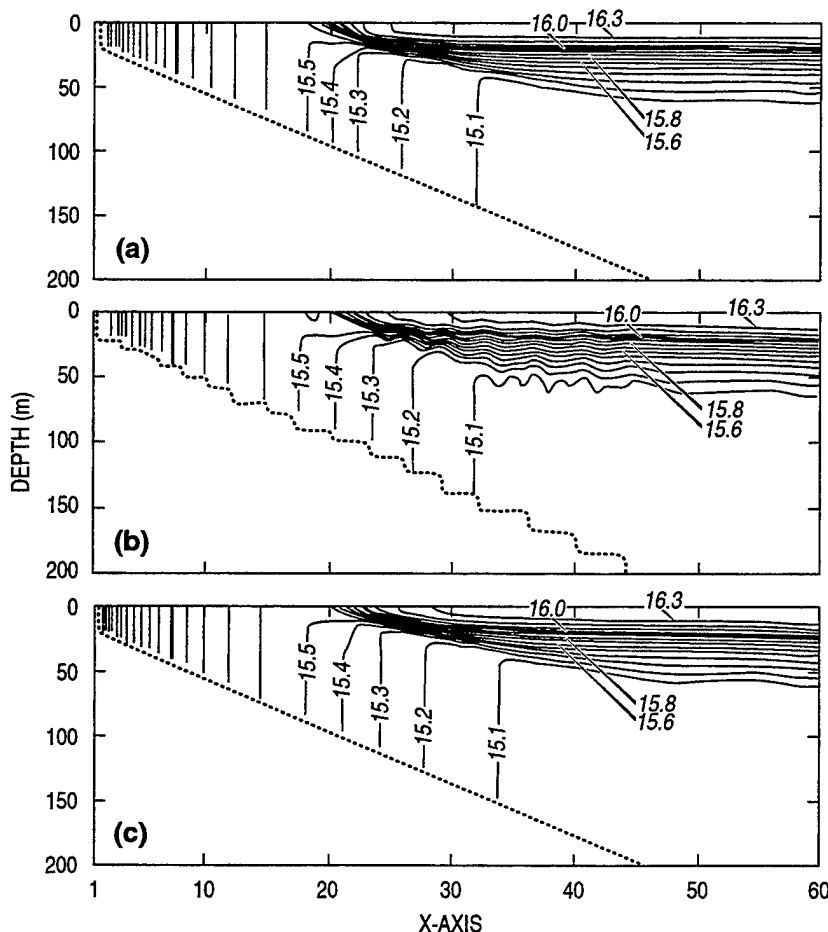
Fig. 14 — Temperature x - z sections at 30 d for the formation of a tidal mixing front using SZM with different vertical grids: (a) 20 sigma layers as in Fig. 13, (b) 20 layers with z -levels, except for two sigma layers at the surface, and (c) 50 layers with z -levels, except for two sigma layers at the surface. The 20-layer sigma and z -level grids in (a) and (b) have the same vertical spacing in deep water. The 50-layer z -level grid in (c) has a uniform 4-m vertical spacing and exactly resolves the shelf slope.
