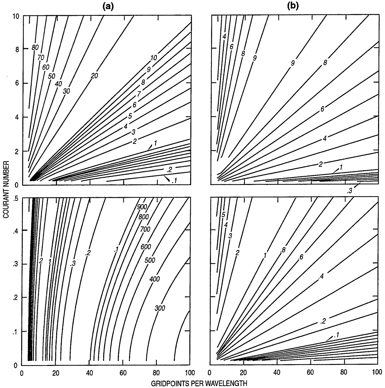
Fig. 39 — Same as Fig. 37, but for SZM. The Asselin filter coefficient for this calculation is set to 0.05.
