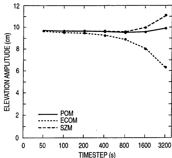
Fig. 19 — Maximum tidal elevation at west end of bay for POM, ECOM-si, and SZM for different values of the timestep. The tide was forced by specifying the elevation at the east end of the bay with an amplitude of 10 cm with a period corresponding to the M2 tide.
