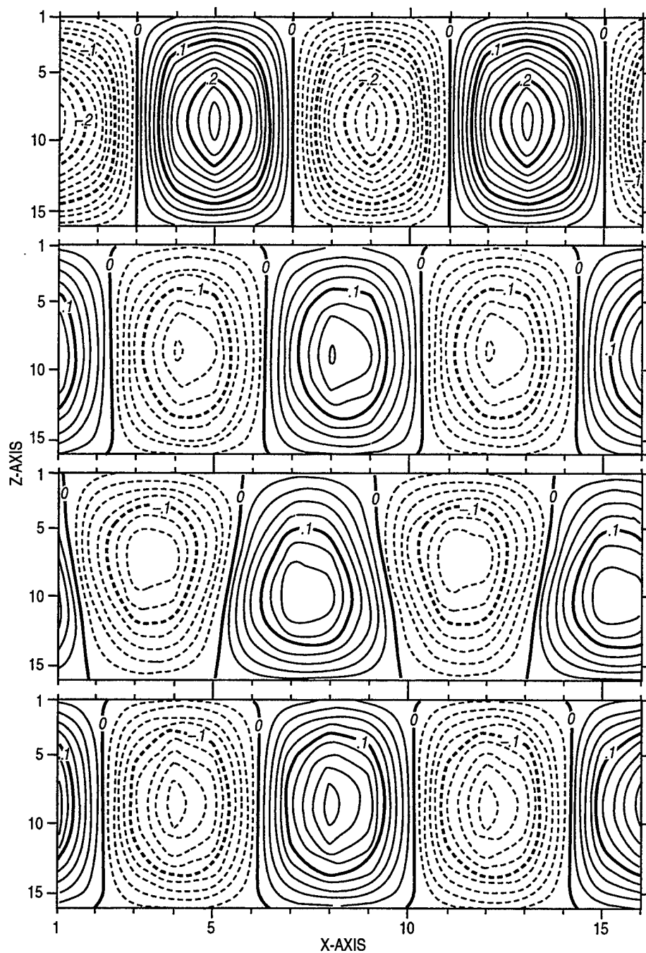
Fig. 21 — Salinity anomaly S' for propagation of internal waves of 8-km wavelength. The uppermost plot shows the initial condition and the other plots show results after 48 h for POM, ECOM-si, and SZM. The internal wave amplitude was 100 cm and the timestep was 200 s.
