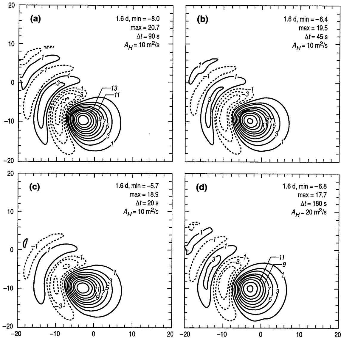
Fig. 5 — Results of rotating cone advection test after one revolution (1.6 d) with forward temporal scheme for different timestep and viscosity values
