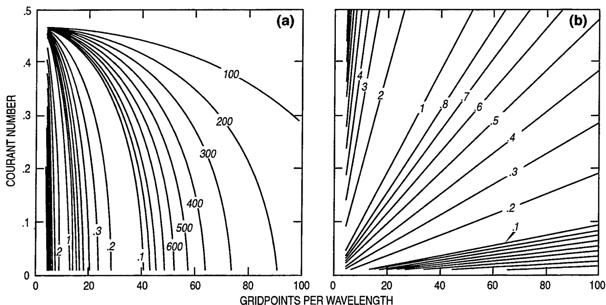
Fig. 37 — (a) Phase speed error and (b) damping for the numerical scheme used by POM for the free surface mode. The phase speed error is expressed as the percent error relative to the analytically calculated phase speed. The damping is expressed as the percent damping per wave period based on the analytically calculated wave period. The Asselin filter coefficient for this calculation is set to 0.05. Contour labels less than 0.1 are multiplied by 10,000.
