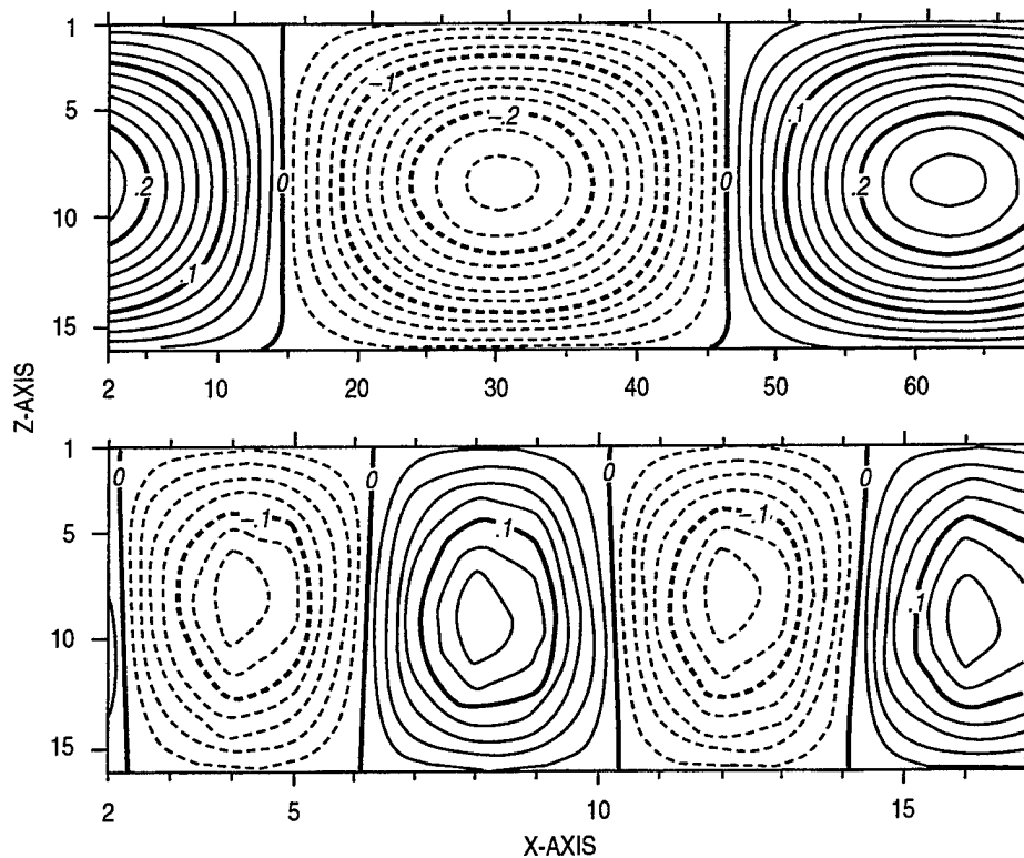
Fig. 22 — Salinity anomaly S' for propagation of internal waves of 64- and 8-km wavelengths with ECOM-si with a timestep of 50 s. The internal wave amplitude was 100 cm.
