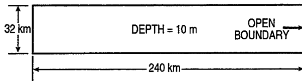
Fig. 18 — Model domain for the test problem of tides in a bay
