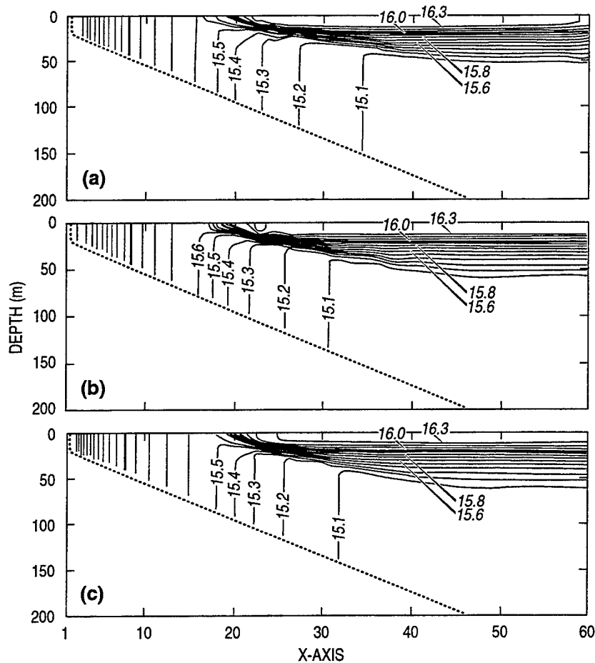
Fig. 13 — Temperature x - z sections at 30 d for the formation of a tidal mixing front for (a) POM, (b) ECOM-si, and (c) SZM. The tick marks along the horizontal axis denote the gridpoint locations. 20 sigma layers were used in the vertical, with an upper layer thickness of 5 m in deep water and a uniform stretching to the bottom.
