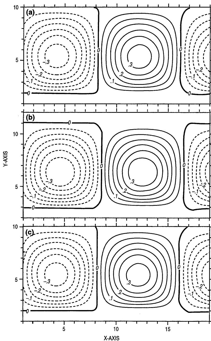
Fig. 28 — Comparison of the cross-channel velocity fields at 48 h from the models for the propagation of a barotropic shelf wave: (a) POM, (b) ECOM-si, (c) SZM. The horizontal grid spacing for the models is 8 km, and the barotropic timestep is 80 s for POM and 1600 s for ECOM-si and SZM. The contour interval is 0.05 cm/s.
