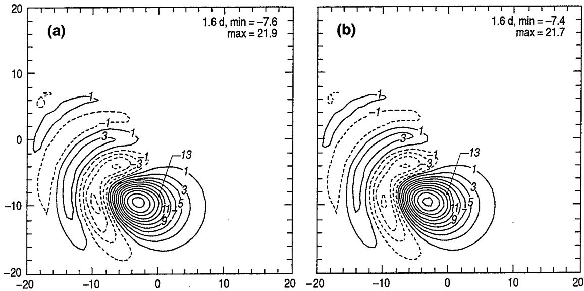
Fig. 4 — Results of rotating cone advection test after one revolution (1.6 d) for (a) leapfrog and (b) AB3 schemes with a constant horizontal viscosity of 5 \text{ m}^2/\text{s}
