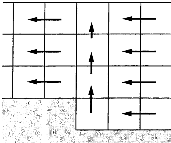
Fig. 15 — Schematic showing an x-z section for the horizontal convergence of a barotropic flow toward the coast for a model with a z-level vertical grid in which the bathymetry is rounded to the nearest z-level. The horizontal convergence is localized at the front of a step and generates a vertical jet at the front of the step.
