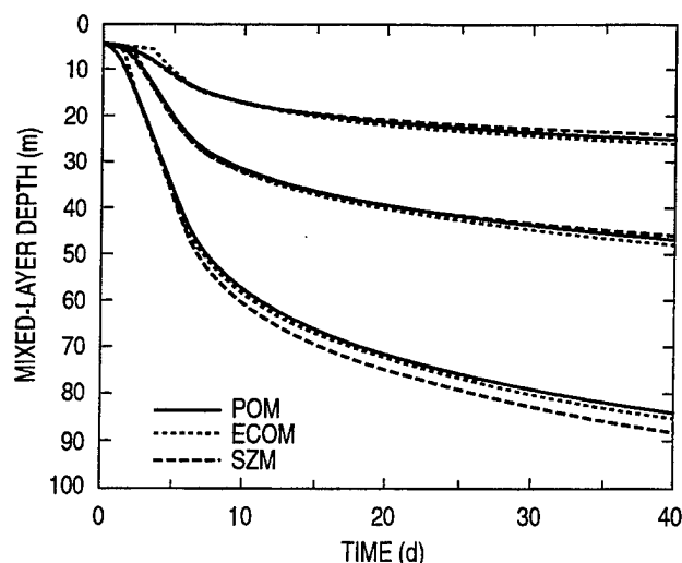
Fig. 11 — Bottom mixed-layer depth vs. time for the models for an oscillating tidal current with a period of 12.42 h. The tidal current is driven by an imposed surface pressure gradient. Three cases are shown with maximum amplitudes of the tidal current of 24, 48, and 95 cm/s. The initial condition was zero current, a constant salinity of 35 psu, and a temperature profile defined by a uniform stratification of 5°C/100 m and a bottom temperature of 19°C. The latitude is 29.91° N, where f = 2\pi/(24 \text{ h}) .
