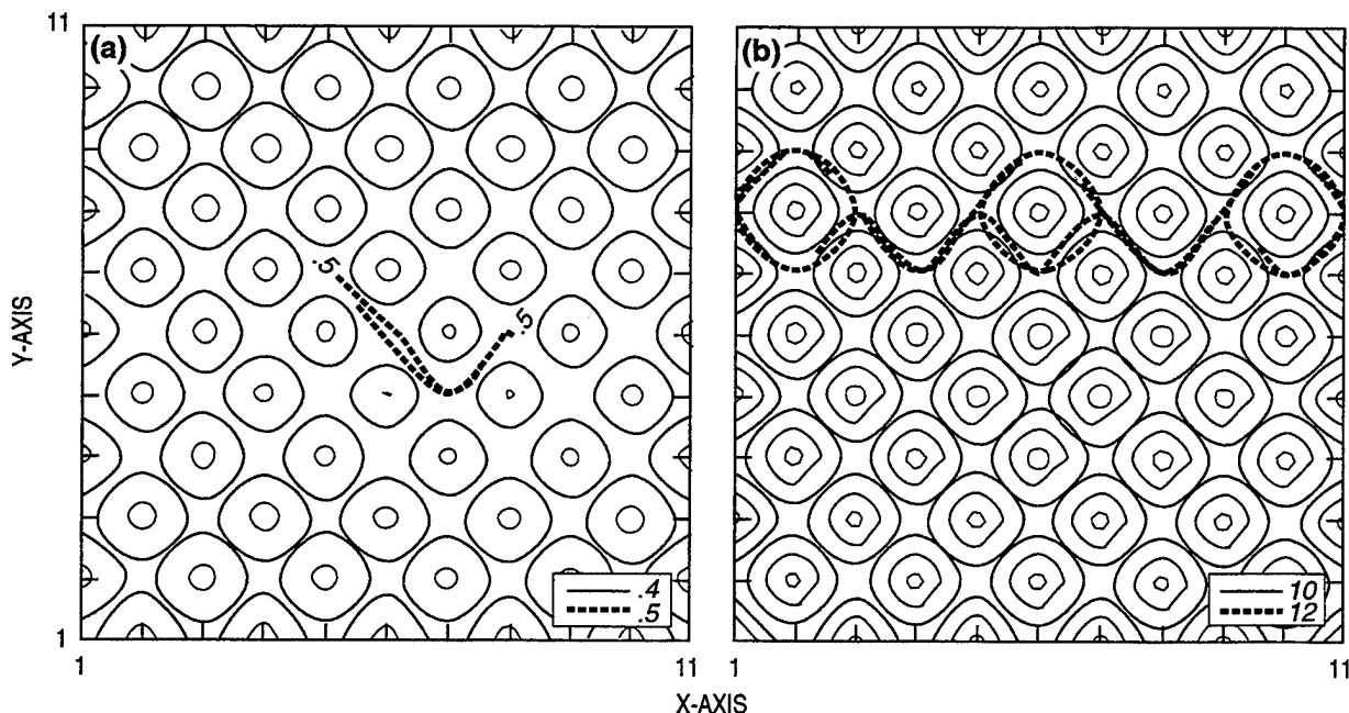
Fig. 16 — (a) SST and (b) SMLD at 2 d for the simulation of checkerboard mixing. The SMLD is defined as the depth at which the temperature is 0.2^\circ\text{C} less than the SST. The contour interval is 0.1^\circ\text{C} for the SST and 2 m for the SMLD.
