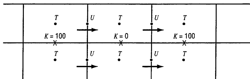
Fig. 17 — Schematic to help explain the cause of checkerboard mixing. The diagram shows an x - z section through the center of a row of grid cells.
