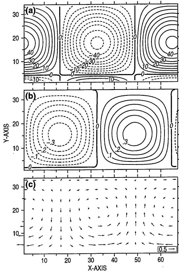
Fig. 27 — Analytical solution for a barotropic shelf wave at 48 h: (a) surface elevation, (b) cross-channel velocity, and (c) horizontal velocity vectors. The contour interval for the surface elevation is 0.005 cm and for the cross-channel velocity is 0.05 cm/s. The scaling arrow in the velocity vector plot indicates a speed of 0.5 cm/s.
