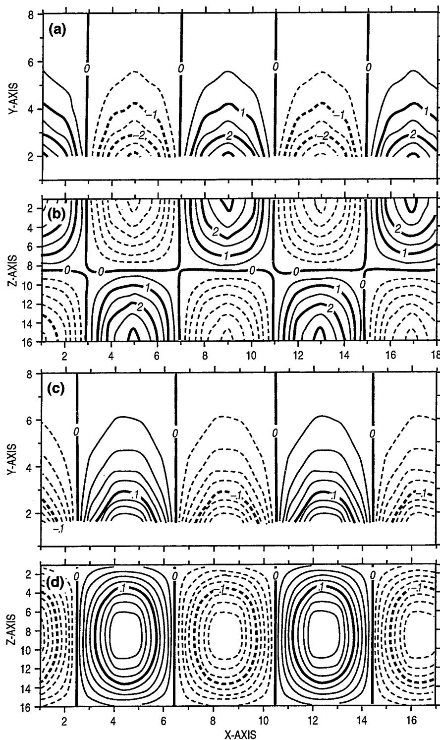
Fig. 25 — Analytical solution for an internal Kelvin wave at 48 h: (a) horizontal section of along-channel velocity u at 1.25-m depth, (b) x - z section of u at 4 km from southern boundary, (c) horizontal section of salinity anomaly S' at depth of 18.75 m, and (d) x - z section of S' at 4 km from southern boundary. Contour interval is 1.0 cm/s for u and 0.02 psu for S' .
