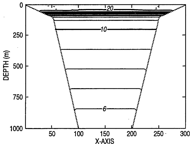
Fig. 32 — Model domain and initial temperature field for upwelling/downwelling simulations
