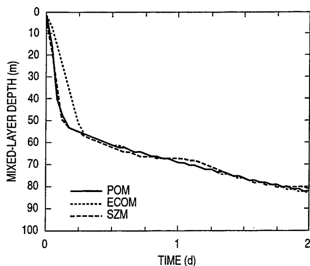
Fig. 10 — Surface mixed-layer depth vs. time for the models for convective deepening due to a surface cooling of -1000 \text{ ly/d} . The initial temperature was a constant 19^\circ\text{C} from the surface to 50 m, followed by a linear decrease to 18.5^\circ\text{C} at 100 m. The surface wind stress was 1 \text{ dyne/cm}^2 .
