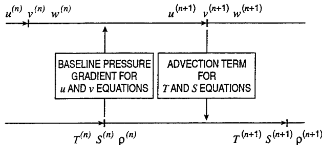
Fig. 40 — Schematic showing the effective leapfrogging in time of the momentum and salinity conservation equations of ECOM-si for the main internal gravity wave terms
