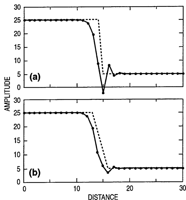
Fig. 6—Results of advective overshoot experiment with second-order, centered advection scheme. The dashed line shows the initial temperature and the solid line shows the predicted temperature at the time of maximum overshoot. In (a), the initial temperature jump occurs between two gridpoints and in (b) it is distributed (linearly) over four gridpoints. The gridpoint locations are indicated by tick marks along the distance axis and also by dots at the predicted temperature values.
