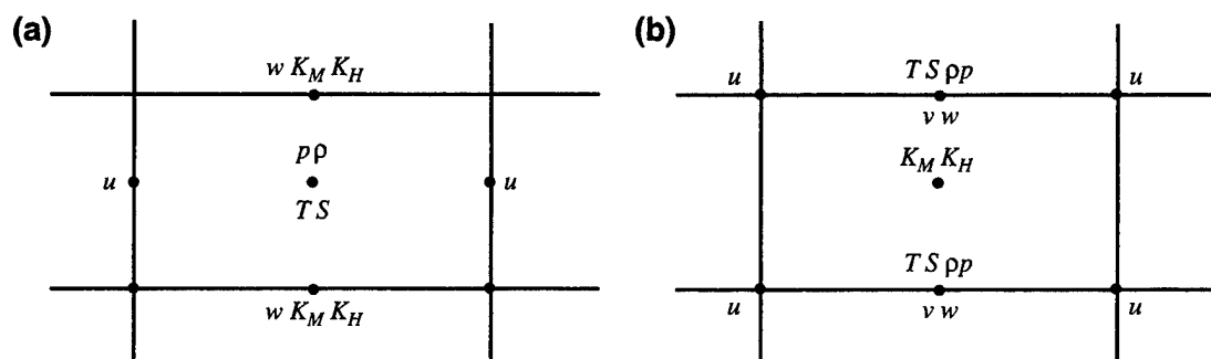
Fig. 2 — Vertical arrangement of primary model variables on the numerical grid for (a) POM, ECOM-si, and SZM and (b) SCRUM
