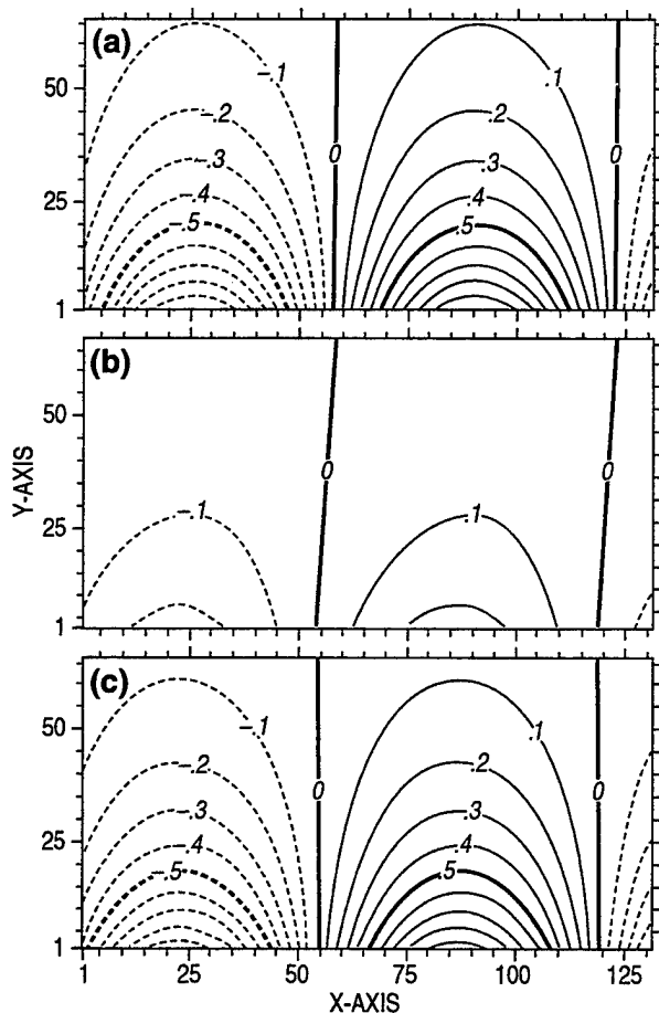
Fig. 24 — Comparison of surface elevation (cm) from the models at 48 h for the propagation of a surface Kelvin wave: (a) POM, (b) ECOM-si, and (c) SZM. The horizontal grid spacing was 10 km and the baroclinic timestep was 1800 s.
