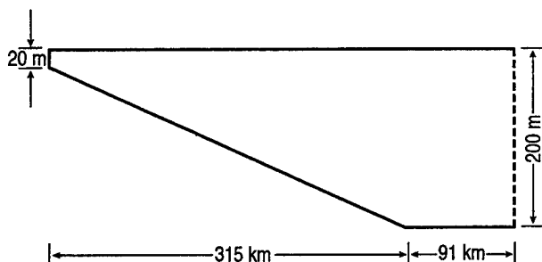
Fig. 12 — Schematic showing the model domain used for the problem of the formation of a tidal mixing front
