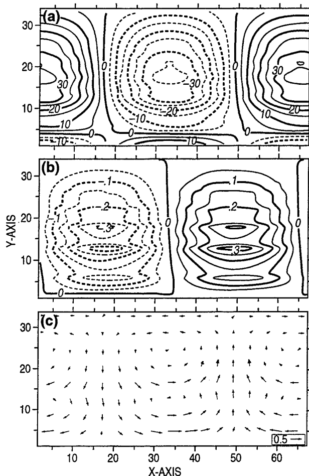
Fig. 29 — (a) Surface elevation, (b) cross-channel velocity, and (c) horizontal velocity vectors at 48 h for a shelf wave simulated by SZM with a z -level vertical grid with \Delta z = 10 m. The horizontal grid spacing is 2 km and the timestep is 400 s. The contour interval is 0.005 cm for the surface elevation and 0.05 cm/s for the cross-channel velocity. The representative scaling arrow in the velocity vector plot indicates a speed of 0.5 cm/s.
