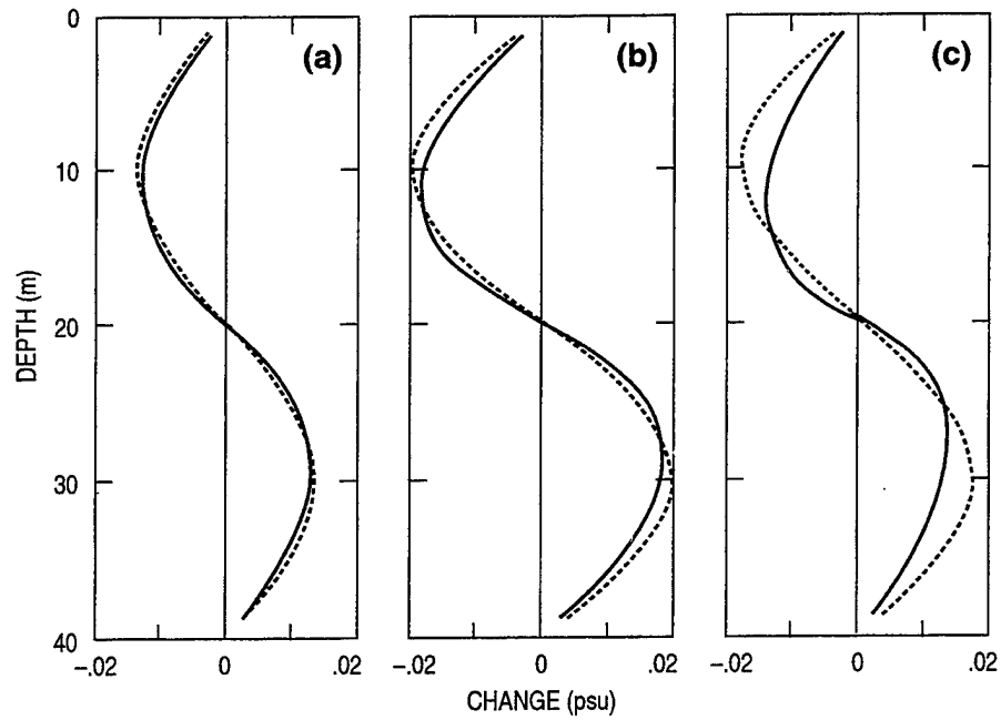
Fig. 41 — Change in ambient stratification during internal wave propagation for ECOM-si (solid line) and as predicted by numerical analysis (dashed line) after 24 h. The wavelength is 8 km. The internal wave amplitude and timestep are (a) 100 cm and 200 s, (b) 200 cm and 200 s, and (c) 400 cm and 400 s.
