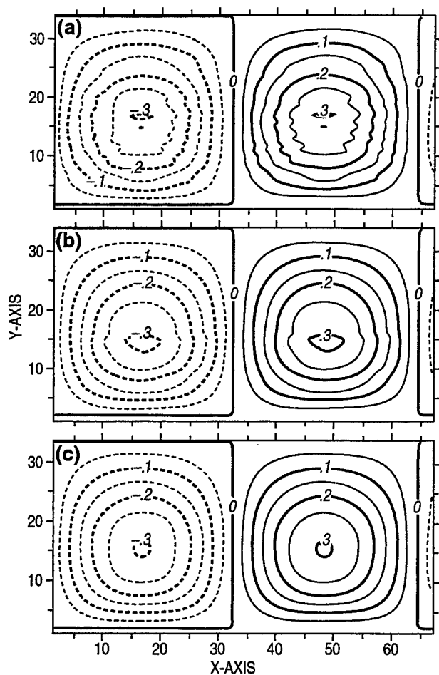
Fig. 31 — Cross-channel velocity fields at 48 h for the propagation of a barotropic shelf wave with SZM for different z-level vertical grids: (a) 30 uniformly spaced z-levels, (b) 60 uniformly spaced z-levels, and (c) 51 z-levels with variable spacing so as to exactly resolve the exponentially varying bathymetry. The horizontal grid spacing for these results is 2 km and the timestep is 400 s.
