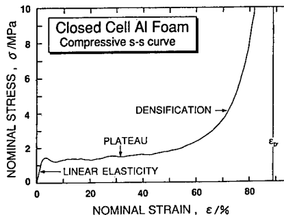
Fig.9 Compressive stress-strain curve
