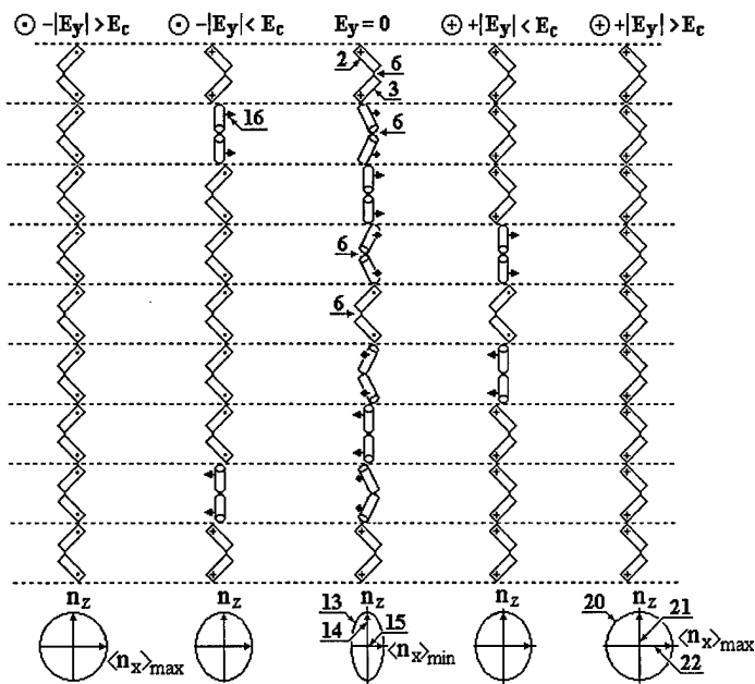
Fig.12. Ferroelectric packing of neighbour smectic layers, composed from banana shape molecules.
