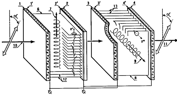
Fig.6. Polarization non-sensitive DHF phase modulator composed from two crossed DHF cells.
