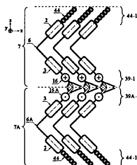
Fig.43. Antiferroelectric packing of the neighbour layers 7 and 7A. The dipole moments in neighbour layers have opposite directions. The tips 6 and 6A, respectively, have the same directions.
