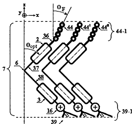
Fig.22. The polyphilic molecules with the perfluorinated chain 44 connected to the aliphatic hydrocarbon tail 36 outside of central core 2.
