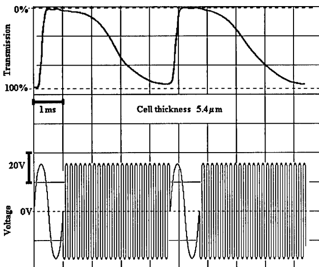
Fig.31. The response oscillogram of nematic liquid crystal with change of sign of dielectric anisotropy. The low frequency is 1kHz, the high frequency is 20kHz. Cell thickness 5.4\mu\text{m} . Nematic liquid crystal ZhKM-1001 (NIOPIC, Moscow, Russia).
