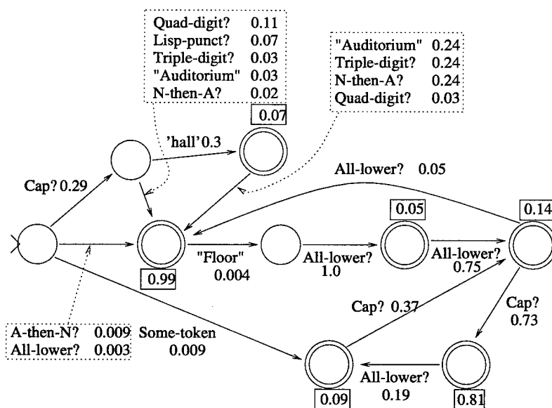
FIGURE 4.7: A small piece of an automaton, used for recognizing seminar locations, learned by Alergia using a decision list created with m -estimates.
