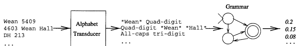
FIGURE 4.6: The pipeline through which raw text fragments are passed to produce structure estimates.
