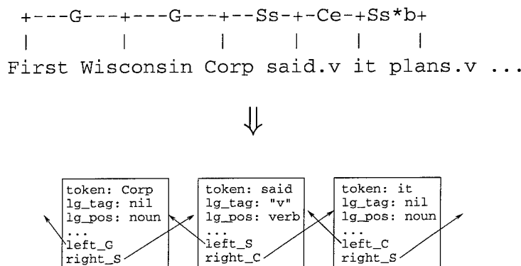
FIGURE 5.7: An example of link grammar feature derivation.
