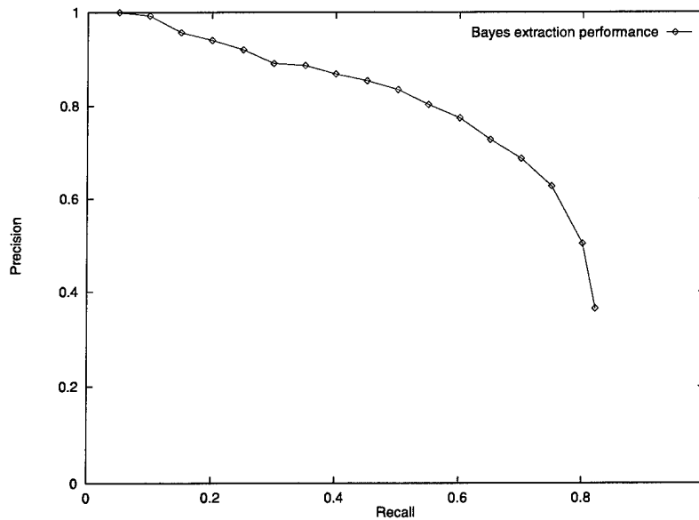
FIGURE 2.9: A precision/recall graph.
