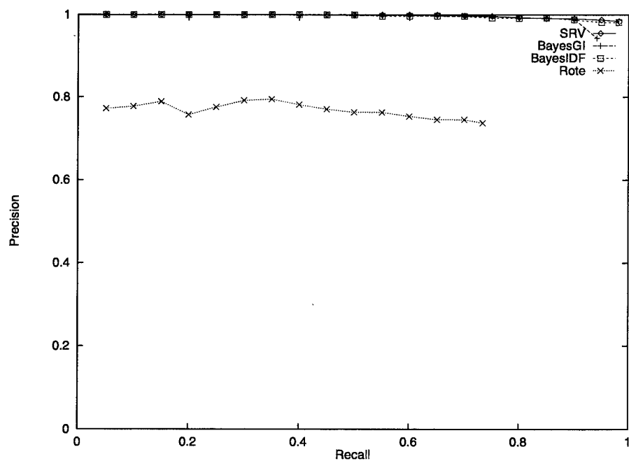
FIGURE 5.12: Precision/recall plot comparing all four learners on the time field from the seminar announcement domain.
