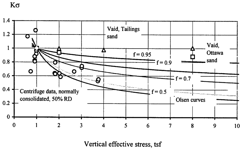
Figure 3.11 Comparison between Figure 2 data expressed as K\sigma at 10 cycles, compared with Olsen, 1984 and data from Vaid for Tailings and Ottawa sand
