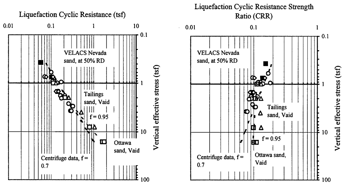
Figure 3.12 Stress focus plots using centrifuge data, normally consolidated, at 50% RD, compared with VELACS laboratory test data on Nevada sand corrected to 50% RD (CIUCyclic solid squares, CSS open diamonds) and 10 cycles, and data from Vaid at 50% RD on Tailings sand and Ottawa sand.
