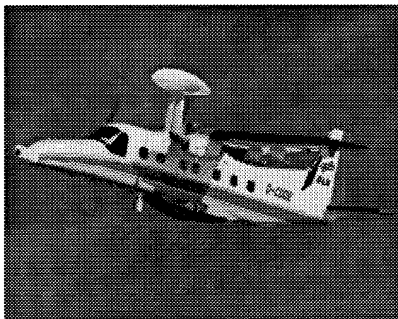
Fig. 4.2: DASA HiVision radar mounted on top of a DO-228.
