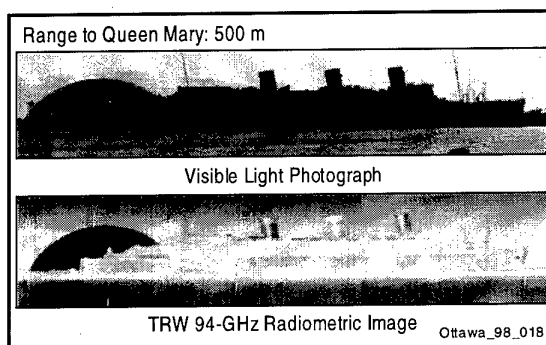
Figure 21. Passive Imaging mmW Sensors Provide High Contrast
