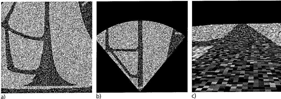
Fig. 4.5: Different radar image representations of the same scene. a) range-angle (B-scope), b) radar-map (PPI-scope), c) "out-the-window-view" (C-scope).
