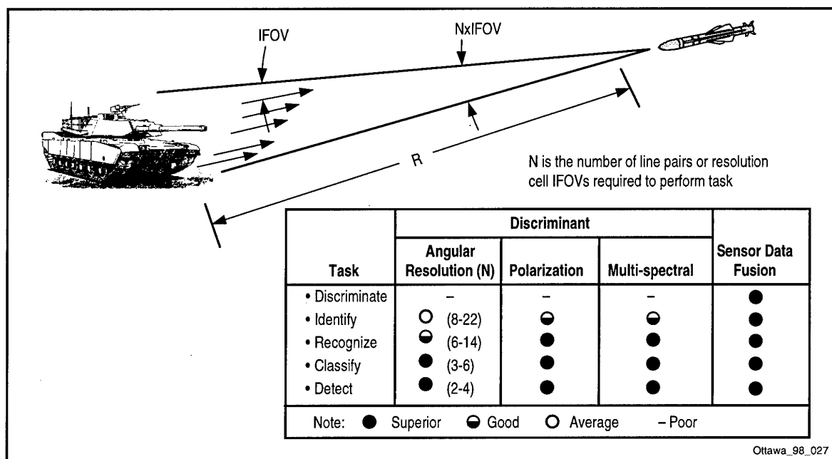
Figure 27. Example of Benefit of Sensor Data Fusion
