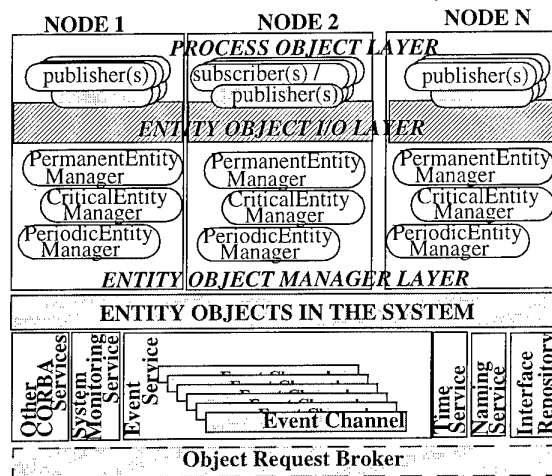
Figure 4. General Schema of the Proposed Architecture
