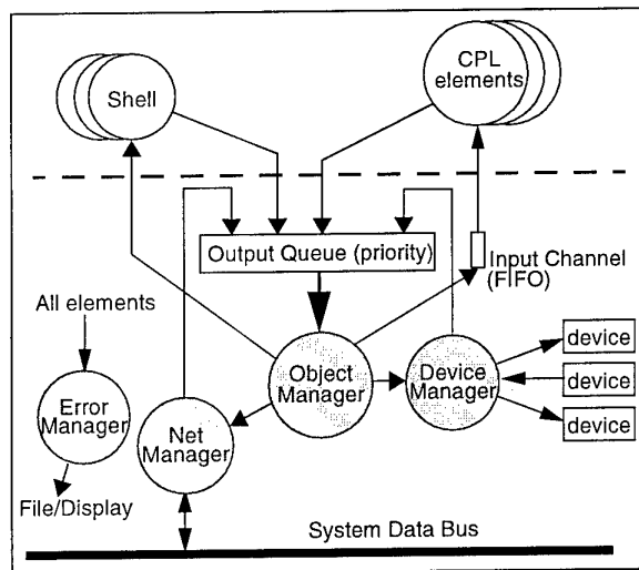
Figure 2. The CORD system infrastructure
