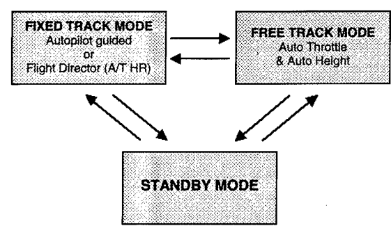
Figure 4: Care Free Moding Concept
