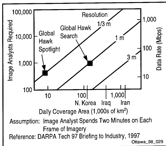
Figure 2. Automated Systems are Required for C4ISR Image Analysis
