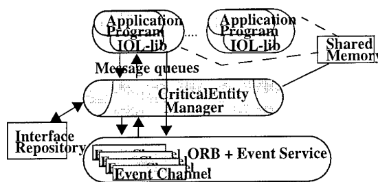
Figure 5. Detailed representation of the CEM part of the proposed infrastructure
