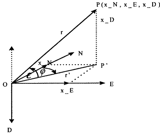
Figure 2.2-1 Definition of Spoke Coordinates In the NED frame
