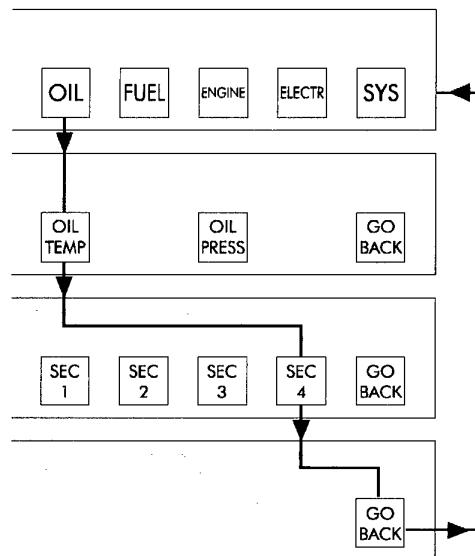
Figure 11: Typical operational process in the AMS system-hierarchy.
