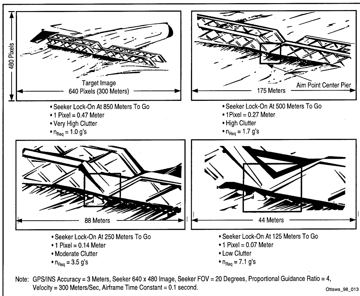
Figure 16. Precision GPS/INS Facilitates Targeting in a Clutter
