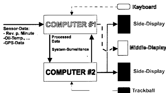
Figure 7: Schematic structure of the electrical system components.
