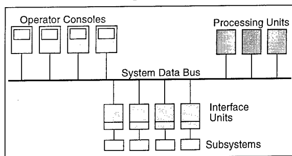
Figure 5. Distributed system architecture
