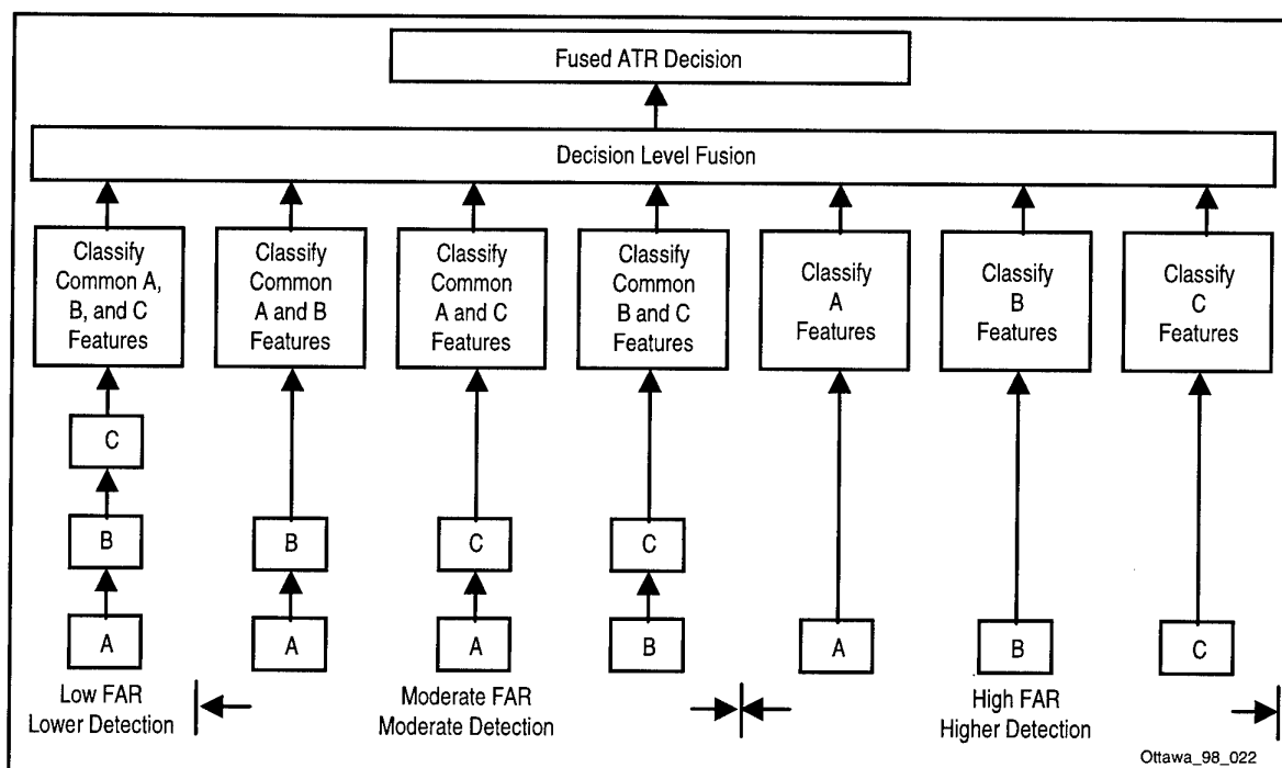
Figure 25. Example of Robust Sensor Data Fusion Architecture for Low FAR and High Detection ATR
