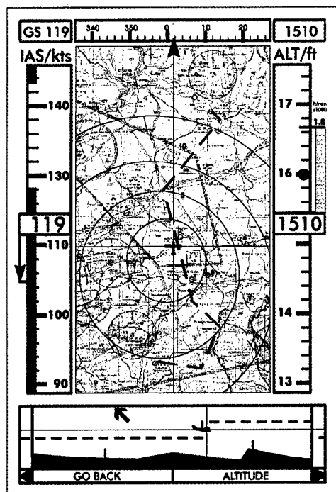
Figure 16: FPNS with active 'side-view' and circles of equal flight-time in the map area (flight-mode status).
