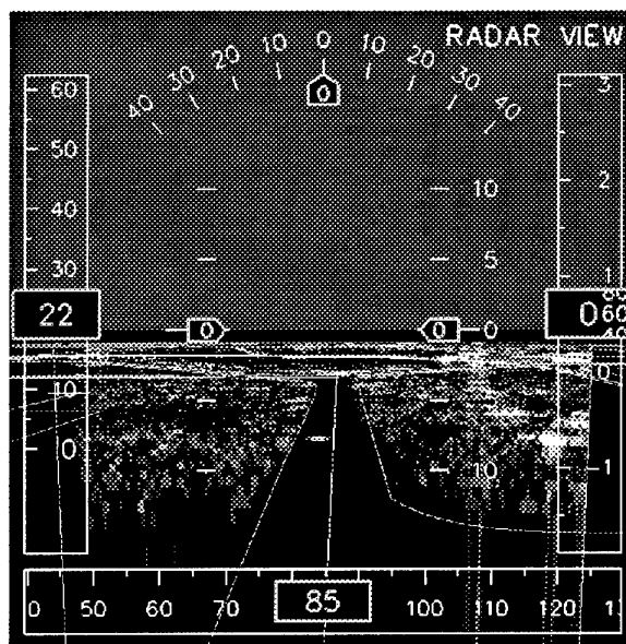
Fig. 4.6: Design example for a fused EVS-display: perspective radar view with overlaid terrain data and PFD-symbolology.
