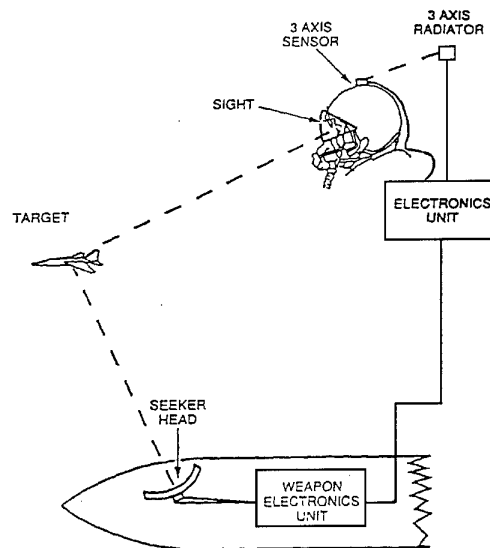
Figure 1-4 Use of head pointing in an off-bore-sight capability weapon system
