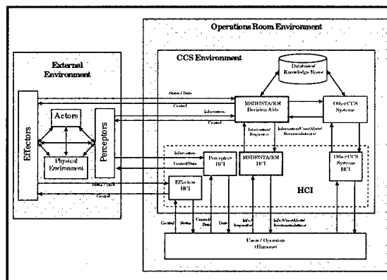
Figure 10. Operations room environment with DSS
