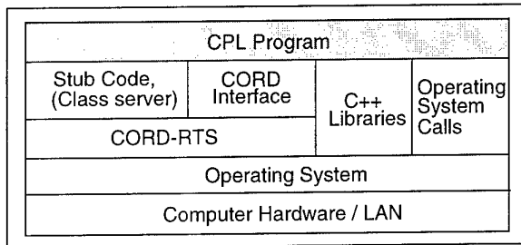
Figure 3. Software architecture
