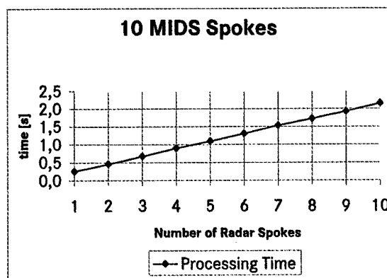
Figure 8.3-1: total processing times with 10 MIDS Spokes and variable number of Radar Spokes
