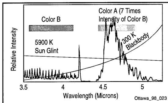
Figure 23. Example of Unique Two-Color IR Signature of Missile Plume
