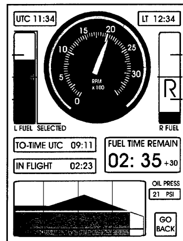
Figure 12: AMS-display in proceeding-level I status (oil pressure turned 'amber').
