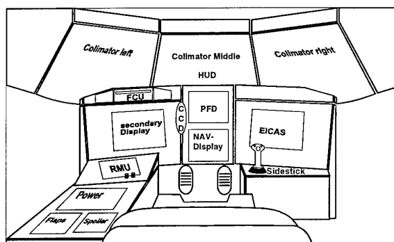
Figure 2: Experimental Simulator Configuration
