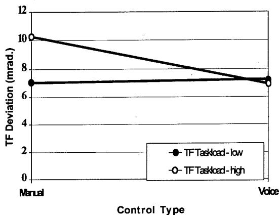
Figure 6. Terrain Following (TF) Deviation during Navigation as a Function of Control Type With High Auditory Task Load
