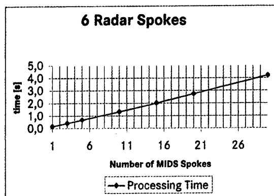
Figure 8.3-2: Processing time over MIDS Spoke number by maintaining the number of Radar Spokes constant.
