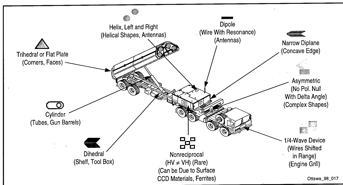
Figure 20. SAR Full-Polarization Scatter Physical Basis
