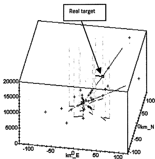
Figure 8.2-1: 6 Radar and 10 MIDS Spokes with a real target placed in the random scenario
