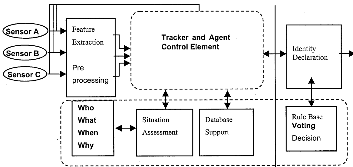
Figure 4 – OPTIMISED SYSTEM ARCHITECTURE
