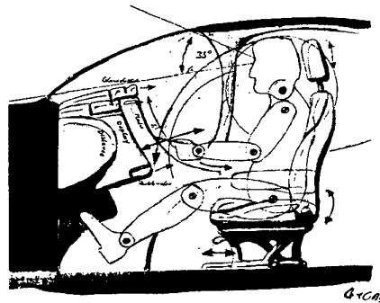
Figure 9: Sketch of the new cockpit concept, showing ergonomic details (side view).
