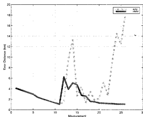
Figure 5.e : Distance error for IMM and HMM
