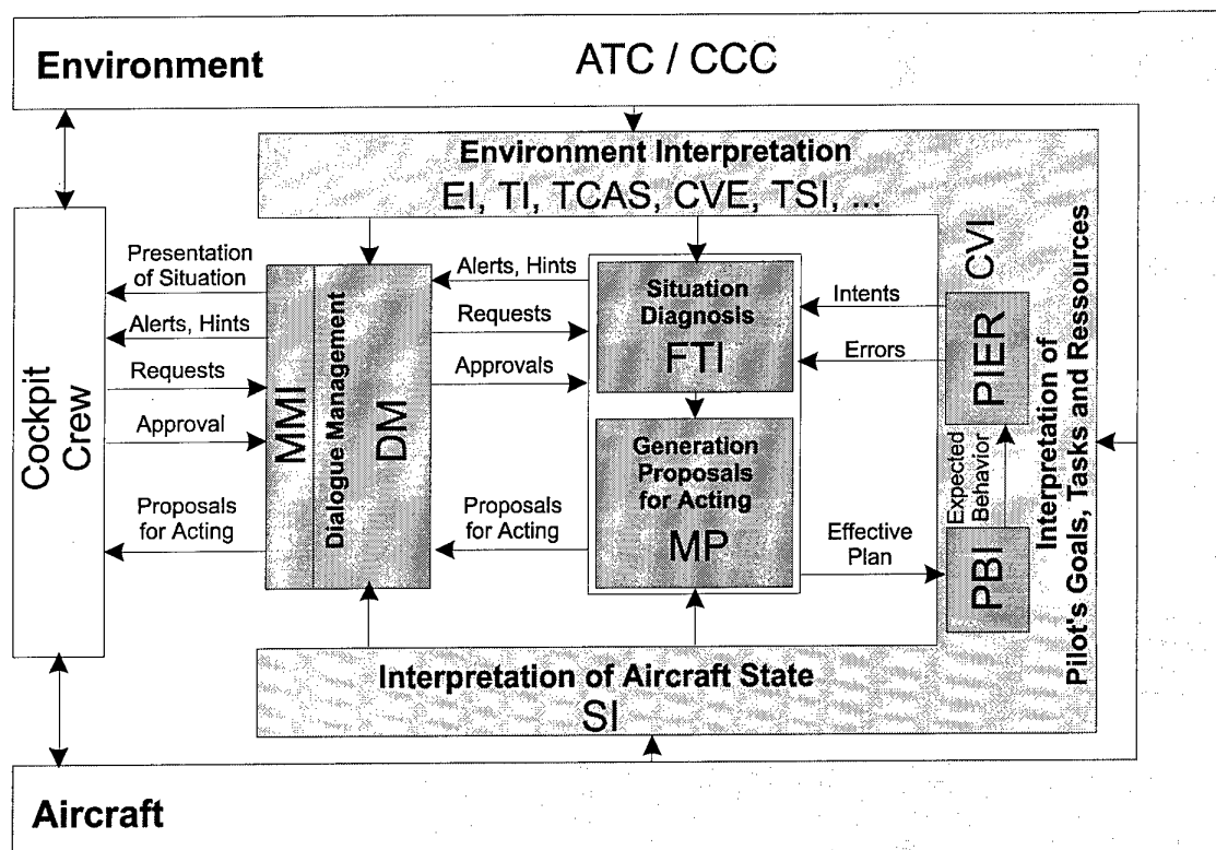
Figure 1: Functional Structure of the Crew Assistant Military Aircraft.
