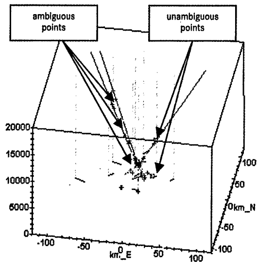
Figure 8.1-1: 6 Radar + 10 MIDS Spokes without any range estimates available.
