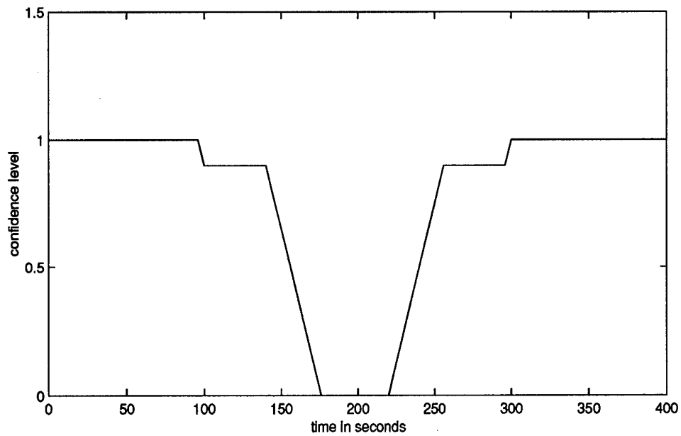
Figure 7 - Variation of coefficient \beta according to time used in application 2
