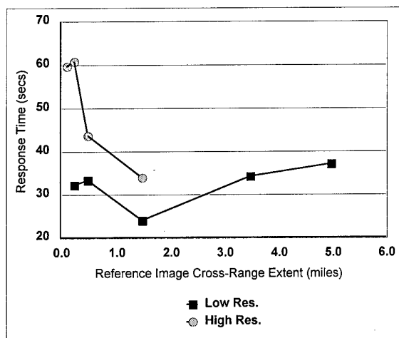
Figure 6. Response Time as a function of Reference Image Cross-Range Extent and Source Database Resolution for the Medium FLIR Sensor Distance.
