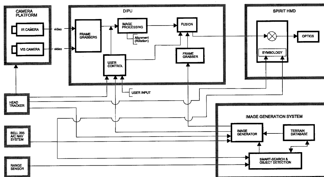
Figure 2 ESVS Architecture Block Diagram
