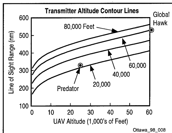
Figure 11. High Altitude UAVs Provide Long Range C4ISR and Safe Operation Above Commercial Aircraft
