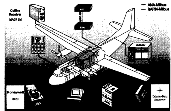
Figure 9: RAPIN in C160 Transall
