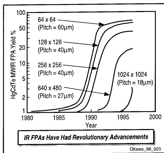
Figure 24. Example of Advancement in SOTA of IR FPAs
