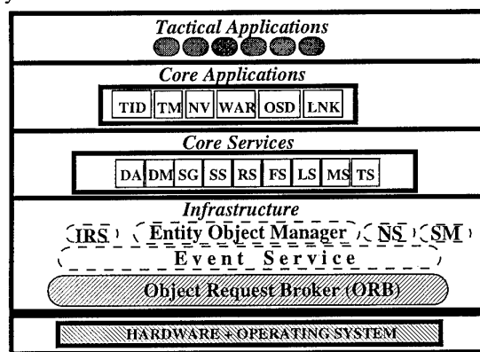
Figure 3. Overall Design for a C2 system
