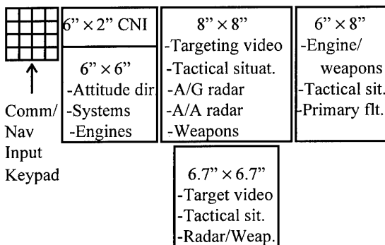
Figure 2. Head-Down Display Configuration (Ref 16)
