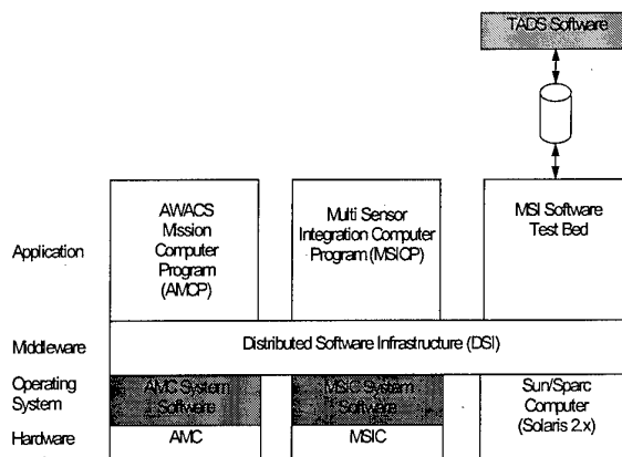
Figure 2-2 Software Layers (Test Configuration)
