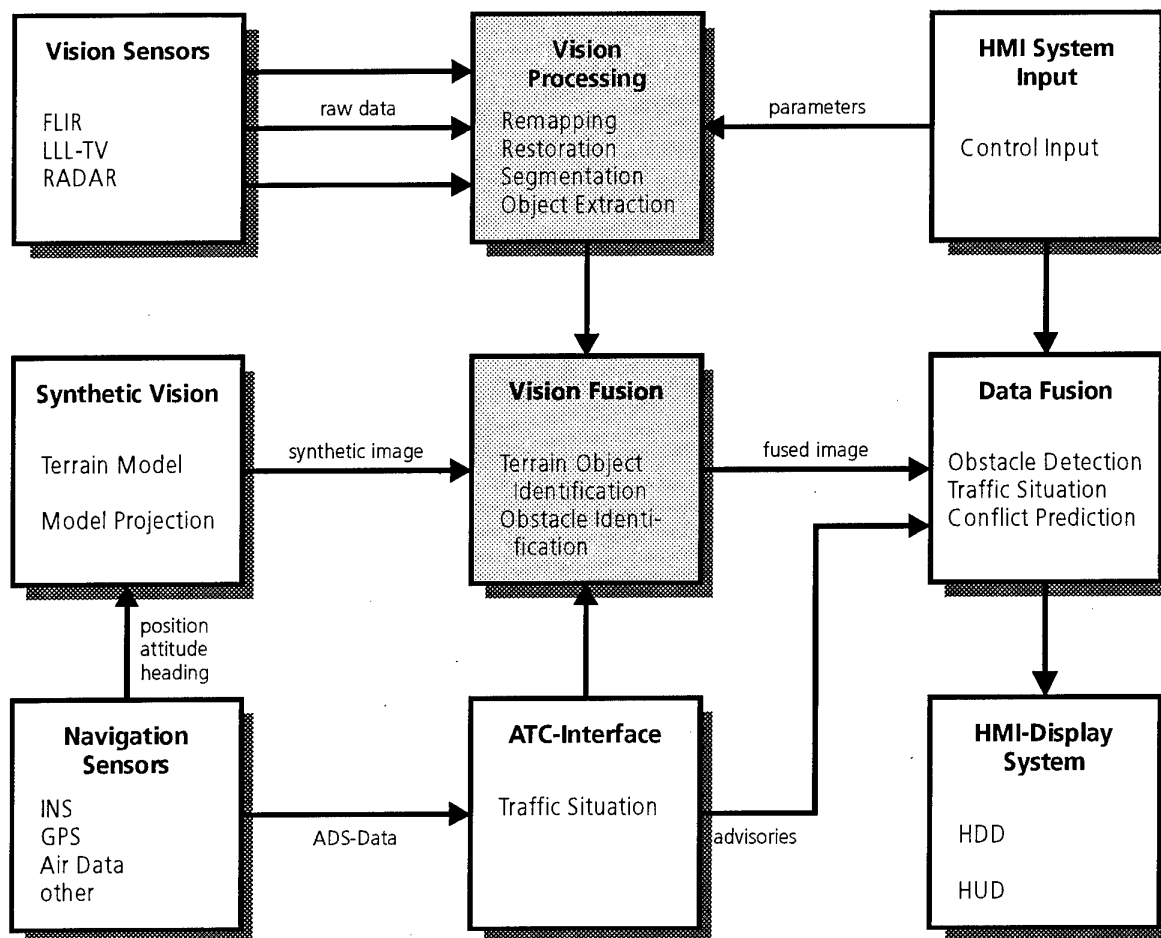
Fig. 2.1: Block Diagram of the DLR "Integrated Enhanced Vision System".
