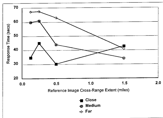
Figure 3. Response Time as a function of Reference Image Cross-Range Extent and FLIR Sensor Distance for the High Resolution Data
