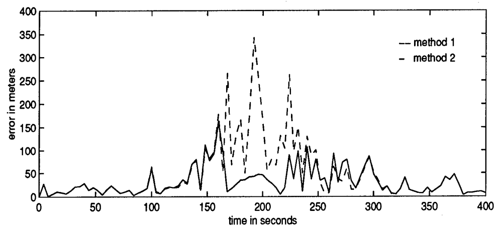
Figure 8 - Absolute error of estimated trajectory in application 2
