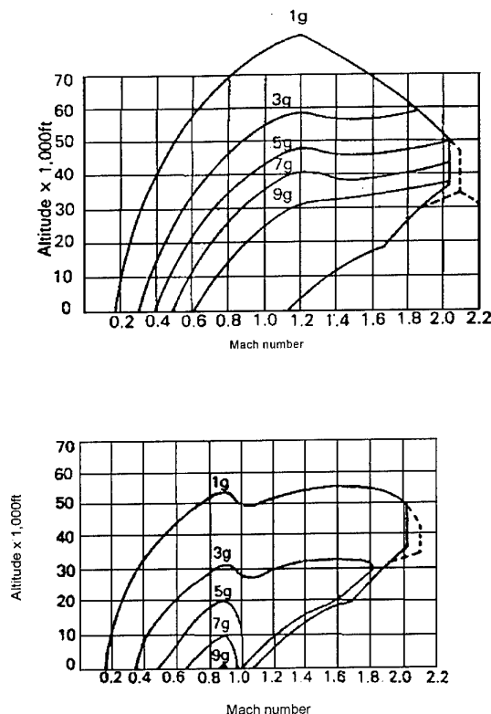
Figure 1-3 Instantaneous (upper) and sustained (lower) manoeuvre capability of the F-16/79
