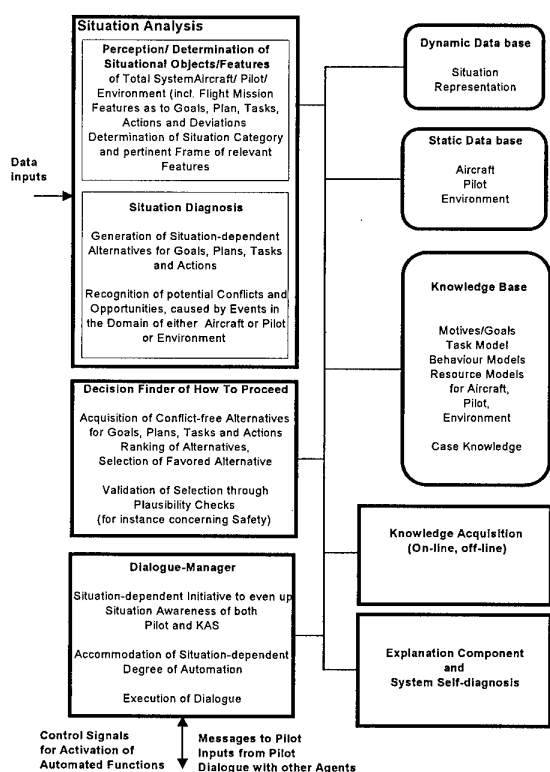
Figure 3: Structure of a Cognitive Assistant System.
