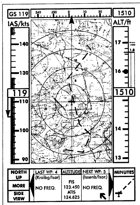
Figure 13: FPNS on side-displays (flight-mode status).
