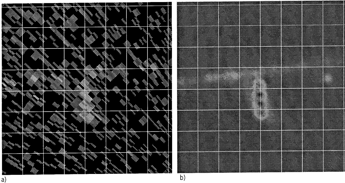
Fig 4.8: Noise reduction in a PPI-scope image (grid-size 20 m). a) detail of single radar image, b) the same part after fusion of 50 single images (approx. 3 seconds of data).
