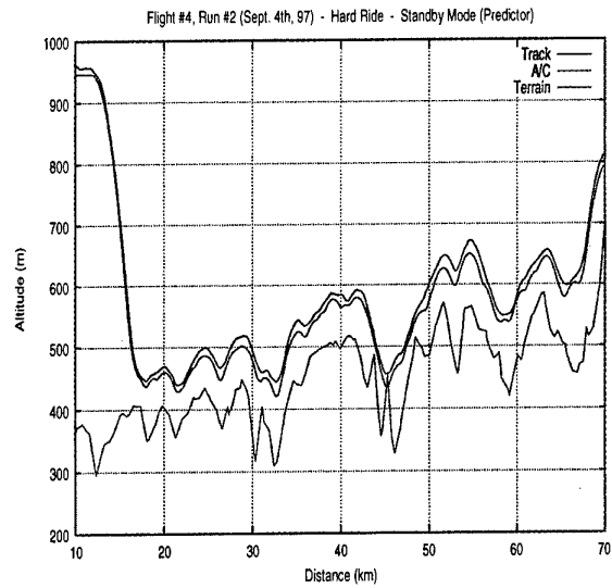
Figure 14: LLF Results - Vertical Profile
