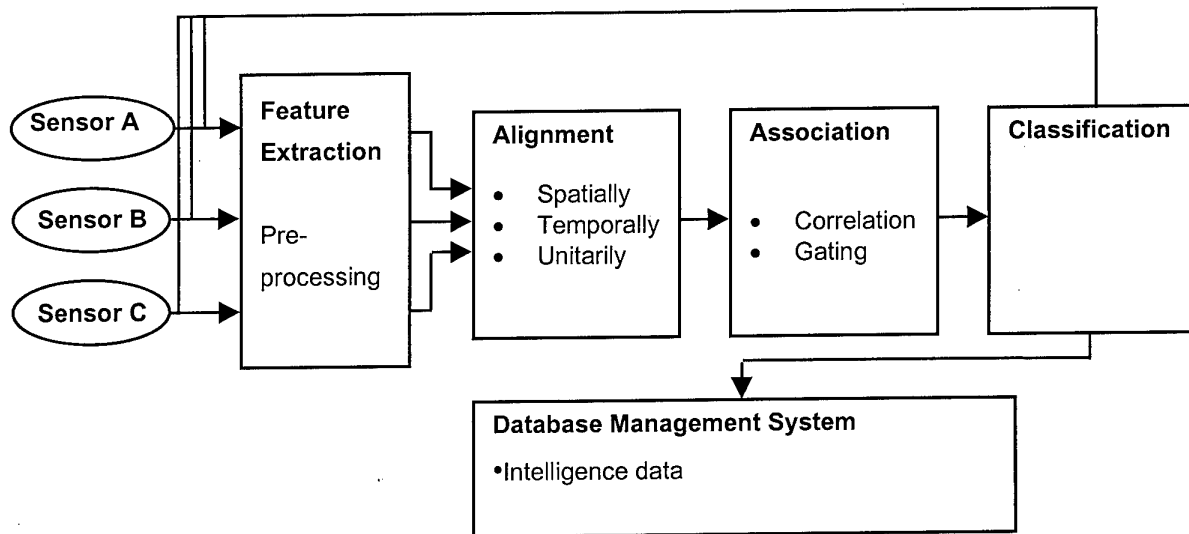
Figure 2 – ARCHITECTURE FOR FEATURE LEVEL MULTISENSOR IDENTITY FUSION
