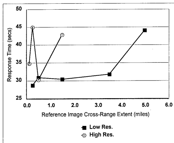
Figure 5. Response Time as a function of Reference Image Cross-Range Extent and Source Database Resolution for the Close FLIR Sensor Distance.
