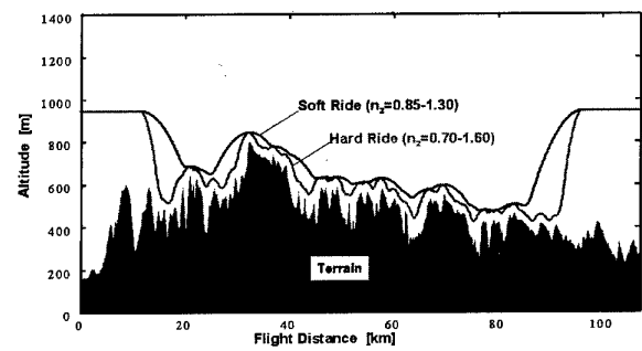
Figure 7: Ride Comfort
