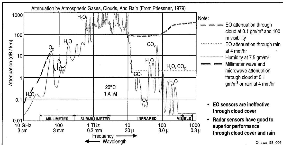
Figure 8. Signal Attenuation Due to Weather
