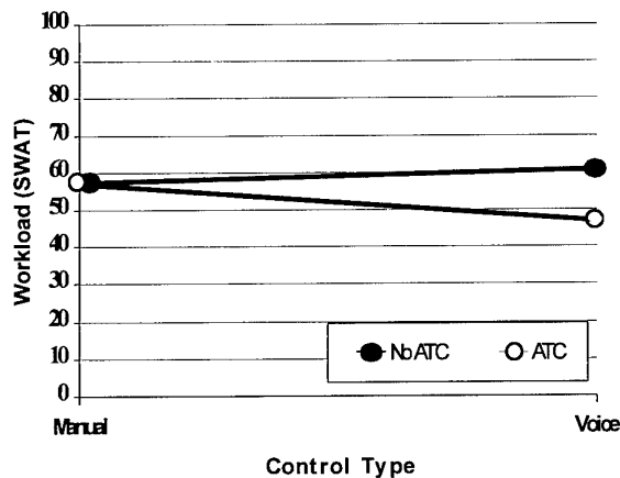
Figure 9. Pilot Workload during Weapon Delivery as a Function of Control Type With and Without Auto-Target Cueing
