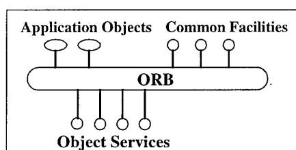
Figure 2. The Components of Object Management Architecture (OMA)
