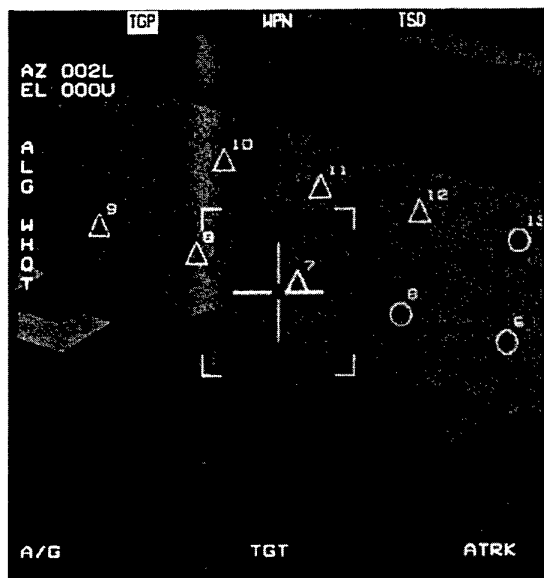
Figure 3. Target Designation Symbology with Auto-Target Cuer (ATC)
