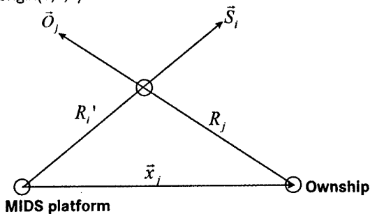
Figure 5.2-1 Geometric Basis for Triangulation
