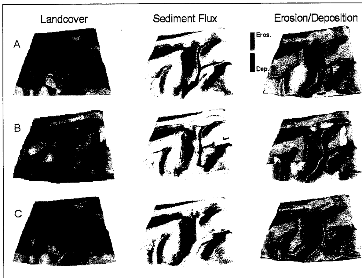
Figure 10. Estimates of sediment flux and spatial patterns of erosion and deposition predicted by SIMWE. Graphics represent the original distribution of grass (green) vs. cultivated area (brown) at the Scheyern Experimental Farm (A), the new design (B), and the design optimized by SIMWE (C).
