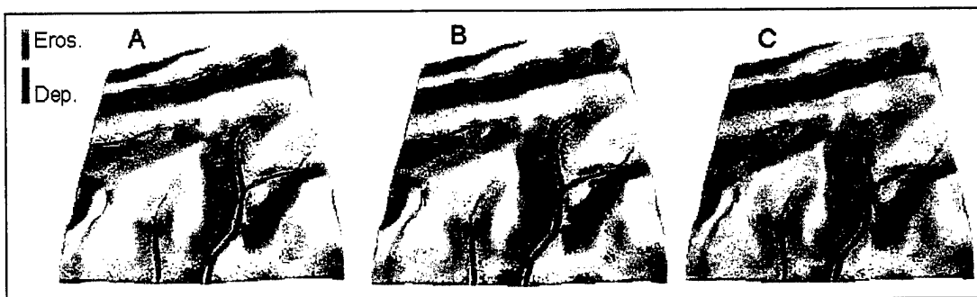
Figure 4. Effect of increasing rainfall excess. Graphics show an increase from 36 mm/hr (A) to 72 mm/hr (B) to 114 mm/hr (C).
