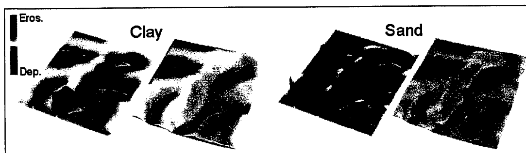
Figure 7. The effect of soil type on sediment flux and erosion/deposition patterns. Clayey soils are difficult to detach (low detachment capacity) but easy to transport (high transport capacity); sandy soils have high detachment capacity but low transport capacity. Left graphic in each pair shows sediment flux; right graphic shows erosion/deposition patterns.
