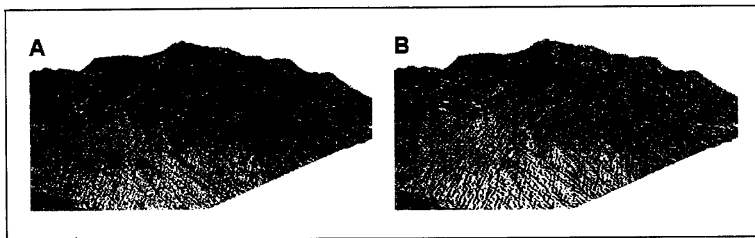
Figure 12. Terrain with draped tangential curvature using the original 30-m DEM (A) and with a resampled 10-m DEM with smoothing (B).
