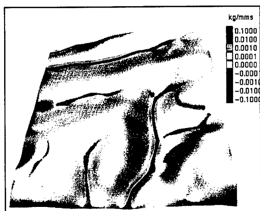
Figure 11. Impact of terrain structures on water and sediment flow and net erosion/deposition under uniform conditions. A sediment retention basin has been simulated near the left margin of the figure. The simulation shows significant deposition in the basin. A simulated terrace is seen as the crescent shape near the right side of the figure. Note that deposition occurs above the terrace, but erosion occurs on the downslope side of the terrace.
