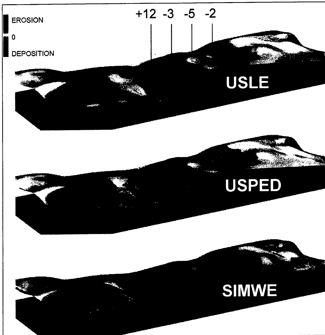
Figure 2. A comparison of the topographic potential for erosion and deposition for the traditional USLE, the unit stream power analog (USPED), and SIMWE. Soil samples were taken from the locations represented by the green dots. The samples were analyzed for cesium-137 content as an index to erosion and deposition. Net loss or gain of cesium-137 (see numbers at the top) represent proportional levels of erosion and deposition, respectively. The blue band below each figure is an exaggerated depiction of relative sediment deposits as determined by soil cores. Data is from the Scheyern Experimental Farm, Germany, courtesy of Dr. Karl Auerswald.
