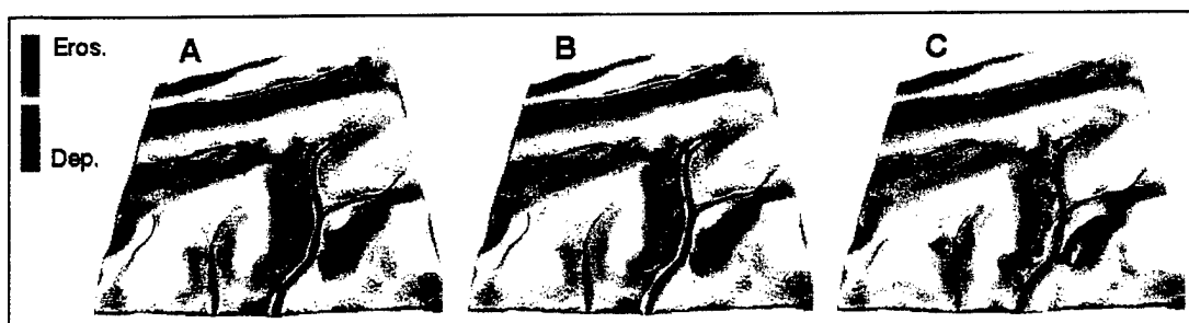
Figure 6. Changing patterns of the intensity and spatial distribution of erosion and deposition. Graphics show change resulting from increasing the critical shear stress of the soil from 1 (A) to 3 (B) to 7 (C).
