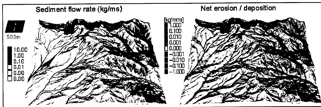
Figure 14. Sediment flow rate and net erosion/deposition as predicted by the SIMWE model using a 30-m resolution DEM resampled and smoothed to 10-m resolution.
