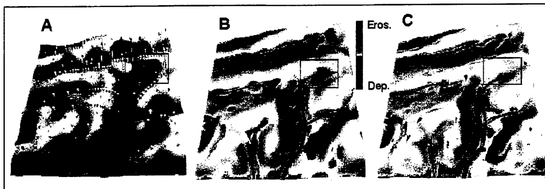
Figure 3. A comparison of measured colluvial deposits. Graphics show (A) with predicted erosion and deposition applying to USPED with 2D (B) vs. 1D (C) flow, i.e., with and without incorporation of the tangential curvature, respectively.
