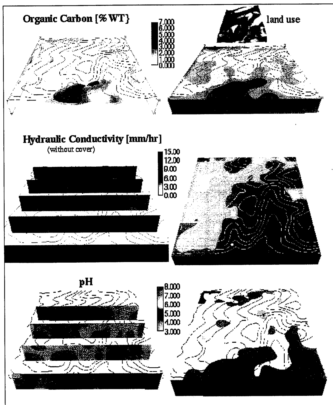
Figure 9. Three-dimensional visualization of soil organic matter content, hydraulic conductivity, and pH. The vertical profile has been exaggerated 100x to facilitate visualization. The small insert labeled "land use" shows cultural practices at the time the data were collected; the brown areas represent cultivated areas while the green areas are grassed.
