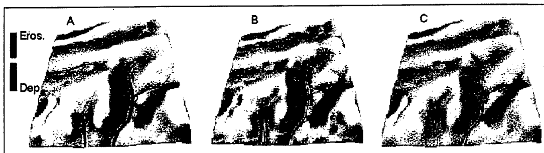
Figure 8. Erosion and deposition as a result of using different equations. Graphics represent the Julen and Simon equation with m=1.5 (A) and m=0.6 (B), and the Mitas and Mitasova equation (C).
