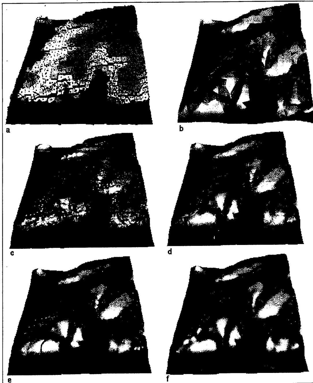
Figure 1. Interpolation of a digital elevation model (DEM) from scattered data points. Graphics represent (a) Voronoi polygons, (b) triangulated irregular network (TIN) based linear interpolation, (c) inverse distance weighting, (d) ordinary kriging, (e) spline with tension and stream enforcement, and (f) regularized spline with tension and smoothing. The data is from the Scheyern Experimental Farm, Germany, courtesy of Dr. Karl Auerswald.
