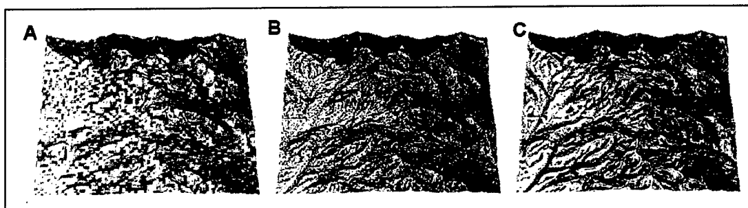
Figure 13. The topographic potential for net erosion and deposition as predicted by the USPED model using DEM resolutions of 90 (A), 30 (B), and 10 m (C).
