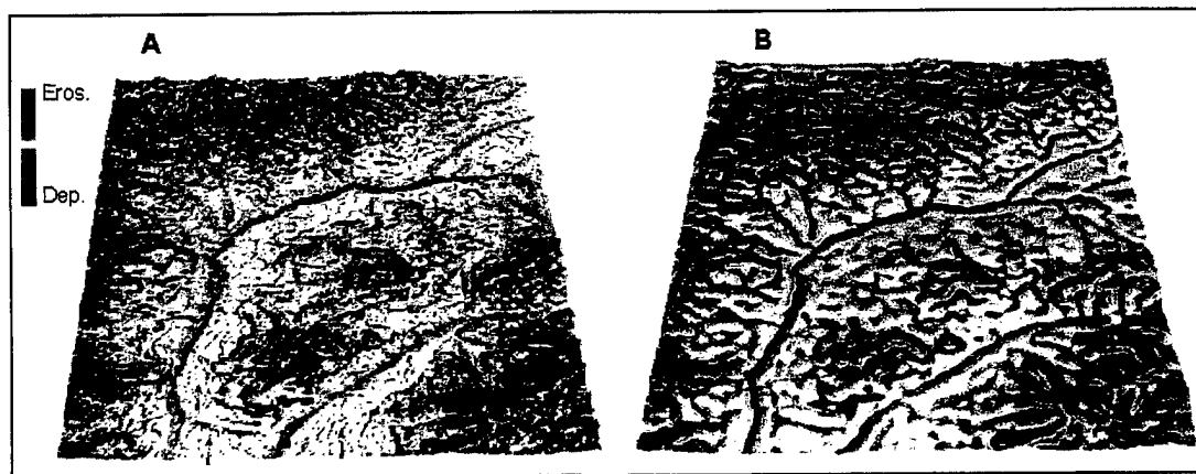
Figure 15. Topographic potential for erosion and deposition as predicted by the USPED model using a 30-m resolution DEM (A) and a 10-m resolution DEM (B) created by resampling and smoothing the 30-m DEM.
