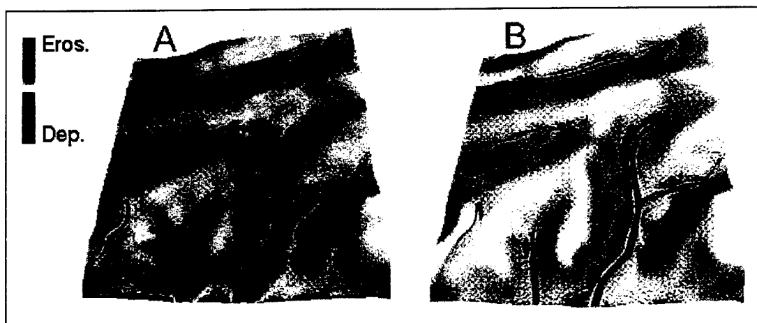
Figure 5. The effect of increasing surface roughness on erosion and deposition. Graphics show Manning's N=0.01 (smooth, A) and 0.10 (rough, B).
