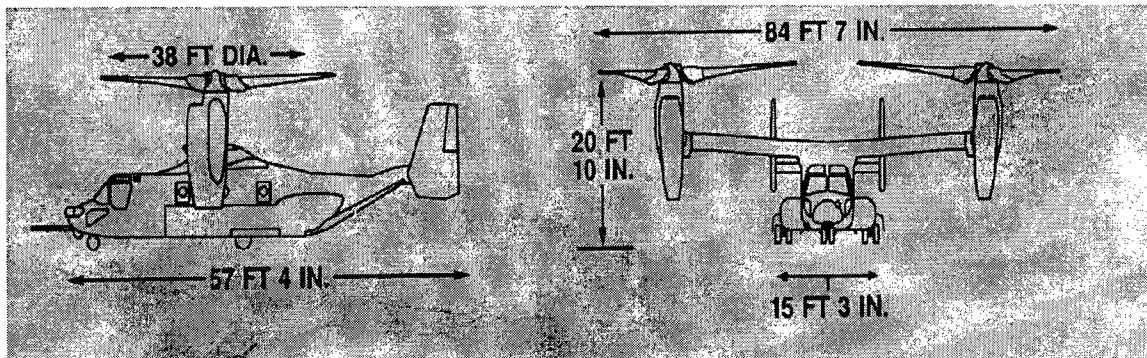
Figure 7. Folded dimensions.
