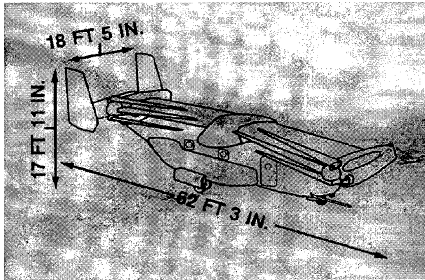
Figure 6. Side and front dimensions.
