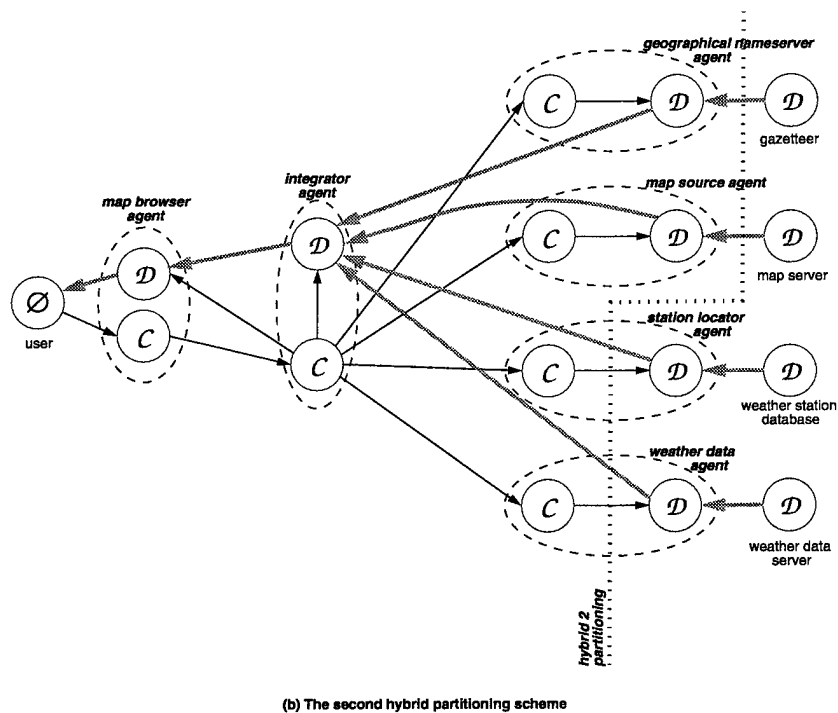
Figure 4.8: Partitions of the weather browser application that were studied in the experiment. Note that the data path labels from Figure 4.3 have been omitted here for clarity.
