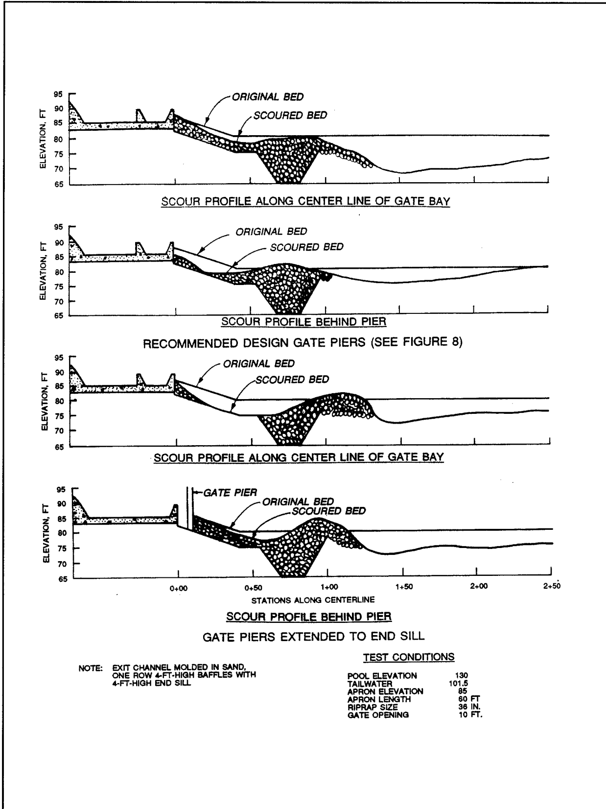
Figure 9. Comparison of scour patterns for Arkansas River stilling basins model tested
