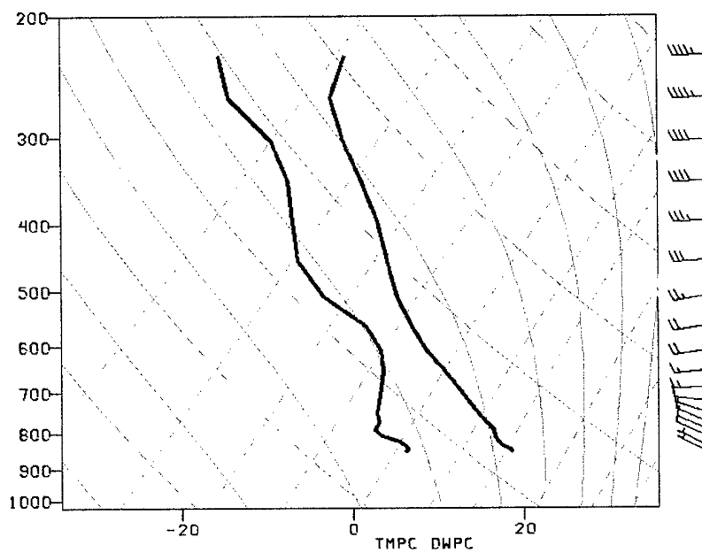
FIGURE 16: 0000 UTC 17 Oct 1996, Skew- T s at GJT. (a) Observed. (b) Forecasted.
