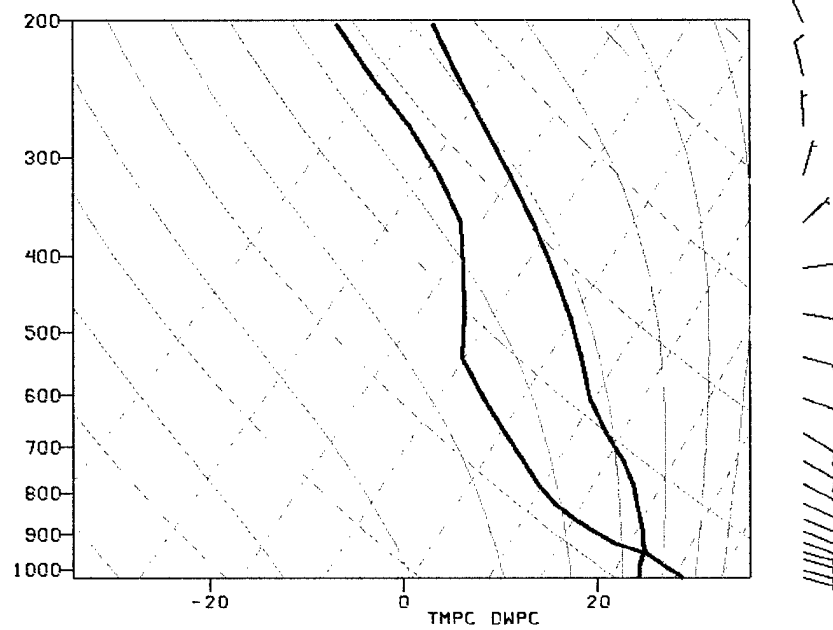
FIGURE 8: 1200 UTC 7 August 1996, Skew-Ts at EYW. (a) Observed. (b) Forecasted.
