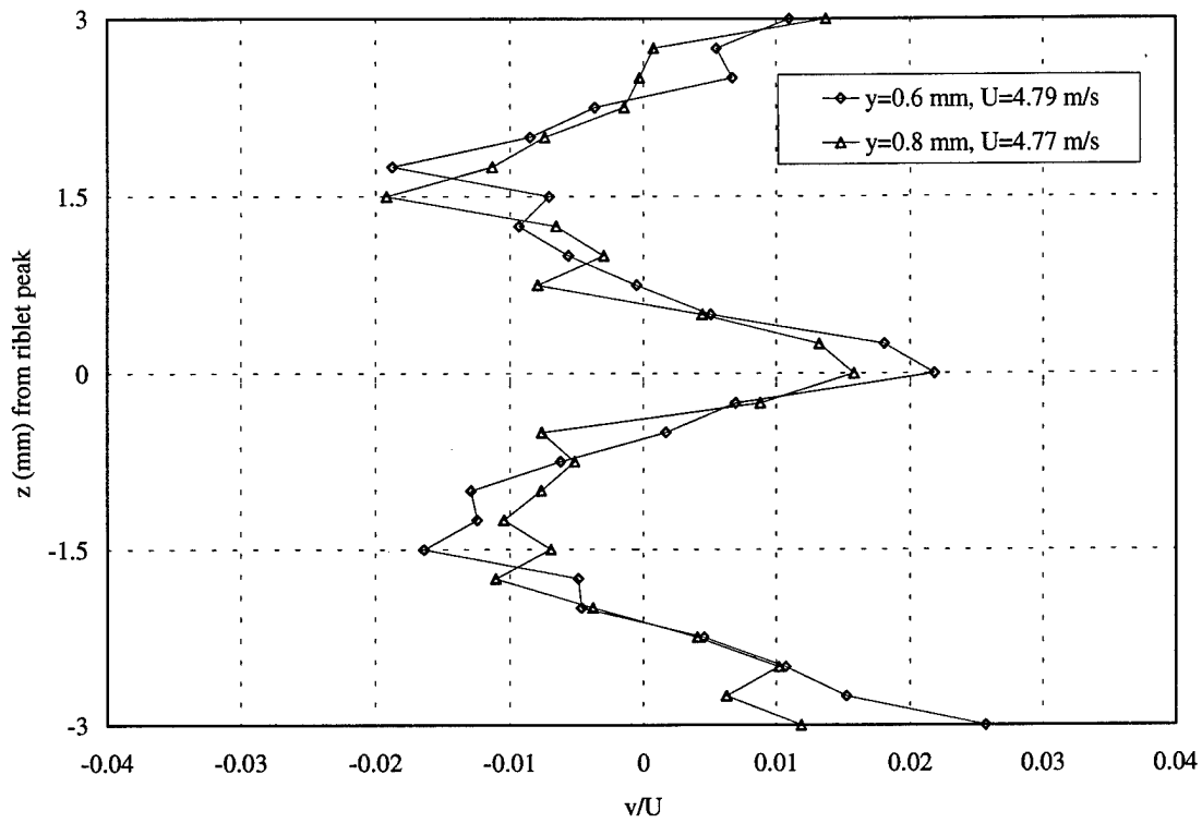
Figure 55. v profile, spanwise direction, riblet, APG, 400 mm
