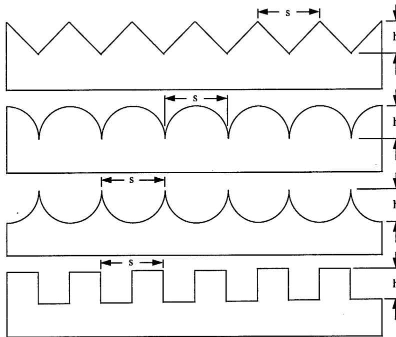
Figure 1. Common Riblet Shapes.
