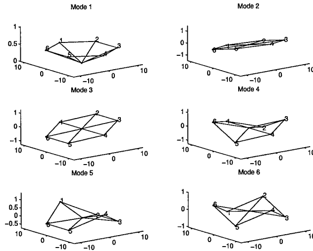
Figure 2.5 Circular Six Pendulum System Modes
