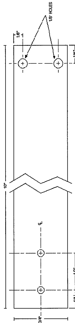
Figure 3.9 Cantilever Beam
