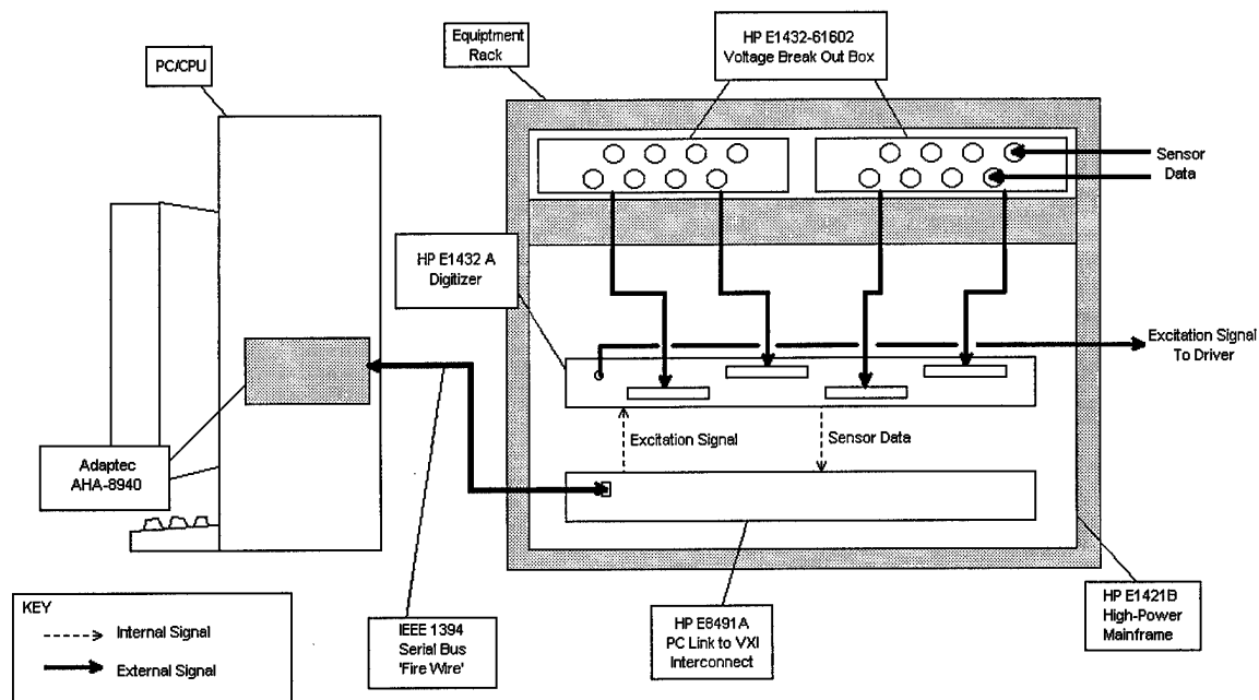
Figure 3.2 Data Acquisition Up Block Diagram
