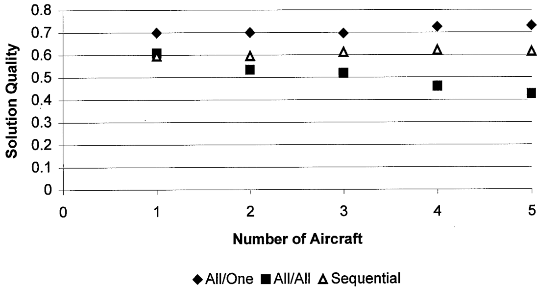
Figure 12. Solution Quality
