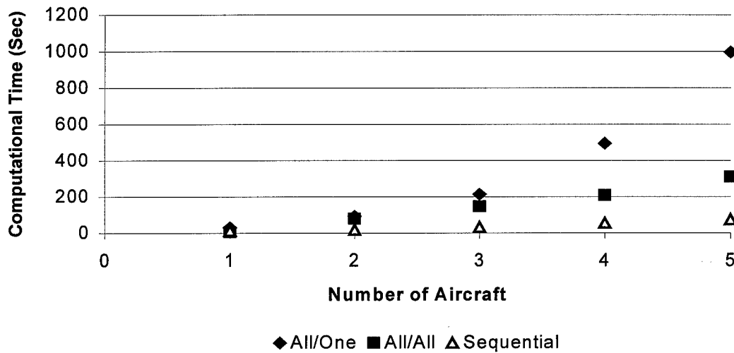
Figure 13. Computational Time
