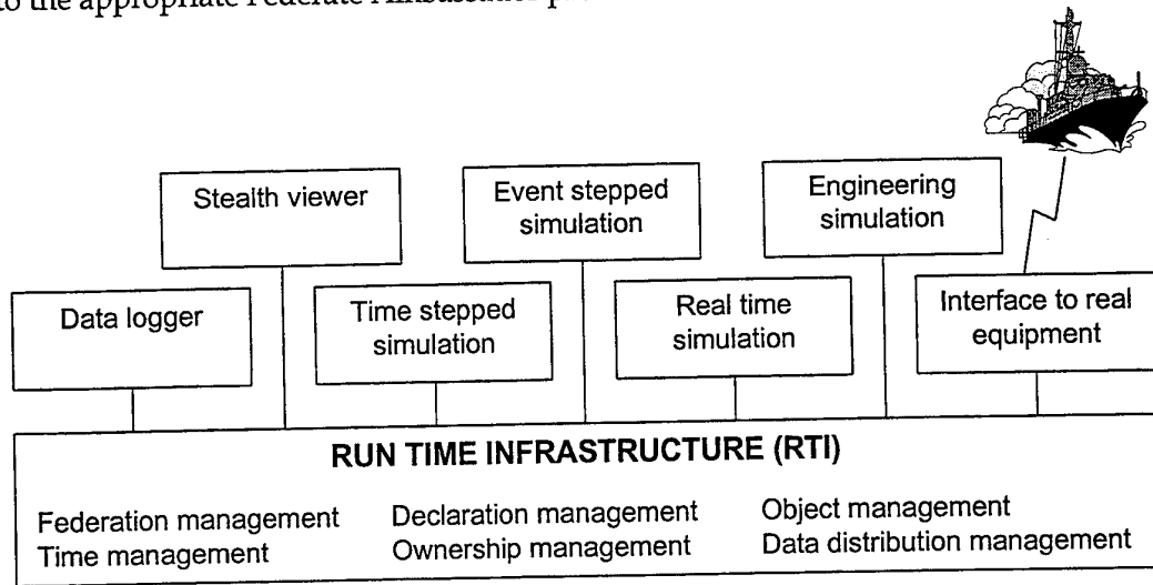
Figure 3: A functional view of the HLA. Many different types of federates may operate together over a network. The RTI provides the services that facilitate transfer of data amongst federates and the co-ordination of their time advances.
