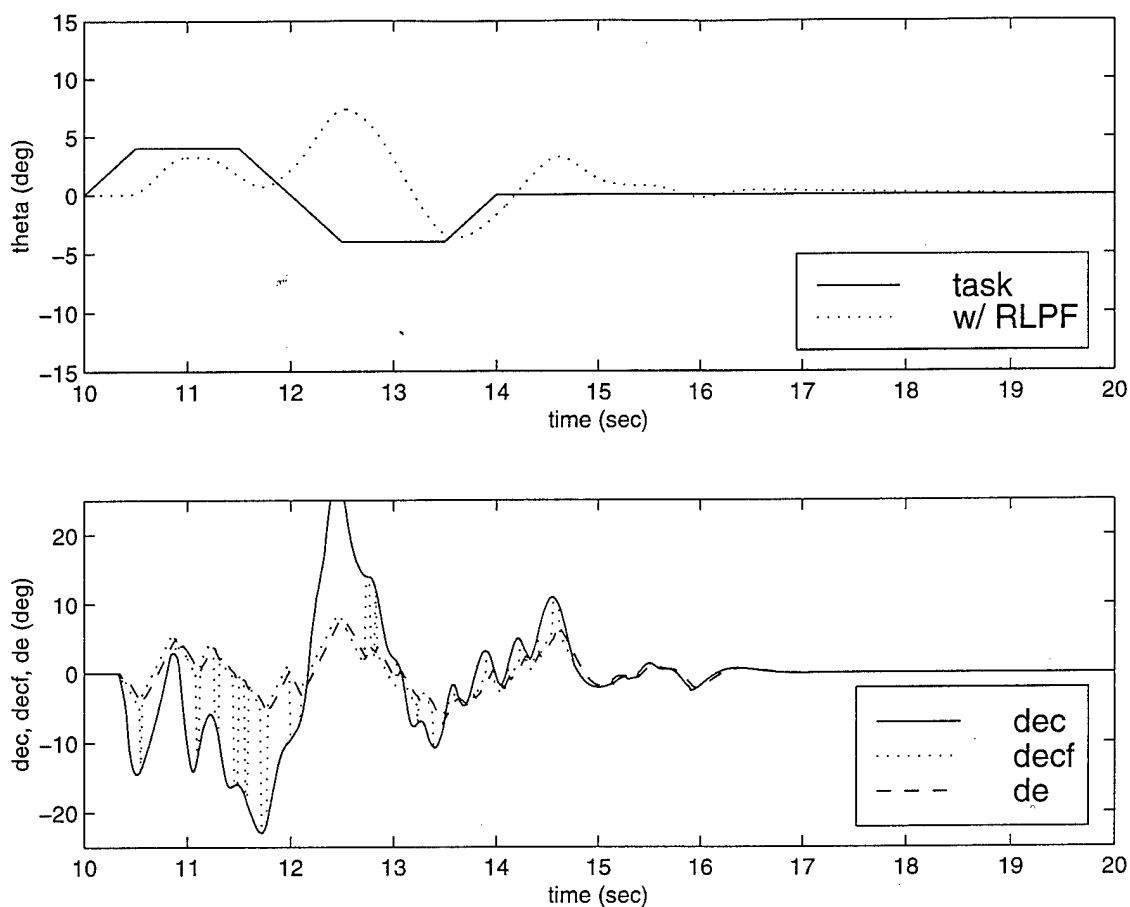
Figure 3-12. 30 deg/sec Actuator Rate Limit (LAMARS)
