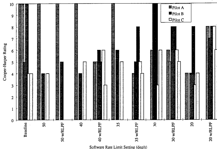
Figure 6-21. HAFA 1 RLPF Effects on Phase 3 Cooper-Harper Ratings (RLPF = 100 deg/sec 2 )
