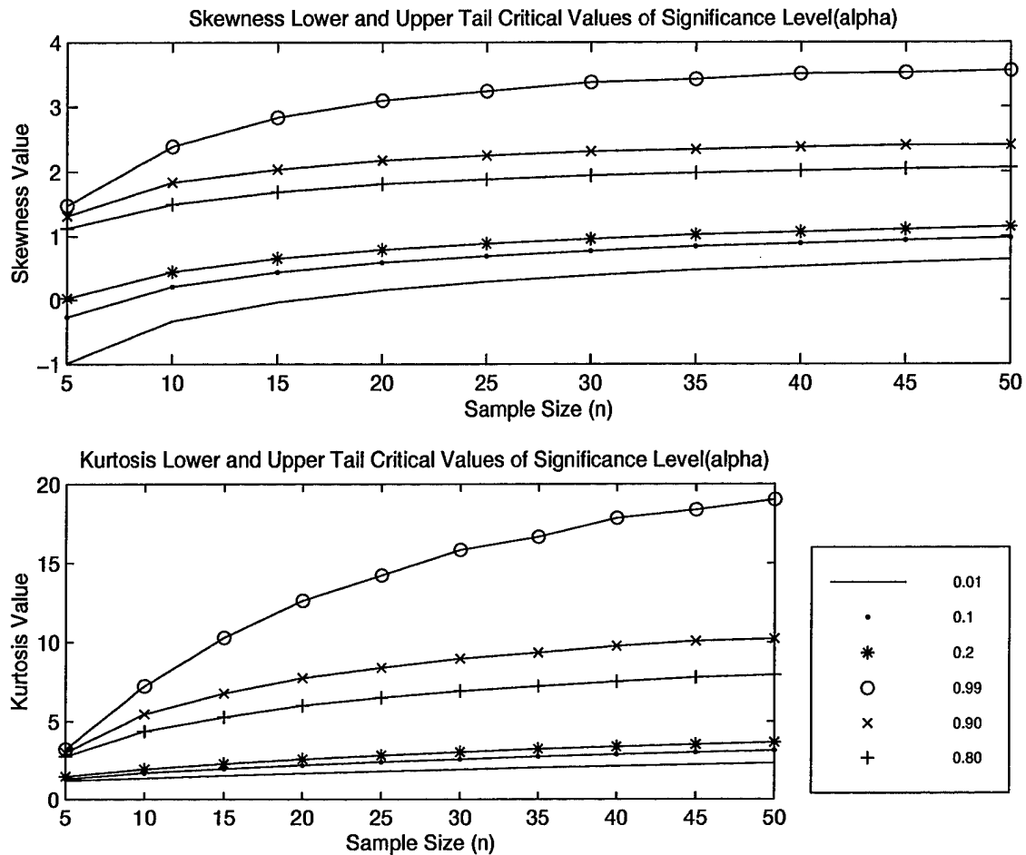
Figure 4.2 Critical Values for Skewness and Kurtosis, \beta=1
