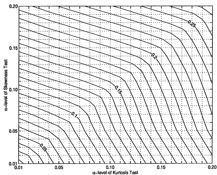
Figure D.1 Sample Size = 5
