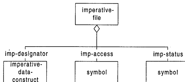
Figure 9. Imperative-File
