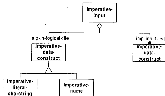
Figure 7. Imperative-Input
