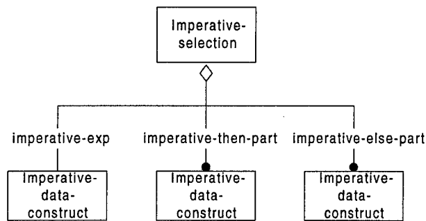
Figure 10. Imperative-Selection
