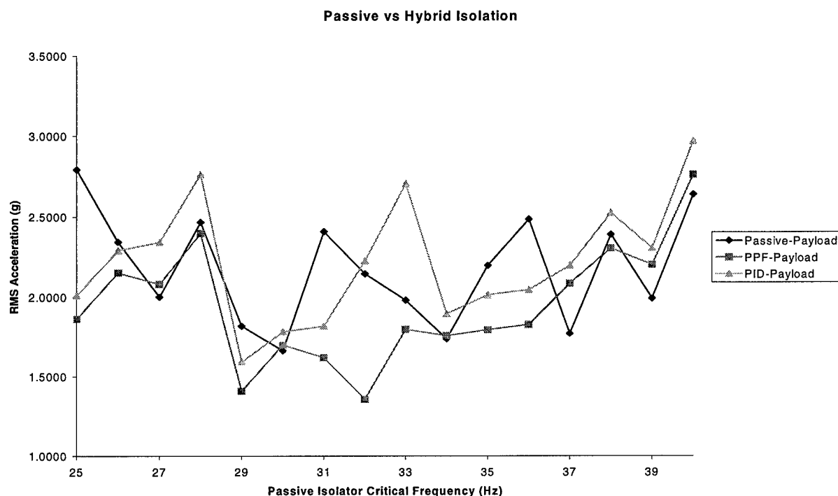
Figure 27 .Passive vs Hybrid Isolation at the Payload Component
