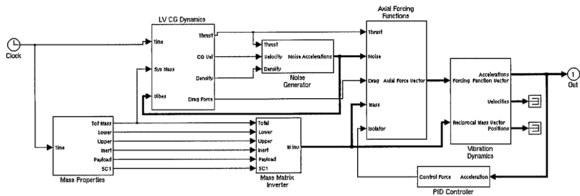
Figure 37 Top level of five DoF PID model
