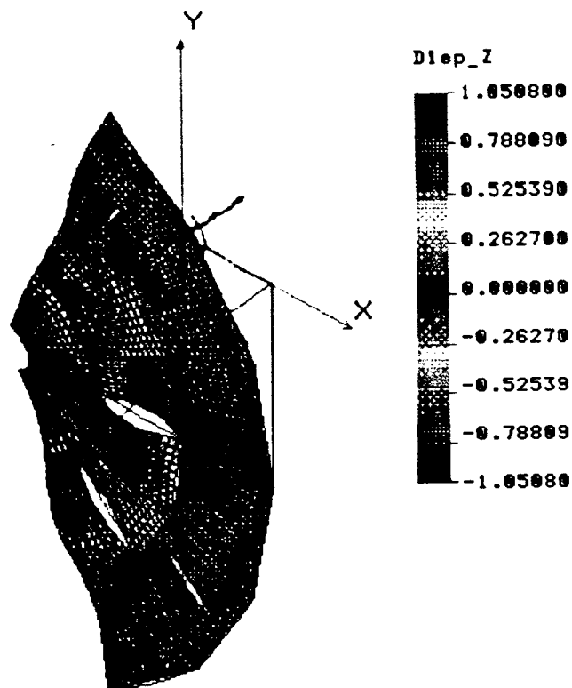
Figure 18: Twelve Meter Primary Mirror, Mode 87 _Mode=87 108.174 Hz
