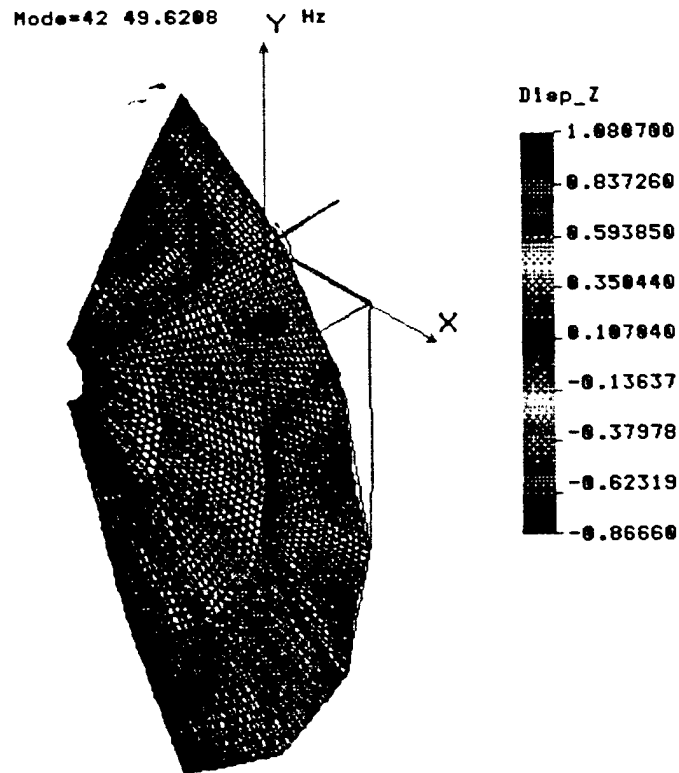
Figure 11: Twelve-Meter Primary Mirror, Mode 42
