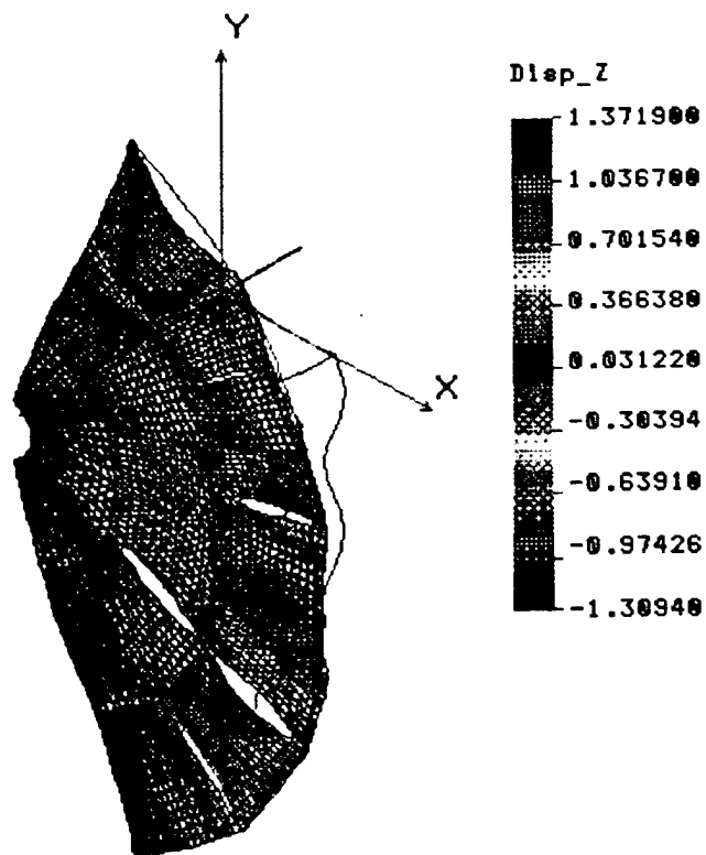
Figure 17: Twelve Meter Primary Mirror, Mode 85 _Mode=85 102.254 Hz
