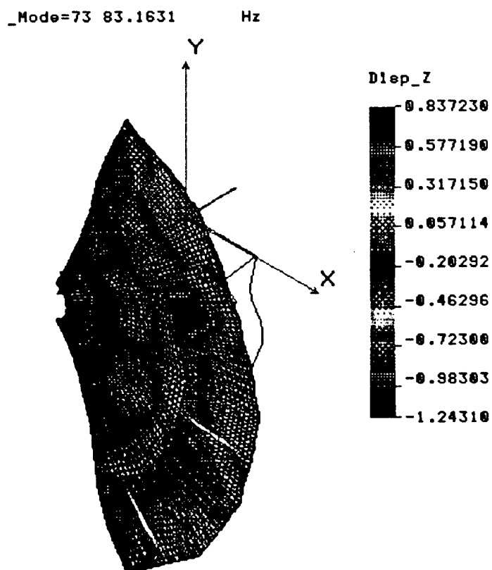
Figure 15: Twelve Meter Primary Mirror, Mode 73
