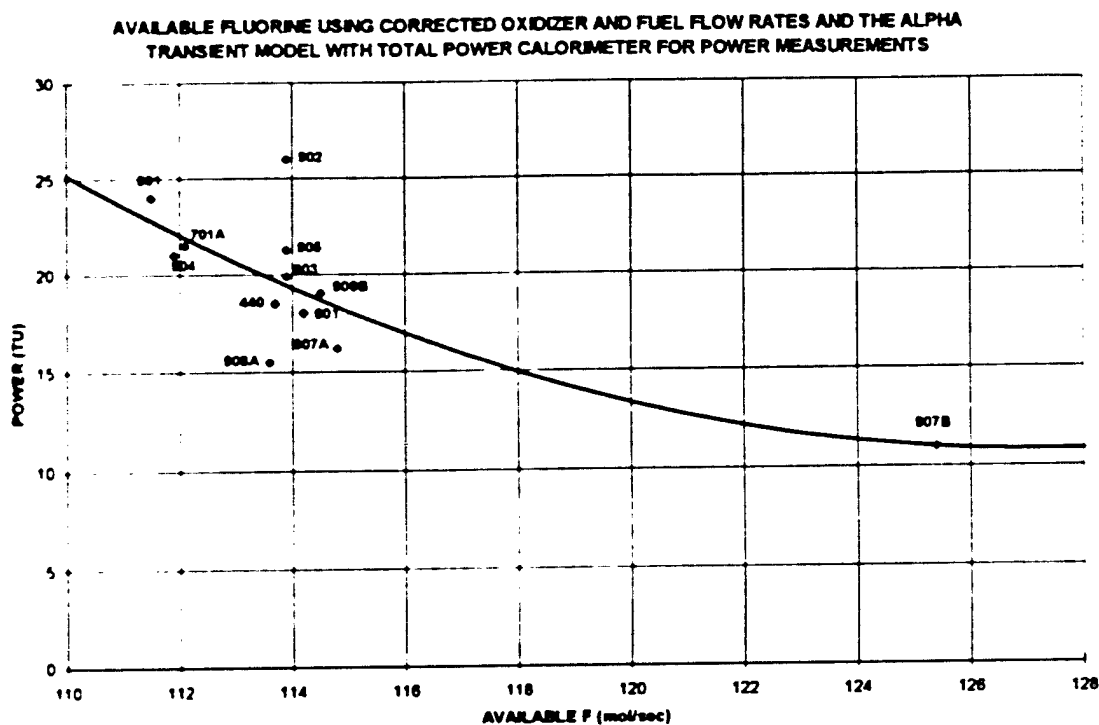
Figure 3.1-2: Available Fluorine
