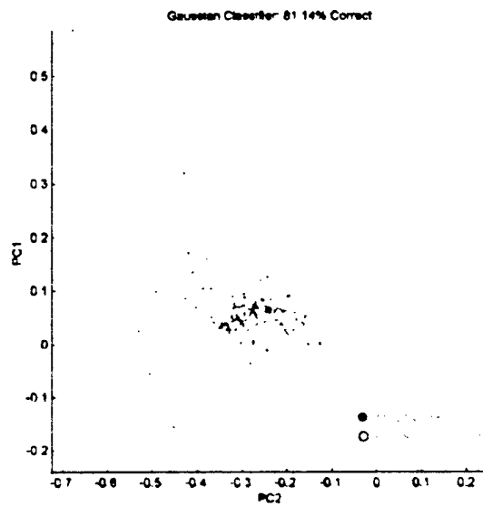
Figure 7 Gaussian classifier
