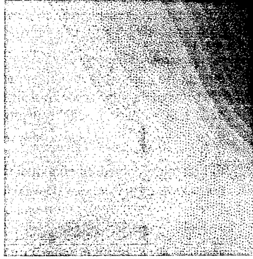
1000 km .37m/pix
