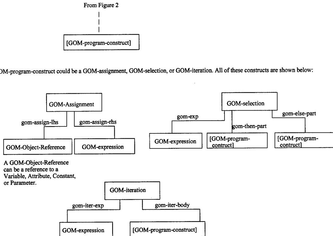
Figure 20 Design Program Constructs
