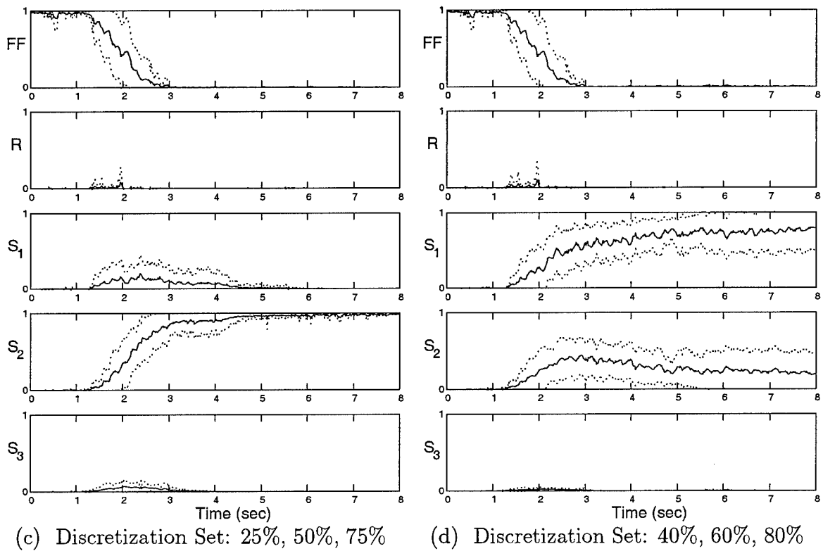
Figure 80. Probability Plot: Rudder Failure, \epsilon = 70\%
