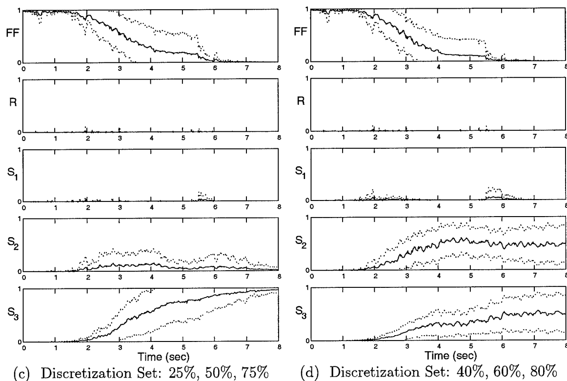
Figure 82. Probability Plot: Rudder Failure, \epsilon = 90\%
