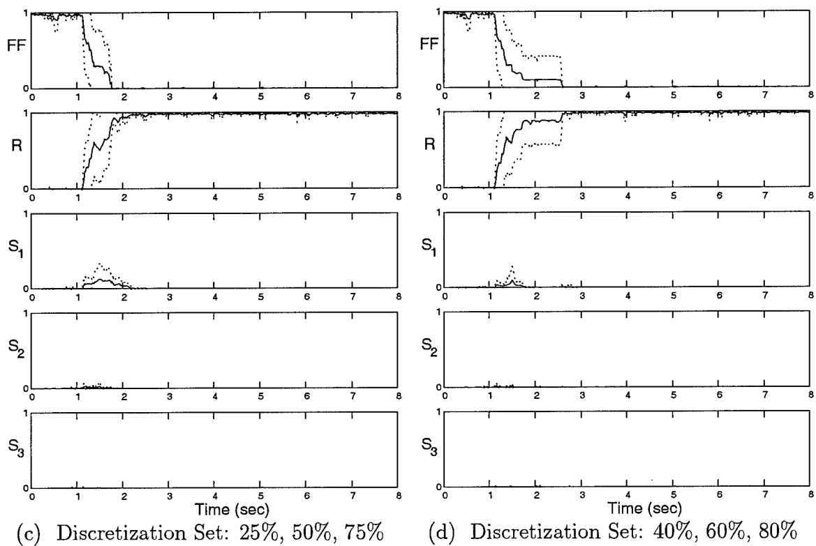
Figure 73. Probability Plot: Rudder Failure, \epsilon = 0\%
