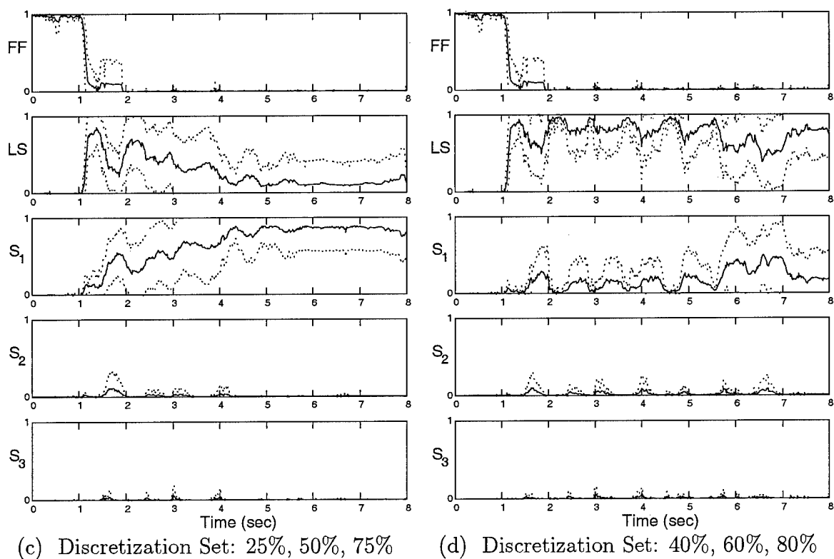
Figure 9. Probability Plot: Left Stabilator Failure, \epsilon = 10\%
