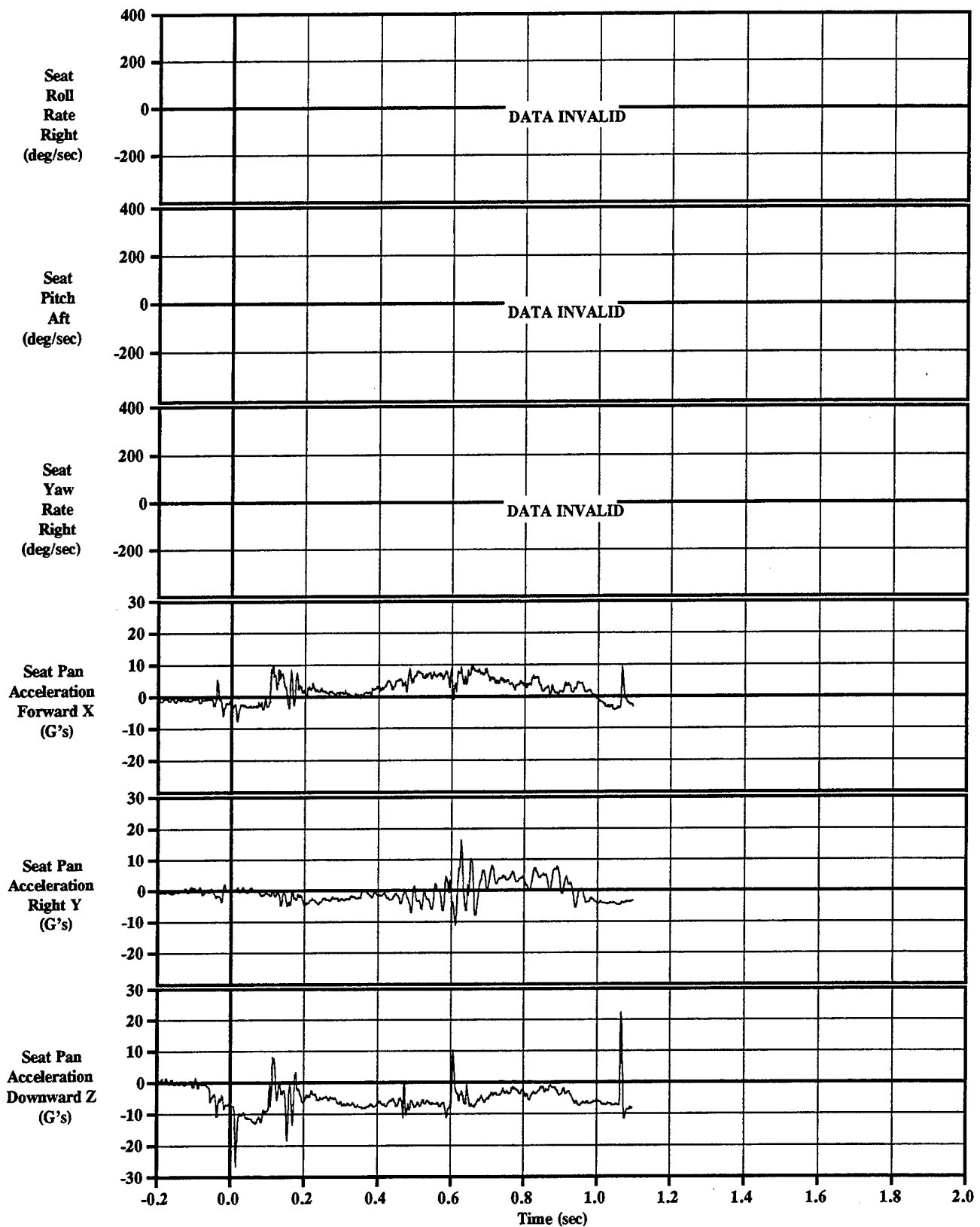
Figure C-4-9 Seat Angular Rates & Seat Pan Acceleration (80 Hz filter) Sled Test=4, KEAS=325, 5th%, Roll=60
