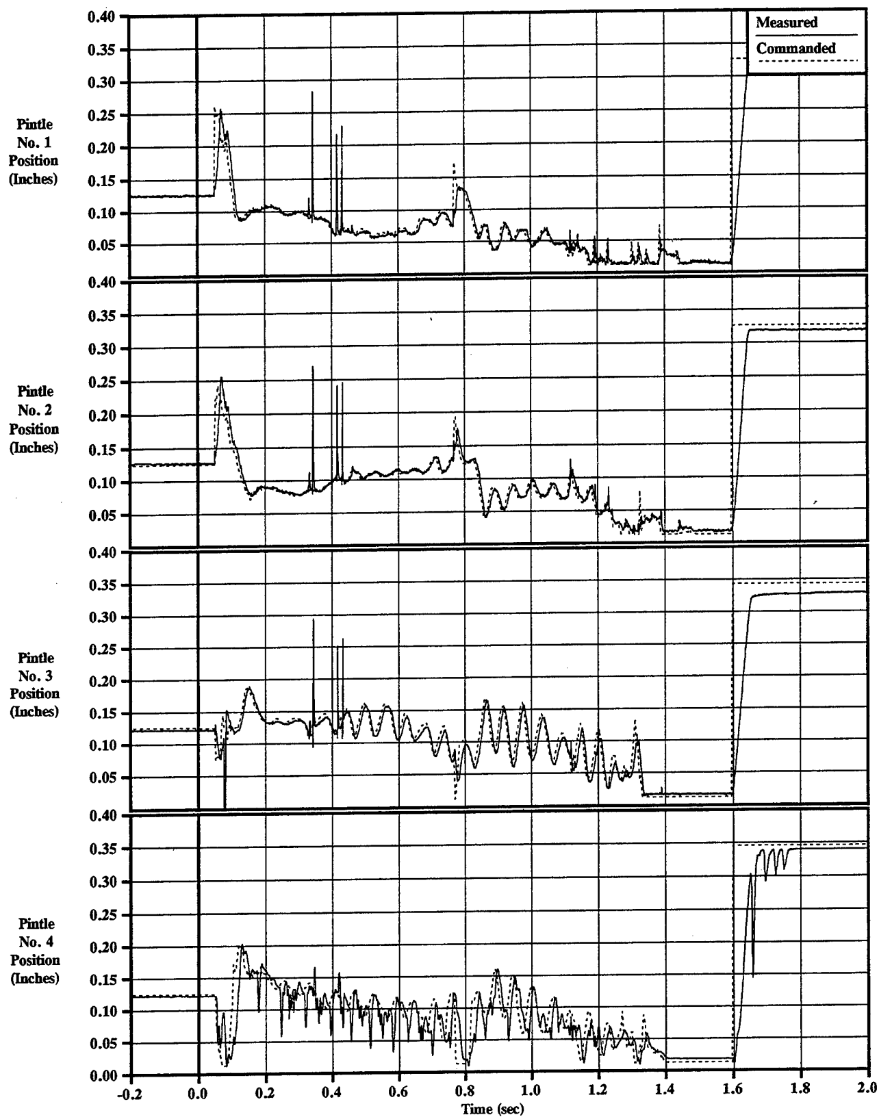
Figure C-10-12 Pintle Positions & Commands Sled Test=10, KEAS=700, 5th%
