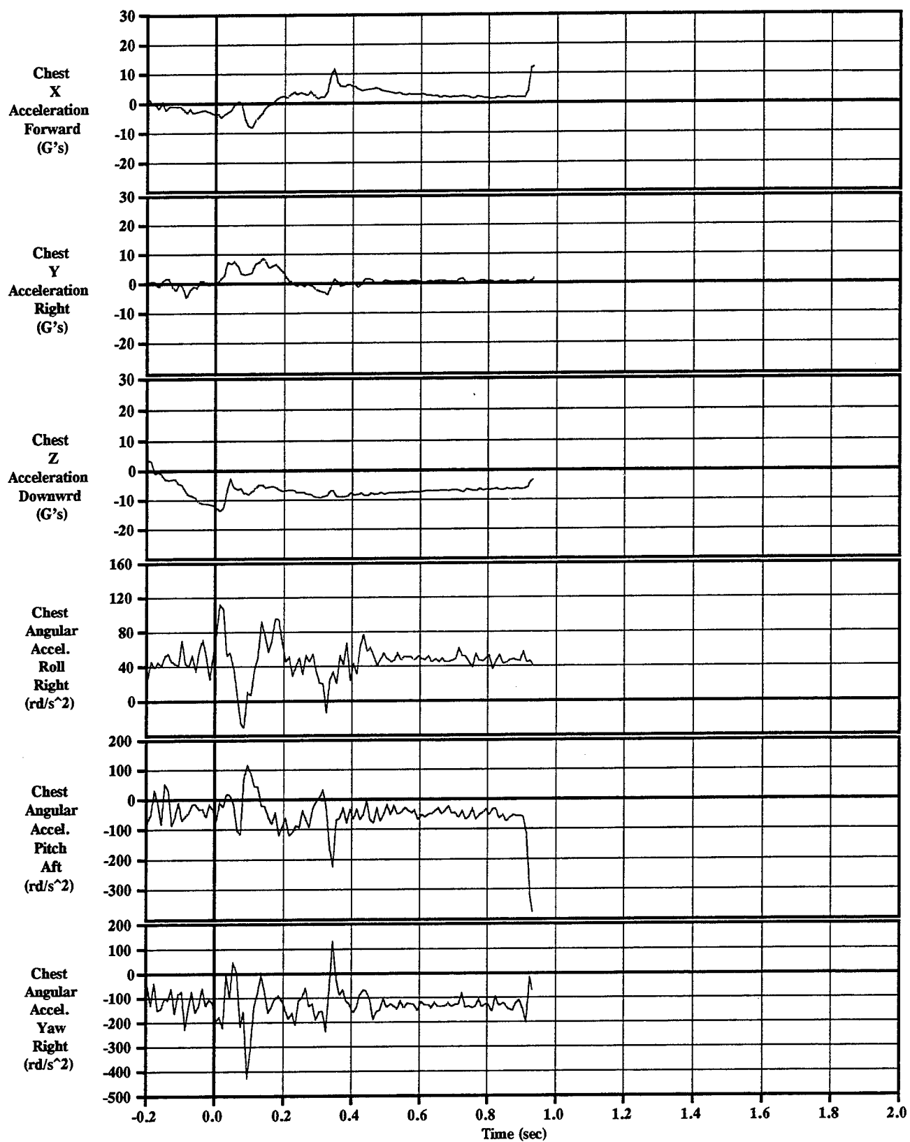
Figure C-8-8 ADAM Chest Linear & Angular Accelerations Sled Test=8, KEAS=438, 5th%, Yaw=20
