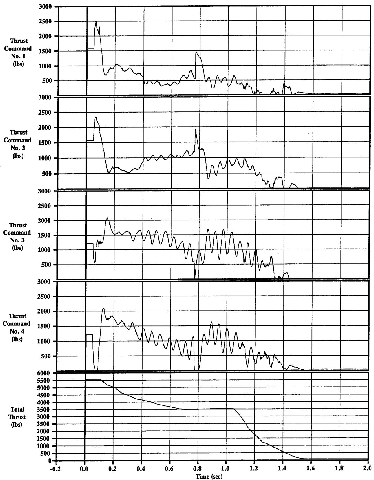
Figure C-10-4 Thrust Commands Sled Test=10, KEAS=700, 5th%
