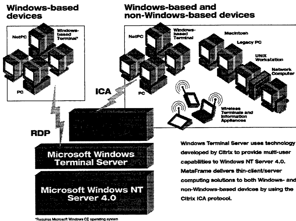
Figure 13. Thin-Client/Server Architecture [20]
