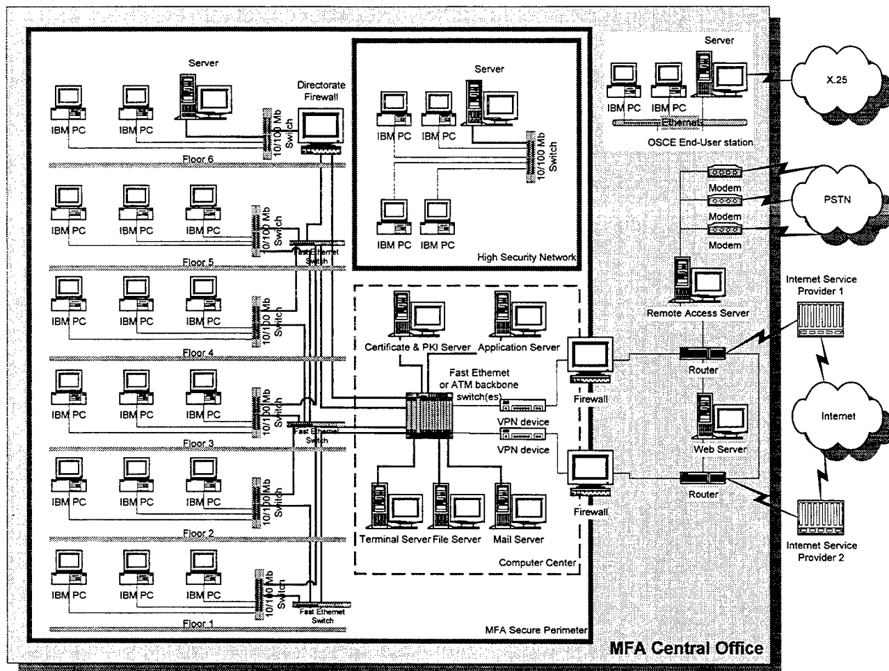
Figure 11. MFA of Ukraine Central Office network diagram.
