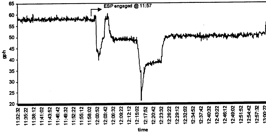
Figure 8. Max Machine Fuel Monitor – Handle Position 7 (August 26)
