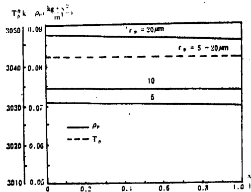
Figure 7. Distribution of Particle Parameters in Two-Phase Flow
