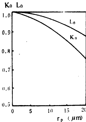
Figure 9. Effect of Particle Size on K_0 , L_0
