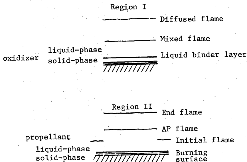
Figure 1. One-Dimensional Steady-State Model
