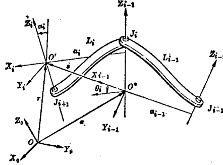
Figure 9. Relation Between the (0, 0^*) and (0, 0') Frames
