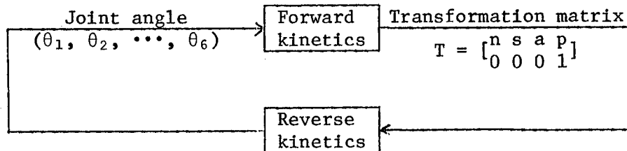
Figure 5. Forward and Reverse Problems in Robotic Kinetics
