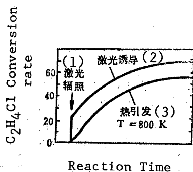
Fig. 1 Comparison of laser induced reaction and thermal reaction for producing chloroethylene
