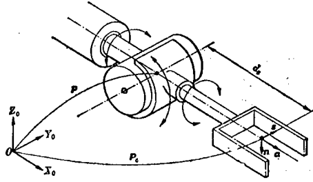
Figure 8. Coordinates To Solve Reverse Problems
