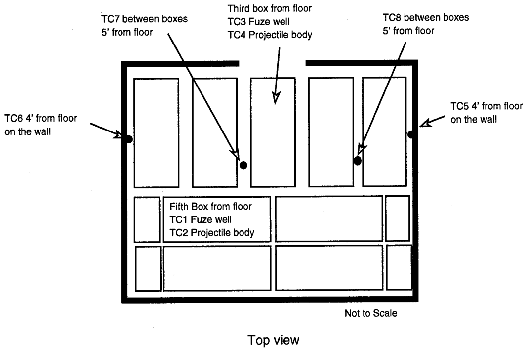
Figure C-2. Thermocouple Locations
