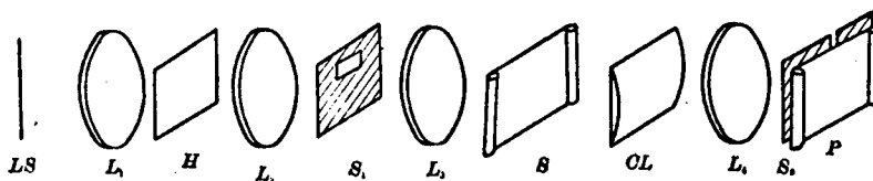
Fig. 10 White Light Optical Convolution System for Deblurring
