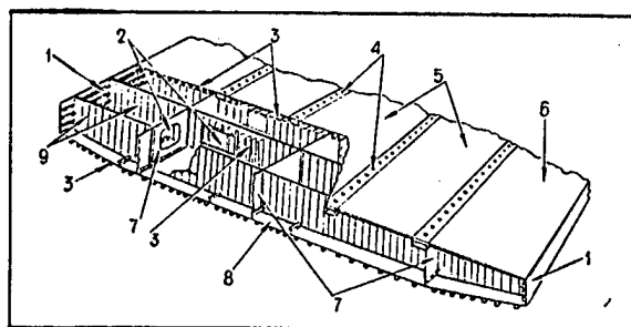
Figure 2. Hull Design of an LCAC-Class Landing Craft
