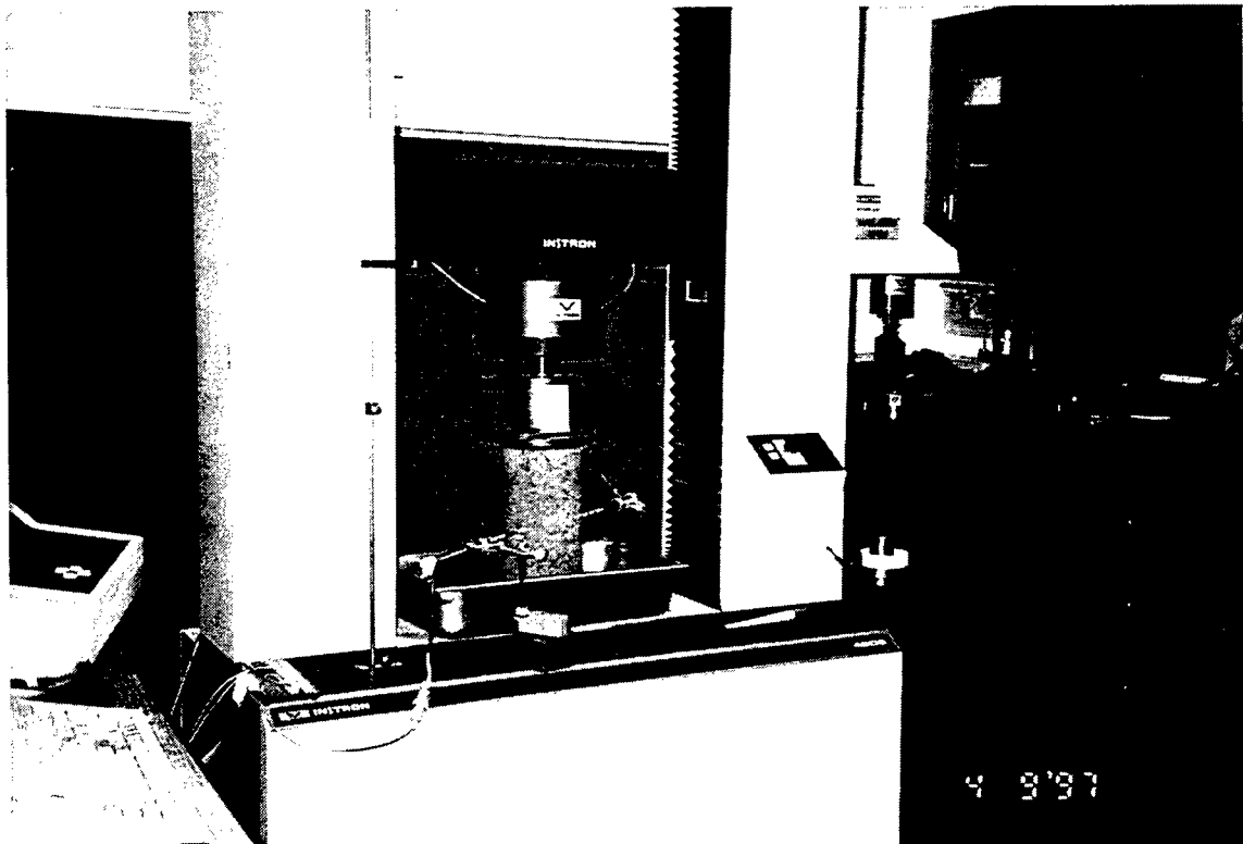
Photo 4. Laboratory unconfined compression test setup
