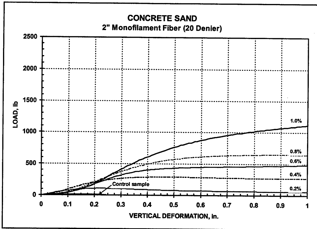
Figure 7. Performance of 2-in. monofilament (20 denier) fibers in concrete sand
