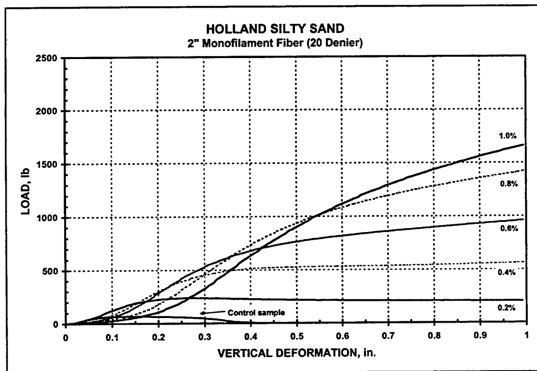
Figure 10. Performance of 2-in. monofilament (20 denier) fibers in Holland LZ sand
